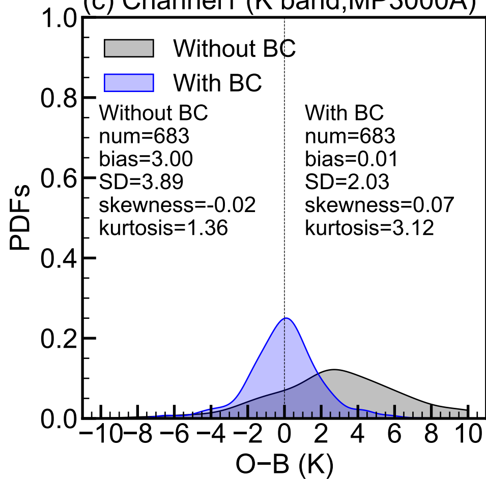
(c) Channel1 (K band,MP3000A)
