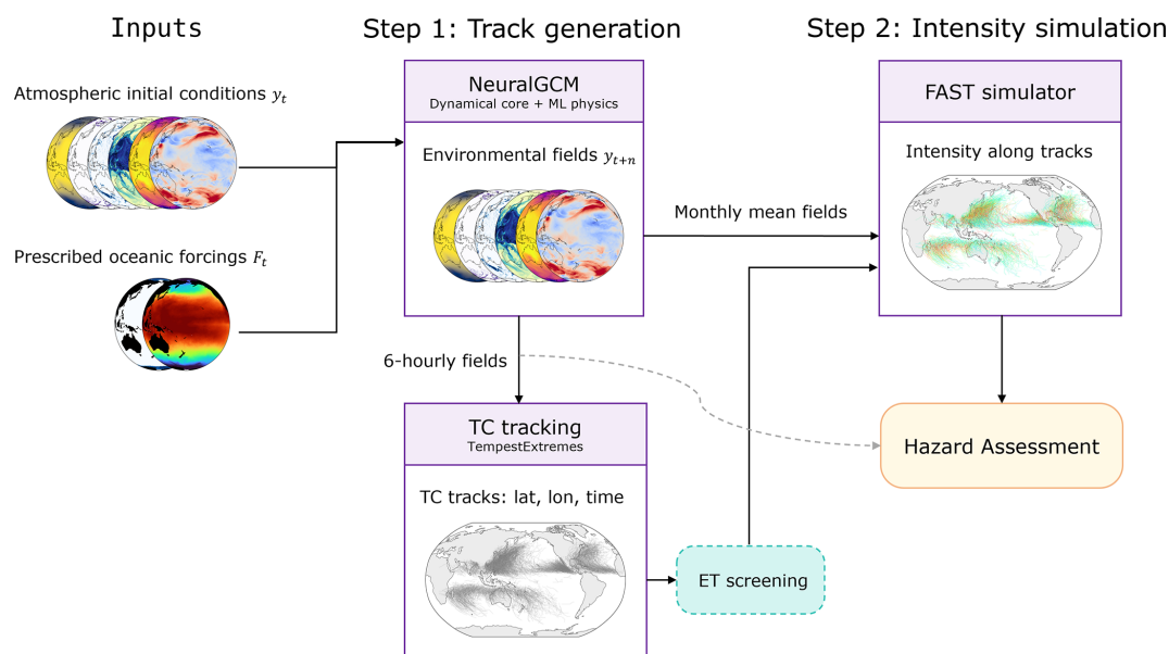
Figure 1. Workflow of the two-step SPIN modelling framework. In Step 1, atmospheric initial conditions y_t and prescribed oceanic forcings F_t are provided to NeuralGCM to generate environmental fields. The simulated 6-hourly environmental fields are used to detect and track TCs with TempestExtremes. Extratropical transition (ET) screening is then applied to the simulated tracks. In Step 2, the generated tracks and simulated monthly-mean environmental fields are passed to the FAST intensity simulator to estimate TC intensity along each track. The synthetic tracks and their ambient environments can then be used for hazard assessment.
