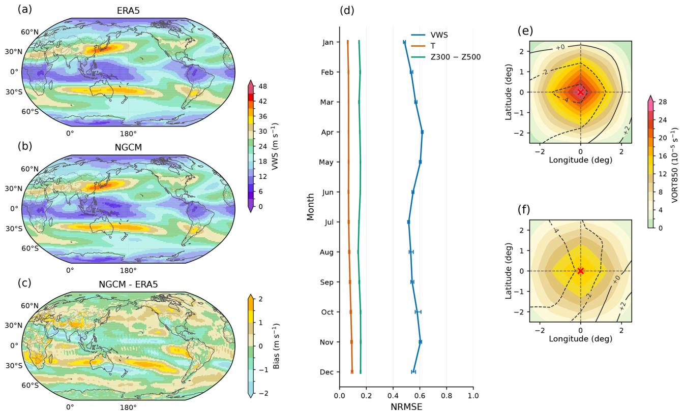
Figure 2. Evaluation of simulated atmospheric environmental fields. Panels show the 1980–2022 mean 200–850 hPa vertical wind shear (VWS; \text{m s}^{-1} ) from (a) ERA5, (b) the NeuralGCM ensemble mean, and (c) their difference. Panel (d) shows monthly normalized root-mean-square errors (NRMSEs) between NeuralGCM and ERA5 for VWS, the meridional temperature profile ( T ; K), and the 300–500 hPa geopotential height difference ( Z300 - Z500 ; \text{m}^2 \text{s}^{-2} ), averaged over 1980–2022, with error bars indicating the 10th–90th percentile range across ensemble members. Panels (e) and (f) show storm-centred composites of the surrounding environment for FAST-simulated extreme TCs in the North Atlantic basin during 1980–2022. Composites are shown for the (e) top 10 % and (f) lowest 10 % of storms ranked by lifetime maximum intensity, evaluated at the time of lifetime maximum intensity. Shading shows 850 hPa relative vorticity ( \text{s}^{-1} ), and contours show surface pressure anomalies (hPa) relative to the mean pressure within a storm-centred 500–800 km annulus.
