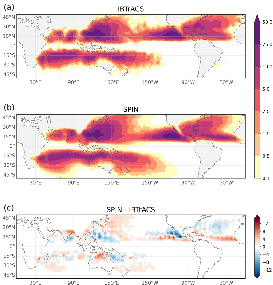
Figure 8. Annual 6-hourly TCs track density on a 1^\circ \times 1^\circ grid with Gaussian smoothing for 1980–2022. (a) IBTrACS, (b) ensemble-mean simulations from SPIN, and (c) their difference (b–a). Only storms reaching maximum wind \geq 18 \text{ m s}^{-1} are included, with tracks evaluated from the first occurrence of that threshold.
