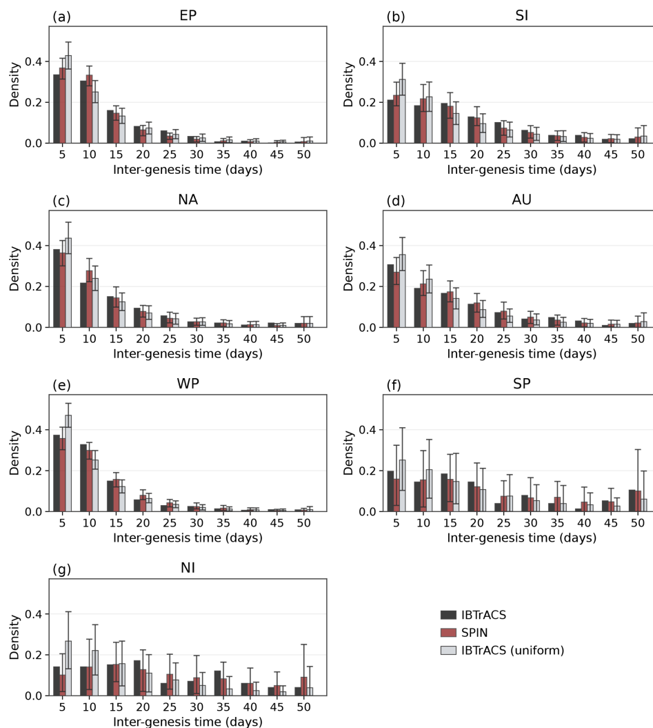
Figure 11. Histogram of TC inter-gensis intervals from 1980–2022. Calculations are limited to the TC season in each year, defined as April–November for Northern Hemisphere basins (EP, NA, WP, NI; panels a , c , e , g ) and from November to the following April for Southern Hemisphere basins (SI, AU, SP; panels b , d , f ). Results from IBTrACS (black), IBTrACS with uniformly sampled dates (grey), the ensemble mean of SPIN simulations (red) are shown for comparison. Error bars denote the 10th–90th percentile range across ensemble members for SPIN and across 1000 Monte Carlo realizations for the uniform experiments.
