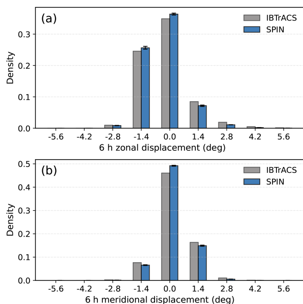
Figure 7. Comparison of 6 h TC displacement statistics between observations and the SPIN ensemble. (a) Zonal and (b) meridional displacements of TCs in IBTrACS (grey) and SPIN (ensemble mean, blue). Error bars indicate the 10 %–90 % ensemble spread for SPIN. Bins are defined at 1.4^{\circ} intervals.
