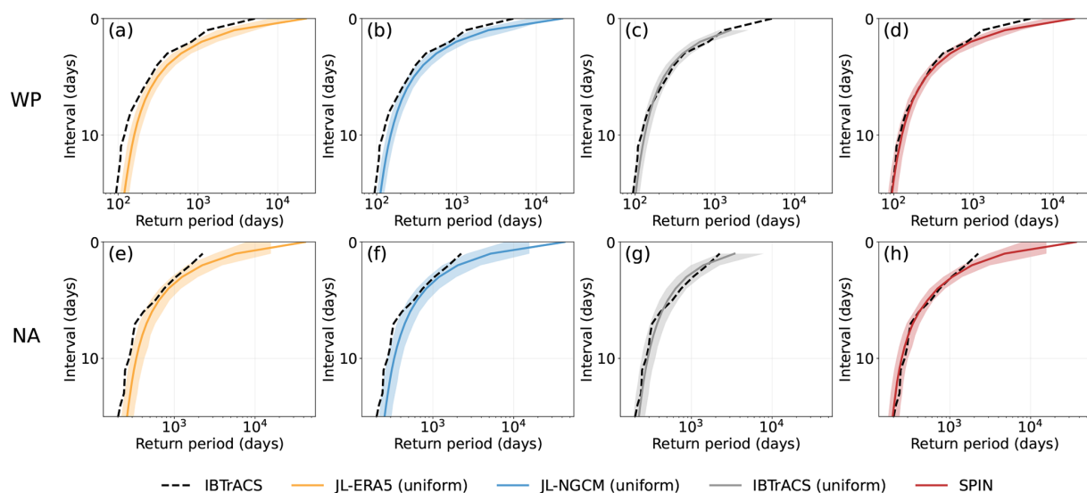
Figure 18. Return periods of inter-MTCE time. The y-axis shows the MTCE inter-genesis interval (0–15 d), and the x-axis shows the return period (days). Panels (a)–(d) correspond to the WP basin and panels (e)–(h) to the NA basin. Shown for comparison are results from IBTrACS (black), IBTrACS with uniformly sampled dates (grey), JL-ERA5 with uniformly sampled dates (yellow), and JL-NGCM (single ensemble member) with uniformly sampled dates (blue), and SPIN (red). The solid line in each panel indicates the return period computed from all Monte Carlo simulations (a, b, c, e, f, g) or all ensemble members (d, h). The shaded region represents the 10th–90th percentile range across individual ensemble members.
