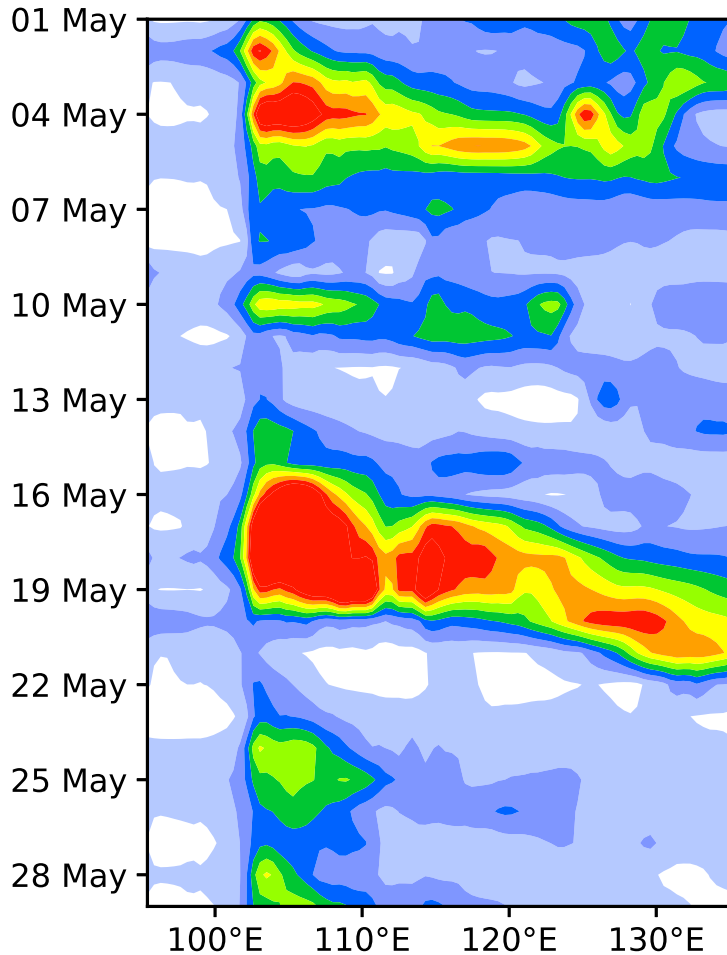
(b) CMA-CPSv4 Dust at 39°N (2011)
