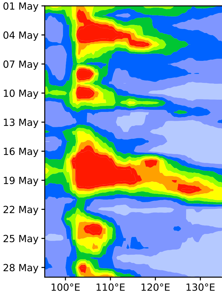
(a) MERRA-2 Dust at 39°N (2011)
