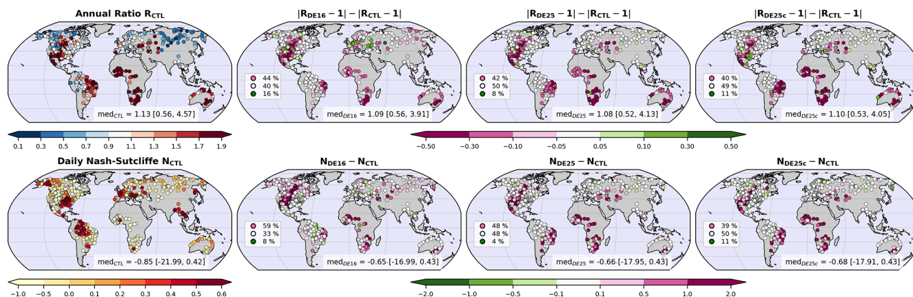
Figure 8. Comparison between observed and simulated daily river discharges over the 1979–2010 period at 698 gauging stations. Each dot represents a river gauging station. The first column shows the annual discharge ratio, R , and the daily Nash–Sutcliffe efficiency, N , for the CTL experiment. The following columns show the differences in these metrics relative to CTL for DE16, DE25, and DE25c, respectively, using |R - 1| for the discharge ratio panels, which measures the distance to the unbiased value. For each panel, the inset reports the median and the [10, 90] % interval of the corresponding metric across all stations. In the difference panels, stations are also classified as improved (pink), neutral (white), or degraded (green) based on their change relative to CTL, and expressed in % of all stations. For |R - 1| , a station is improved when \Delta(|R - 1|) \leq -0.05 , and degraded when \Delta(|R - 1|) \geq 0.05 . For N , a station is improved when \Delta N \geq 0.1 , and degraded when \Delta N \leq -0.1 .
