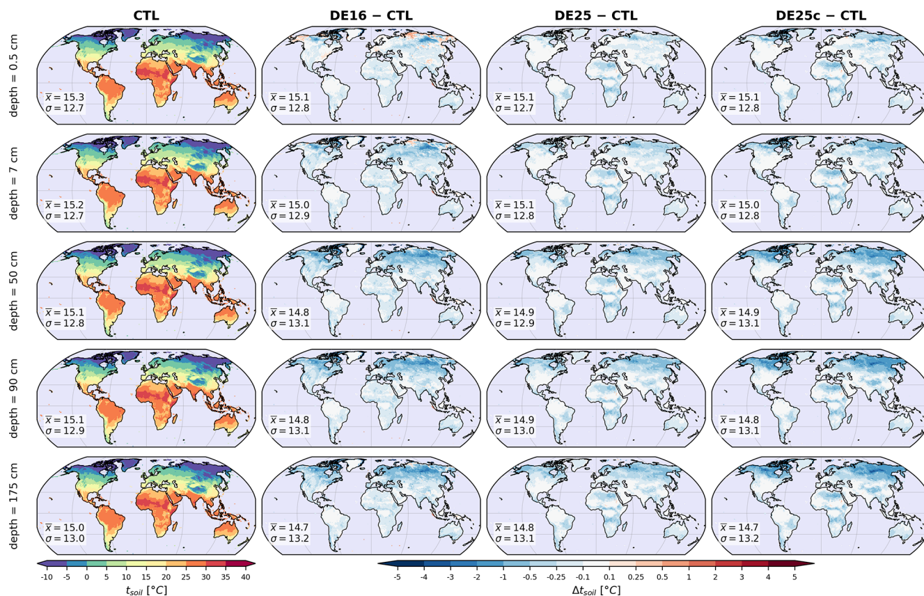
Figure 11. As in Fig. 5, but for the simulated soil temperature ( ^{\circ}\text{C} ).
