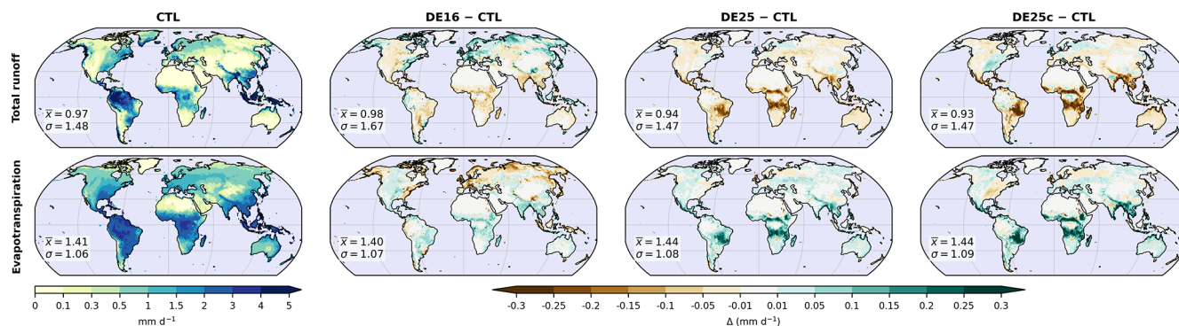
Figure 10. Comparison of simulated continental runoff and evapotranspiration climatologies expressed in \text{mm d}^{-1} over the 1979–2010 period. The first column shows the annual mean total runoff (top row) and evapotranspiration (bottom row) for the CTL experiment. The following columns show the differences relative to CTL for DE16, DE25, and DE25c, respectively. For each map, the inset reports the spatial mean \bar{x} and standard deviation \sigma over land points for the corresponding experiment (not for the differences).
