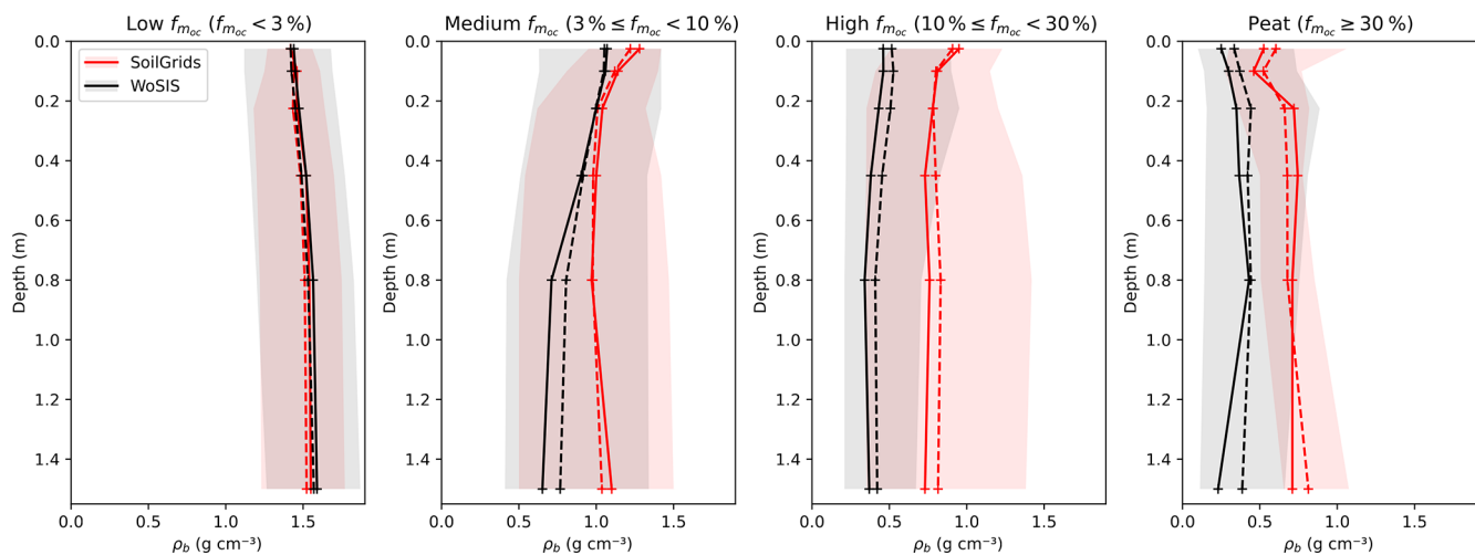
Figure 14. Comparison of SoilGrids and WoSIS vertical profiles of soil bulk density ( \rho_b ) as a function of depth for four classes of organic matter content: low SOC ( f_{\text{moc}} < 3\% ), medium SOC ( 3\% \leq f_{\text{moc}} < 10\% ), high SOC ( 10\% \leq f_{\text{moc}} < 30\% ), and peat ( f_{\text{moc}} \geq 30\% ). WoSIS (World Soil Information Service) is a global database of in situ soil profile observations maintained by International Soil Reference and Information Centre (ISRIC), compiling measured soil properties from multiple sources and regions worldwide, and constitutes the main observational reference for global soil mapping. Profiles are shown for SoilGrids in red and for WoSIS in black. As in Fig. 4, solid lines indicate median profiles, dashed lines indicate mean profiles, and shaded envelopes represent the 10th to 90th percentiles within each SOC class.
