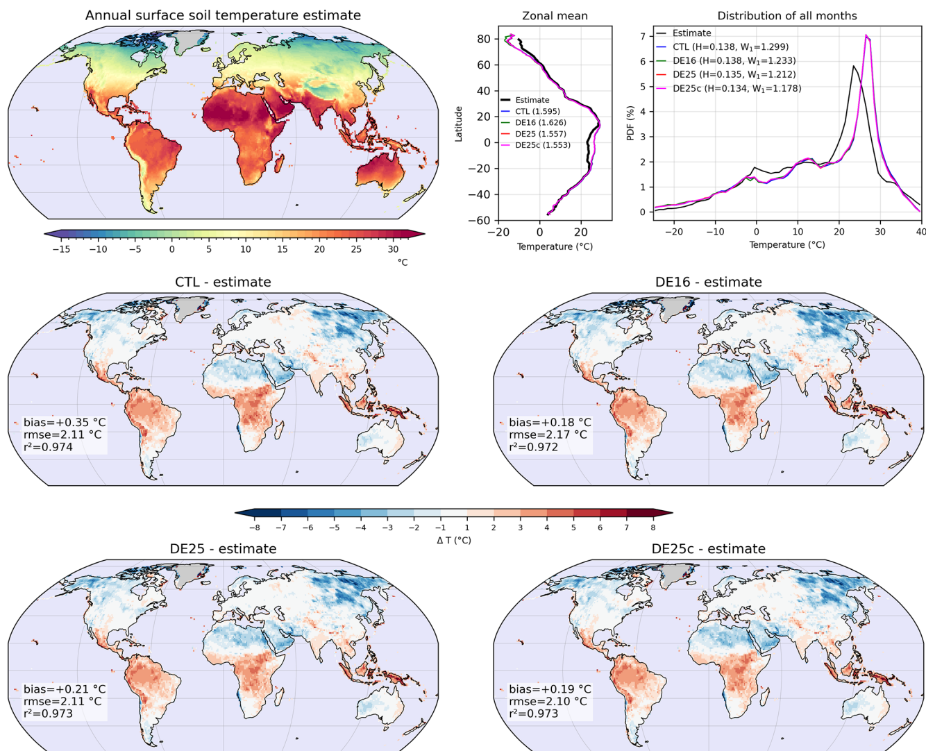
Figure 12. As in Fig. 9, but for the comparison between simulated and estimated near-surface soil temperature (°C) at 0–5 cm depth over the 1979–2010 period. The estimate corresponds to the climatological product of Lembrechts et al. (2022).
