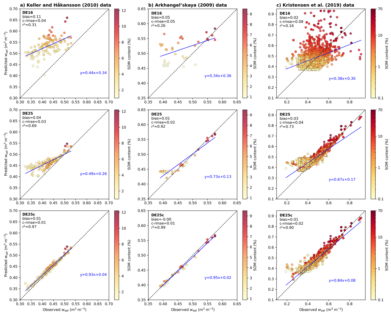
Figure 2. Comparison of observed and predicted soil porosity by the three schemes DE16, DE25 and DE25c across the three in situ datasets already used in Decharme (2025): (a) Keller and Håkansson (2010), (b) Arkhangel'skaya (2009), and (c) Kristensen et al. (2019). The 1 : 1 line is shown in black, and the blue line represents the linear regression between predicted and observed values where its slope and intercept provide an additional measure of agreement. Finally, skill scores (bias, c-rmse and r^2 ) are given for each panel.
