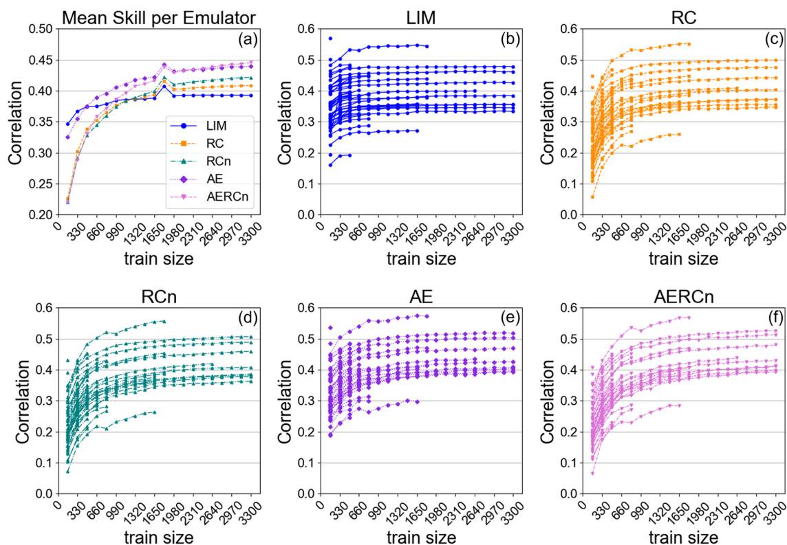
Figure 6. Sensitivity of forecast skill to training data length. Panel (a) shows the spatially averaged correlation as a function of training size (years), with one curve per emulator averaged across CMIP6 models. Panels (b)–(f) display model-specific results for LIM, RC, RCn, AE, and AERCn, with one curve per CMIP6 model.
