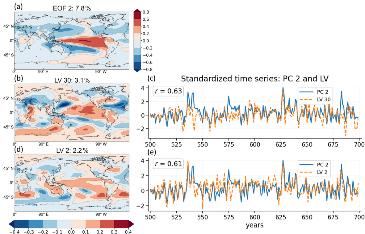
Figure A5. Variance structures associated with EOF 2 and AE latent vectors using a 30-dimensional latent space. Panel (a) shows the local variance explained by EOF 2 . The spatial patterns are dimensionless, as the EOF analysis is performed on the normalized covariance matrix. Panels (b) and (d) display variance explained by AE latent vectors selected based on correlation \geq 0.6 with EOF 2 . Panels (c) and (e) show the corresponding standardized time series over the first 200 years. Correlation coefficients are indicated.
