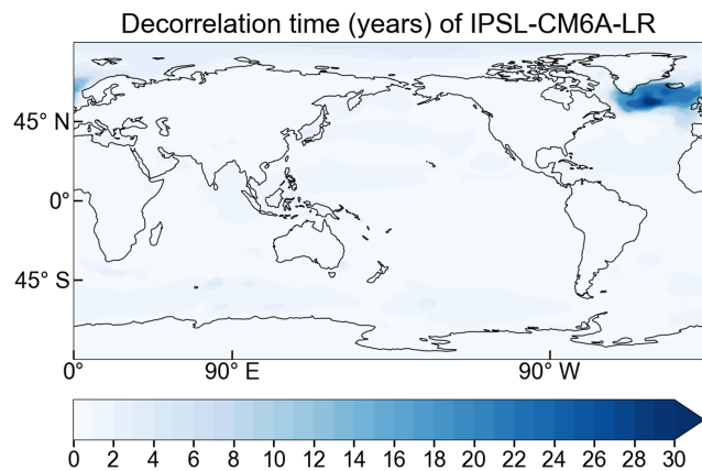
Figure A9. Decorrelation time of surface air temperature anomalies for IPSL-CM6A-LR, computed as the pointwise e-folding time of the autocorrelation function. Values are shown in years.
