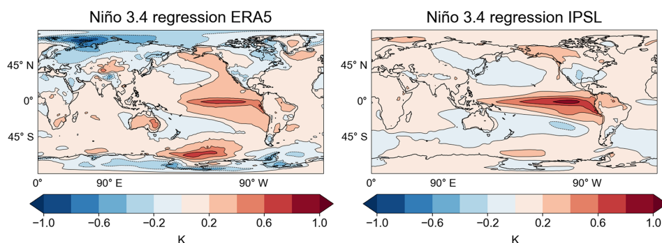
Figure A2. Regression maps of annual surface temperature anomalies onto the standardized Niño3.4 index in ERA5 (left) and in the IPSL-CM6A-LR past2k simulations (right), computed over their common 1940–2014 period. Regression coefficients are expressed in K.
