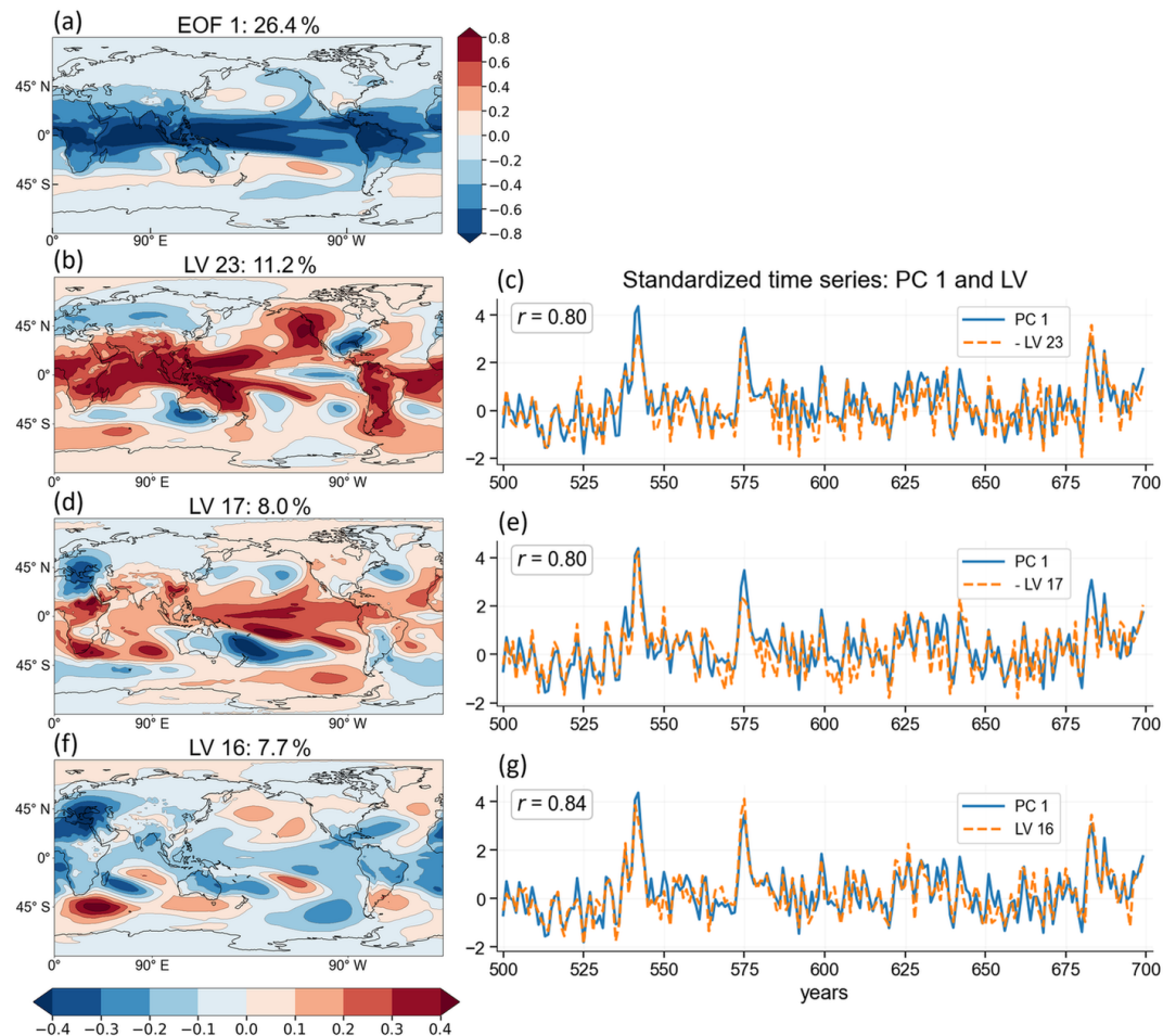
Figure A4. Variance structures associated with EOF 1 and AE latent vectors using a 30-dimensional latent space. Panel (a) shows the local variance explained by EOF 1 . The spatial patterns are dimensionless, as the EOF analysis is performed on the normalized covariance matrix. Panels (b), (d), and (f) display variance explained by AE latent vectors selected based on correlation \geq 0.7 with EOF 1 . Panels (c), (e), and (g) show the corresponding standardized time series over the first 200 years. Correlation coefficients are indicated.
