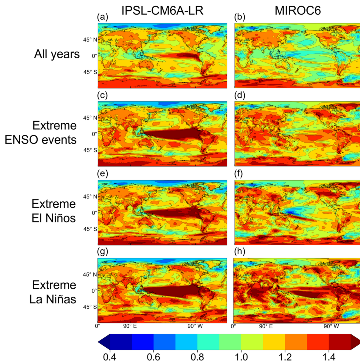
Figure A14. RMSE of one-year lead persistence forecasts with target piControl simulations during all years (a, b) extreme ENSO events (c, d), extreme El Niños (e, f) and extreme La Niñas (g, h). Results are shown for IPSL-CM6A-LR (left column) and MIROC6 (right column).
