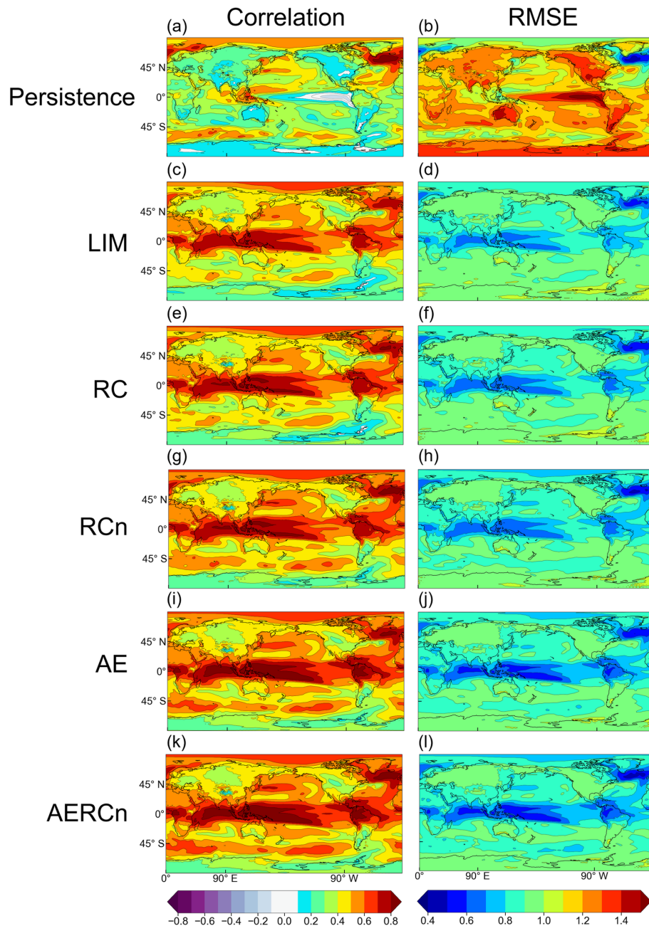
Figure 3. Spatial patterns of forecast skill at one-year lead time for IPSL-CM6A-LR. Correlation (left column) and RMSE (right column) are shown for Persistence (a, b), LIM (c, d), RC (e, f), RCn (g, h), AE (i, j), and AERCn (k, l).
