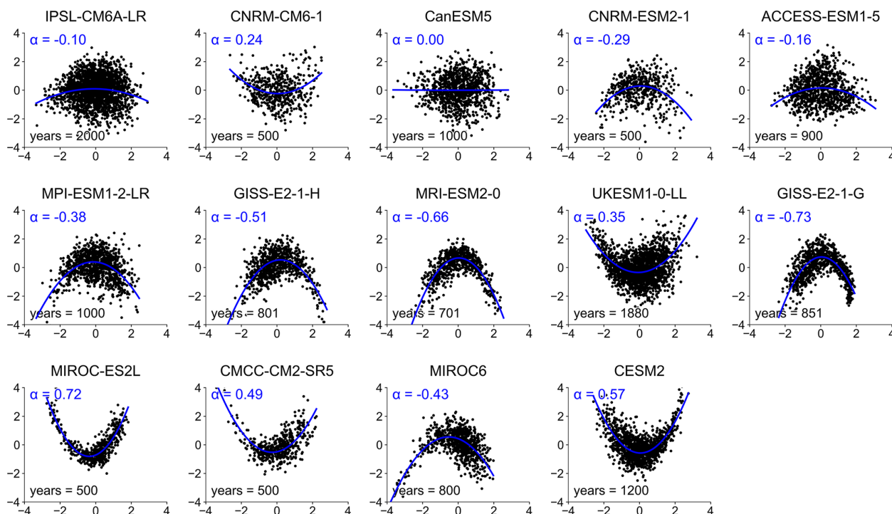
Figure A13. Phase-space representation of ENSO variability. Scatter plots of PC_1 versus PC_2 of DJF SST anomalies from CMIP6 piControl simulations are shown. The fitted quadratic curve provides the nonlinearity coefficient \alpha .
