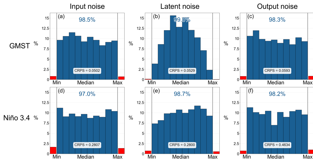
Figure A15. Reliability of AERCn ensemble forecasts generated with different perturbation strategies for IPSL-CM6A-LR. Rank histograms are shown for GMST (a–c) and Niño3.4 (d–f) using 100-member one-year lead ensembles. Columns correspond to input-space white-noise perturbations (left), latent-space white-noise perturbations (middle), and output-space noise based on the covariance of prediction errors (right). Blue bars indicate target frequency within ensemble deciles; red bars denote occurrences outside the ensemble spread. Percentages within the spread and mean CRPS values are indicated in each panel.
