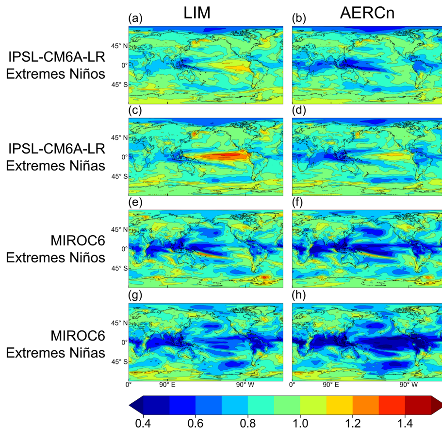
Figure 8. RMSE of one-year lead forecasts with target piControl simulations during extreme El Niño (a, b, e, f) and extreme La Niña (c, d, g, h) events. Results are shown for IPSL-CM6A-LR (a–d) and MIROC6 (e, f) using LIM (a, c, e, g) and AERCn (b, d, f, h).
