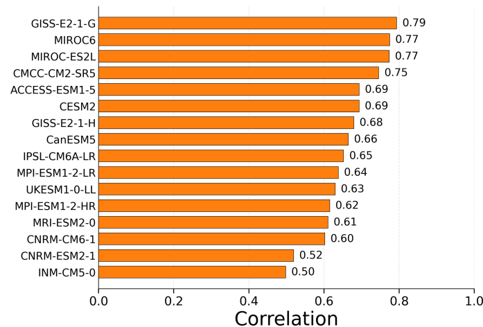
Figure A11. Spatially averaged tropical Pacific correlation at one-year lead time obtained using the RC emulator across 16 CMIP6 models. Models are ordered by decreasing skill.
