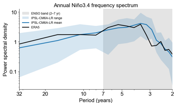
Figure A1. Power spectrum of the annual Niño3.4 index in ERA5 (black curve) and in the IPSL-CM6A-LR past2k simulations, computed over their common 1940–2014 period. The IPSL-CM6A-LR ensemble mean is shown by the blue curve, and the light-blue shading indicates the full range across ensemble members. The grey shading indicates the 2–7-year ENSO band.
