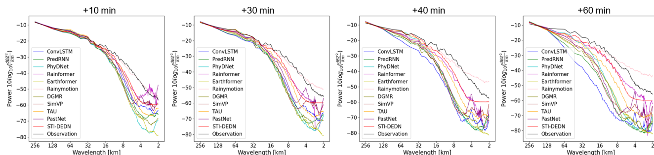
Figure 8. At the lead times of 10, 30, 40, and 60 min, the RAPSD curves at different precipitation thresholds for all methods in Case 2 were obtained.
