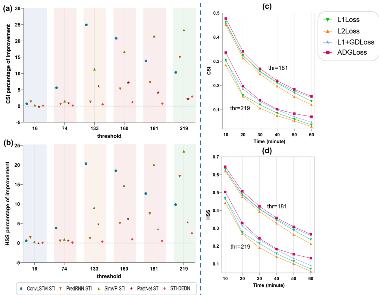
Figure 11. Panels (a) and (b) show the performance improvement of other methods after fusing the STI dual training framework at different thresholds compared with the original method. 0 value is equivalent to the original method without STI. Panels (c)–(d) show ablation experiments of different loss functions at thresholds 181 and 219.
