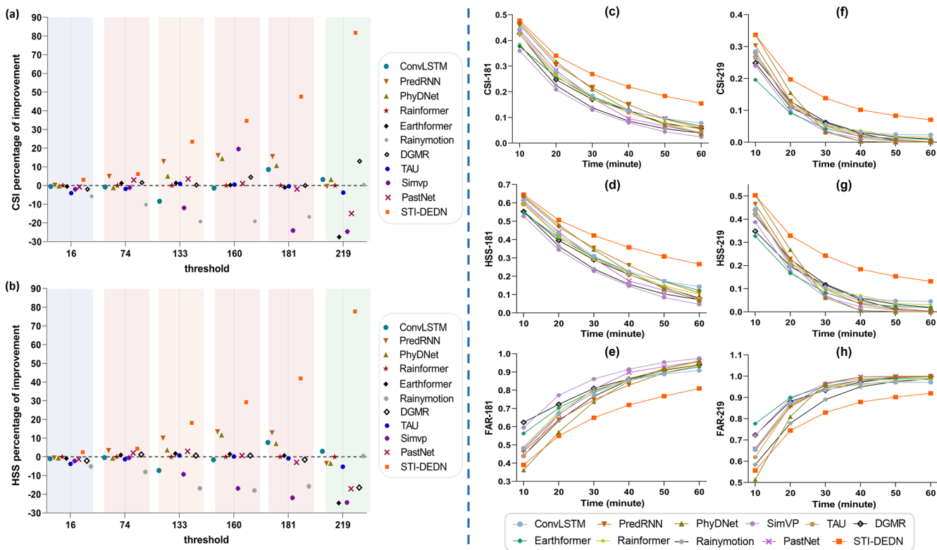
Figure 4. (a, b) scatter plots showing performance improvements at different measurement thresholds, using Rainformer as the baseline. Panels (c)–(h) show the time effect of each evaluation indicators of the model under the condition of high threshold precipitation.
