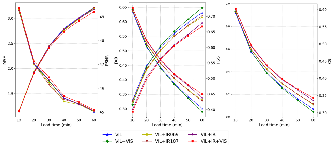
Figure 10. The index timeliness chart of all methods with a lead time of 60 min, MSE and FAR are all gradually increasing with time. PSNR, CSI and HSS are all gradually decreasing with time increasing.
