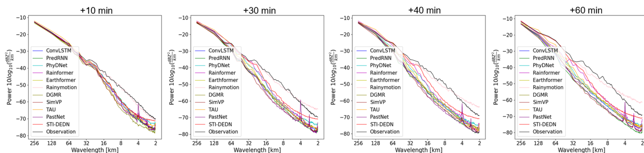
Figure 6. The radial mean power spectral densities (RAPSDs) for all methods in Case 1 were compared with the observed RAPSDs at 10, 30, 40, and 60 min lead times. The observed RAPSDs are shown as solid black lines.
