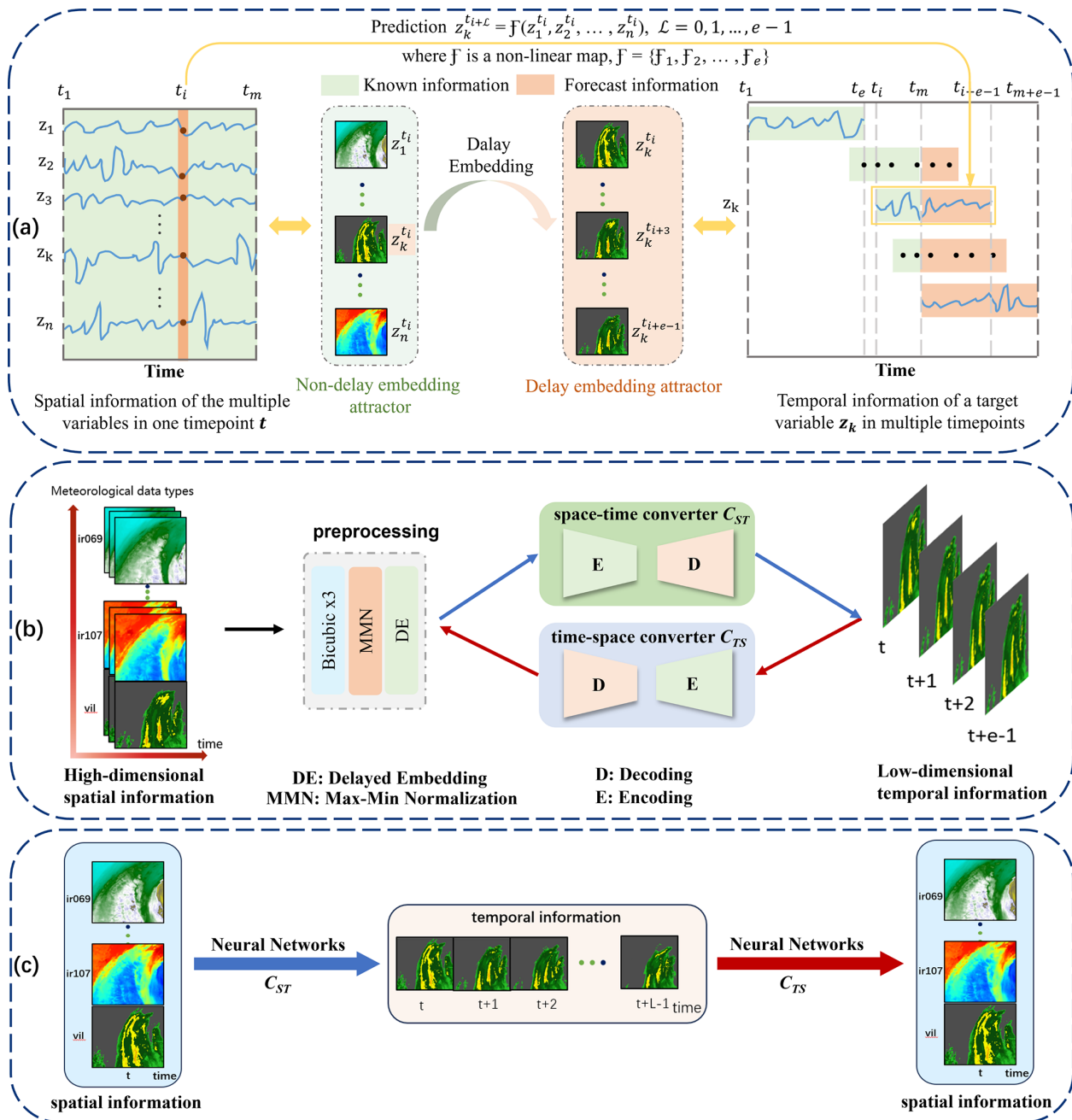
Figure 2. Schematic diagram of STI-DEDN. Panel (a) illustrates the transformation of the target variable z_k into a delayed embedding attractor using the delay embedding theorem, where the attractor exhibits a conjugate relationship with the non-delayed embedding attractor. The two attractors are connected through a nonlinear function \mathcal{F} , which maps the known spatial variable information to the temporal information of the unknown target variable z_k . The future values of z_k are represented as z_k^{t_i+\mathcal{L}} = \mathcal{F}(z_1^{t_i}, z_2^{t_i}, \dots, z_n^{t_i}) , \mathcal{L} = 0, 1, \dots, e-1 . Therefore, the key to predicting z_k lies in fitting the nonlinear function \mathcal{F} . Panel (b) demonstrates the overall training architecture of our proposed STI-DEDN, which mainly includes a space-time converter and a time-space converter, they are implemented using the same neural architecture. Panel (c) mainly illustrates the information flow process of STI-DEDN, the main STI equation corresponds to C_{ST} , and the conjugate STI equation corresponds to C_{TS} .
