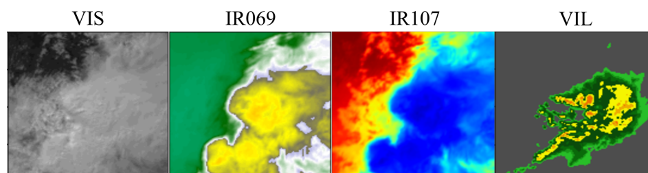
Figure 1. Visualization of various variables in the SEVIR (Storm Event Imager) dataset. VIL, IR107, VIS, and IR069 represent the radar vertical liquid water content, the satellite infrared longwave window, the visible satellite imagery, and the satellite mid-level water vapor, respectively. Among them, VIL represents precipitation data, while VIS, IR107 and IR069 serve as additional meteorological information.
