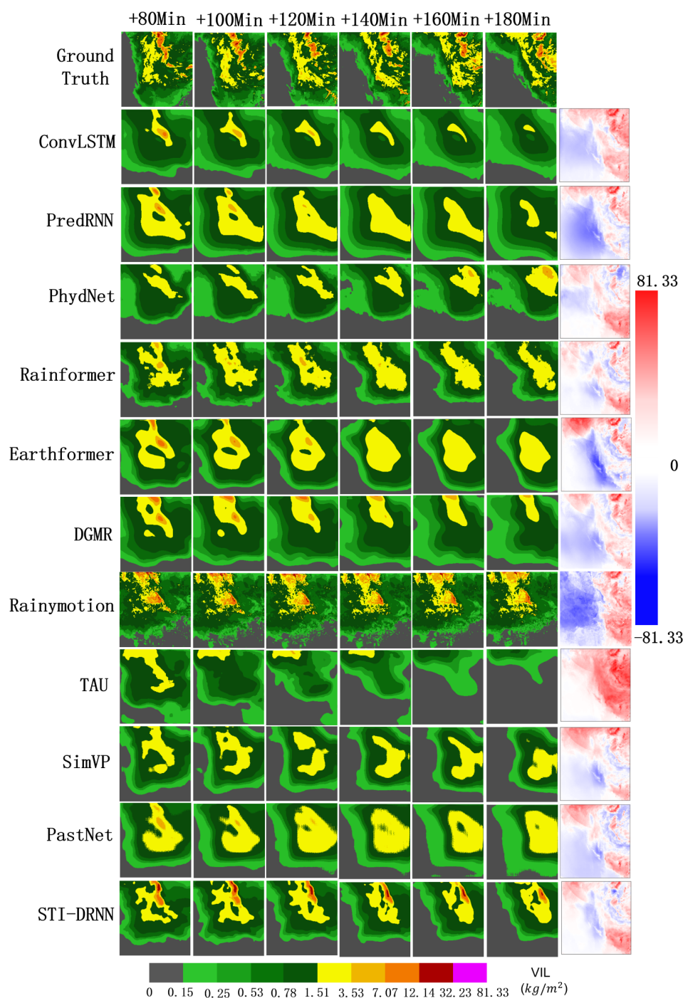
Figure 9. Visualization of precipitation maps and error heatmaps for all methods in the long-term experiment of Case 3.
