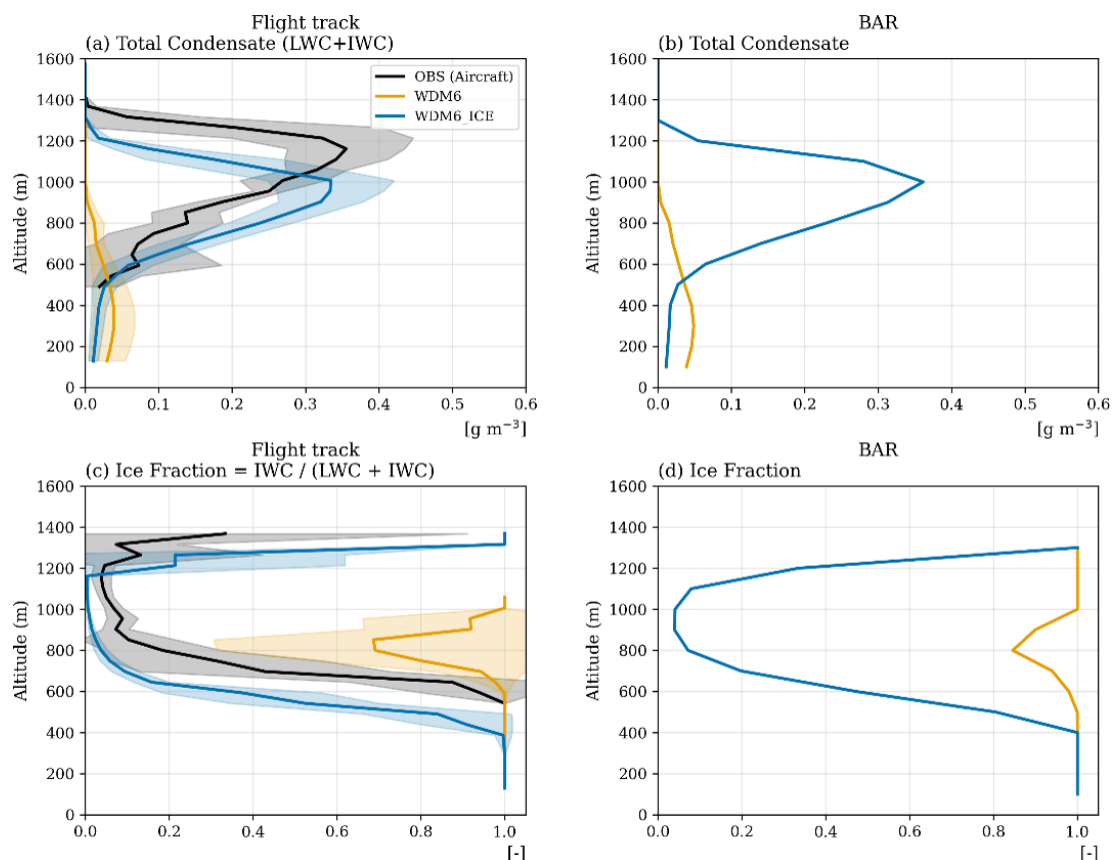
Figure 4. Vertical profiles of (a, b) total condensate (LWC + IWC) and (c, d) ice fraction ( IWC/(LWC+IWC) ; IWC: q_i + q_s + q_g ). The left column (a, c) shows profiles sampled along the flight track of Flight 10a, and the right column (b, d) shows the time-averaged (12:00 UTC 9 October–11:00 UTC 10 October 2004) profiles at BAR. Black lines represent aircraft observations (01:10–02:00 UTC 10 October 2004) with gray shading indicating \pm 1\sigma . Colored lines denote model simulations sampled along the track between 01:00–02:00 UTC, WDM6 (orange) and WDM6_ICE (blue).
