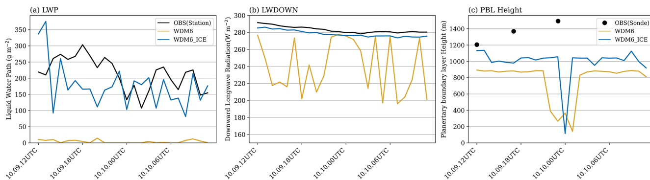
Figure 5. Time series (12:00 UTC 9 October–11:00 UTC 10 October 2004) at BAR of (a) liquid water path (LWP), (b) downward longwave radiation (LWDOWN), and (c) planetary boundary layer (PBL) height. Observations are shown in black, with station time series in (a) and (b) and radiosonde-derived estimates in (c) as filled circles for the three radiosonde times (12:00, 17:00, and 23:00 UTC 9 October 2004).
