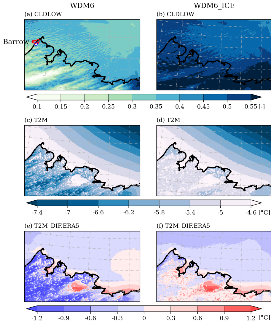
Figure 2. Time-averaged (12:00 UTC 9 October–11:00 UTC 10 October 2004) spatial distributions over domain D03 from (left column) WDM6 and (right column) WDM6_ICE simulations: (a, b) low-level cloud fraction (CLDLow; below 1500 m), (c, d) T2M, and (e, f) T2M differences (simulation – ERA5). The red box in (a) indicates the flight track area during the analysis period (01:00–02:00 UTC 10 October 2004).
