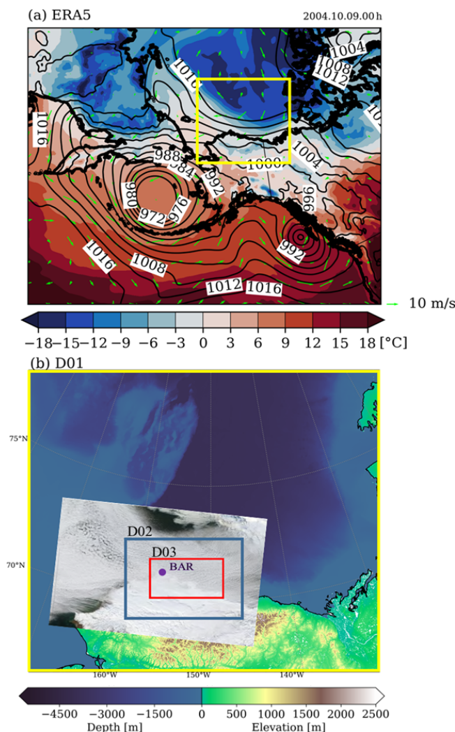
Figure 1. (a) ERA5 data showing sea level pressure (contours), 2 m temperature (shading), and 10 m wind (vectors) at 00:00 UTC 9 October 2004. The yellow box indicates the WRF model domain (D01). (b) Nested model domains with D01 (18 km resolution), D02 (6 km resolution), and D03 (1-km resolution). Ocean depth and land elevation are shaded using the GEBCO_2023 grid (color bar at bottom), overlaid with the MODIS visible image at 00:00 UTC 9 October 2004 over the Arctic Ocean and northern Alaska. The location of Utqiagvik (Barrow; BAR) is marked.
