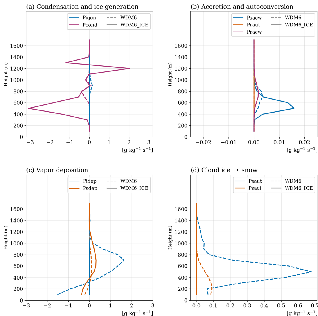
Figure 6. Time-averaged (12:00 UTC 9 October–11:00 UTC 10 October 2004) vertical profiles of microphysical process rates at BAR: (a) condensation and ice generation (Pigen, Pcond), (b) accretion and autoconversion (Psacw, Praut, Pracw), (c) vapor deposition (Pidep, Psdep), and (d) cloud ice to snow conversion (Psaut, Psaci). Dashed lines represent WDM6, and solid lines represent WDM6_ICE. Note that negative values in (a) indicate evaporation.
