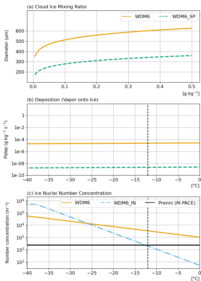
Figure 8. (a) Relationship between cloud ice mixing ratio and diameter in WDM6 (orange, solid) and WDM6_SP (bluish green, dashed). (b) Deposition rate of water vapor onto ice (assuming ice mixing ratio of 0.1 \text{ g kg}^{-1} and supersaturation of 10 %) as a function of temperature. (c) INP number concentration ( \text{m}^{-3} ) as a function of temperature for WDM6 and WDM6_IN (sky blue, dash-dot). The black line shows M-PACE observations (Prenni et al., 2007). Note that the observational upper limit of 500 \text{ L}^{-1} (DeMott et al., 2010) corresponds to 5 \times 10^5 \text{ m}^{-3} . The vertical dashed line marks -12^{\circ}\text{C} , representing the approximate cloud-top temperature during M-PACE.
