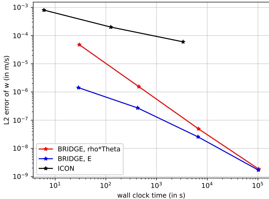
Work precision diagram for the BRZ2014 test
