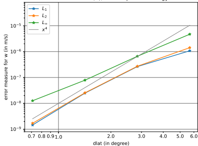
BRZ2014 test (A), Euler equation 'energy'
