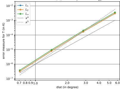
BRZ2014 test (A), Euler equation 'energy'
