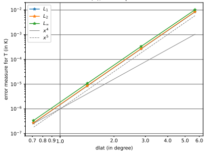
BRZ2014 test (A), Euler equation ' \rho \cdot \theta '
