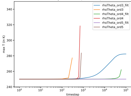
Euler equation set 1 ('rhoTheta')
