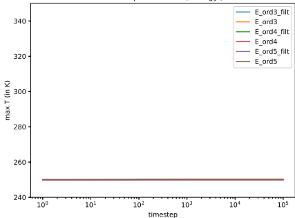
Euler equation set 2 ('energy')
