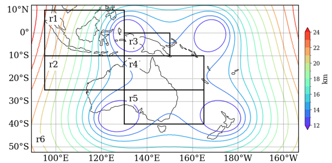
Figure 1. CCAM simulation domain with grid resolution ranging from 12 to 25 km, shown in contour colours. The study domain is divided into six subregions, labelled R1 to R6, representing the Maritime Continent, northwest Australia, southwestern pacific, northeast Australia, southeast Australia, and the whole simulated domain (50° S–10° N, 90° E–150° W), respectively.
