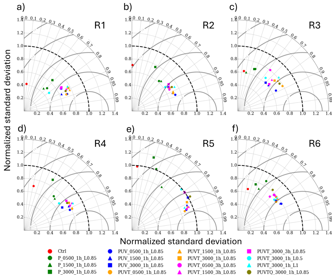
Figure 3. Taylor diagrams of daily precipitation averaged from December 2010 to March 2011 for six subregions (R1–R6), comparing 16 CCAM simulations with IMERG. Radial axis (distance from origin) represents standard deviation of the simulated precipitation (normalized by the observed standard deviation, IMERG). Angular axis (angle from x -axis) represents correlation coefficient between models and IMERG. Solid gray concentric arcs represent the centered root-mean-square error (RMSE) between the models and IMERG [a distance from the reference point on x -axis at (1,0)]. Coloured markers denote simulation groups (legend).
