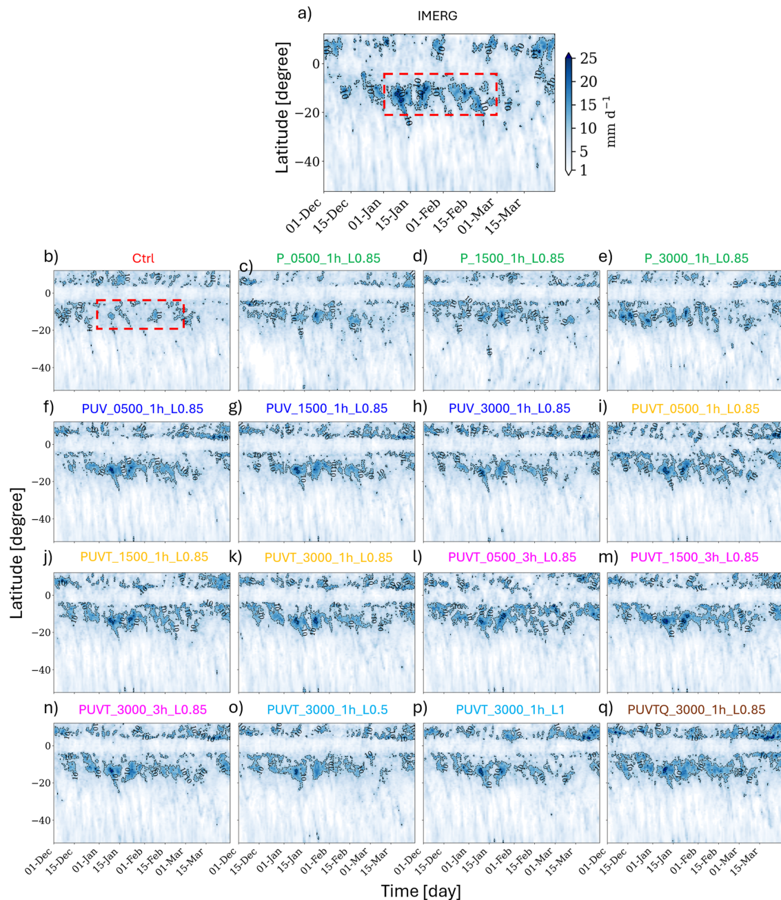
Figure 6. Hovmöller diagram of zonally averaged daily precipitation ( \text{mm d}^{-1} ) from the IMERG dataset for the period 1 December 2010 to 31 March 2011, averaged over 90^{\circ}\text{E} to 170^{\circ}\text{E} . Dash red box indicates the regions of MJO-related peak precipitation.
