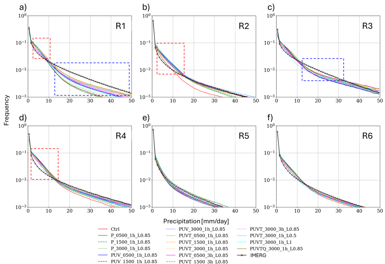
Figure 4. Frequency of daily precipitation intensity for IMERG and 16 CCAM simulations averaged over each region from December 2010 to March 2011. The dashed red and blue boxes indicate regions where the model respectively overestimates and underestimates precipitation compared to IMERG
