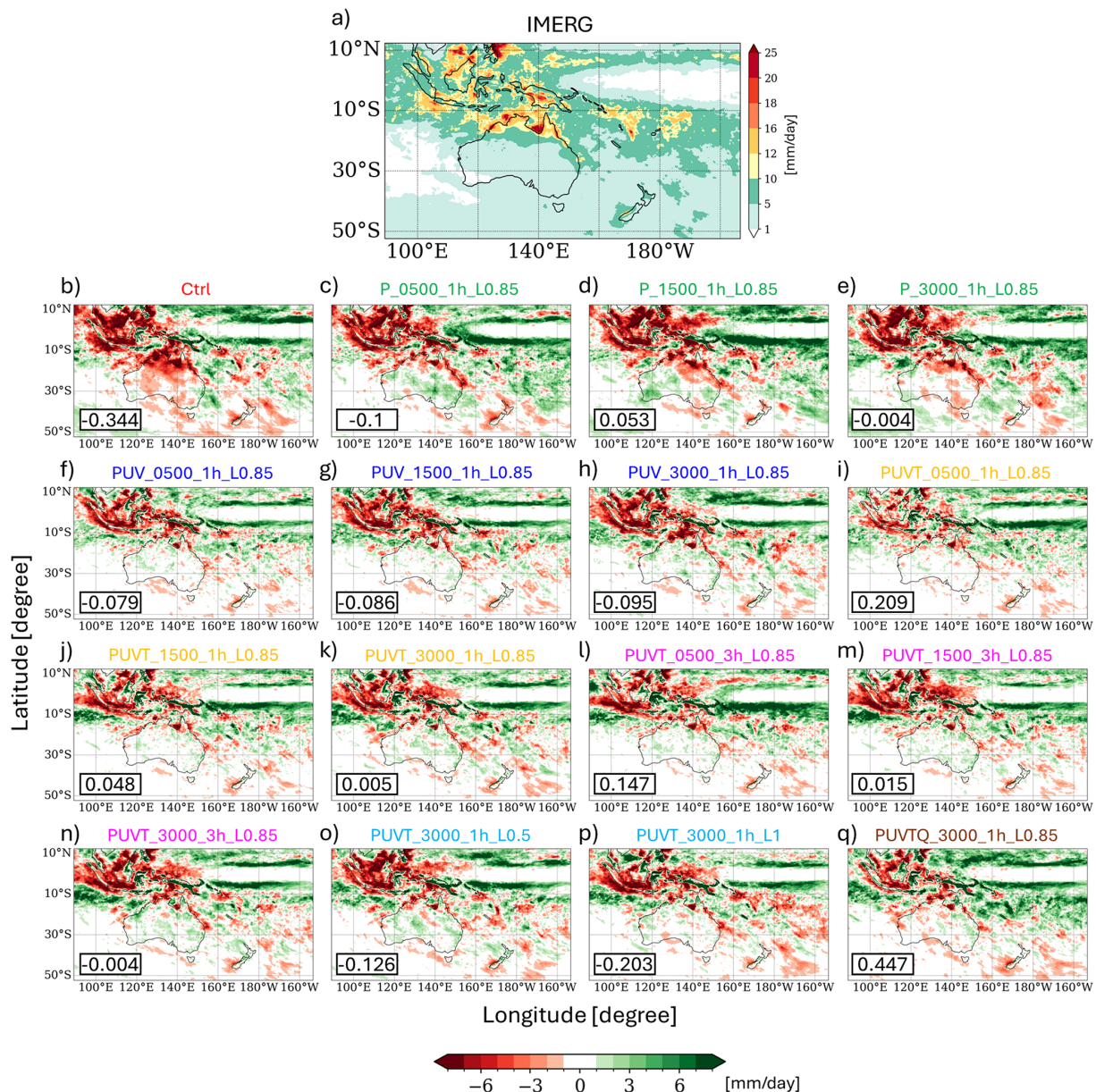
Figure 2. (a) The averaged precipitation from December 2010 to March 2011 over the study domain ( \text{mm d}^{-1} ) for IMERG; and (b–q) the bias relative to IMERG for each of the 16 simulations. Black box in the lower left indicates the domain averaged values. Different colours in the header of each panel indicate the grouped simulations in Table 1.
