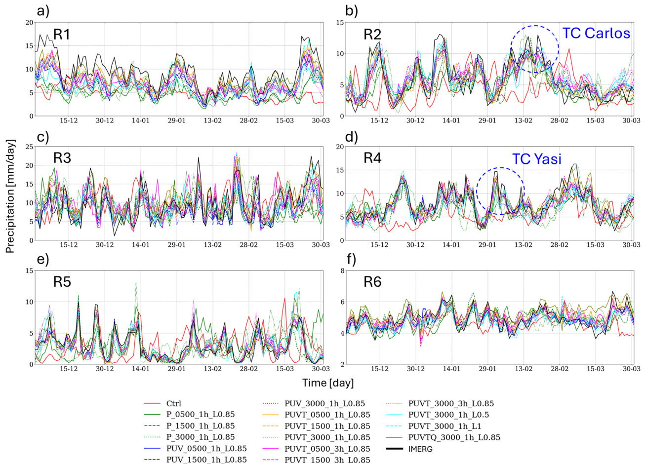
Figure 5. Time series of spatially averaged daily rainfall ( \text{mm d}^{-1} ) for IMERG and 16 CCAM simulations over the six from December 2010 to March 2011.
