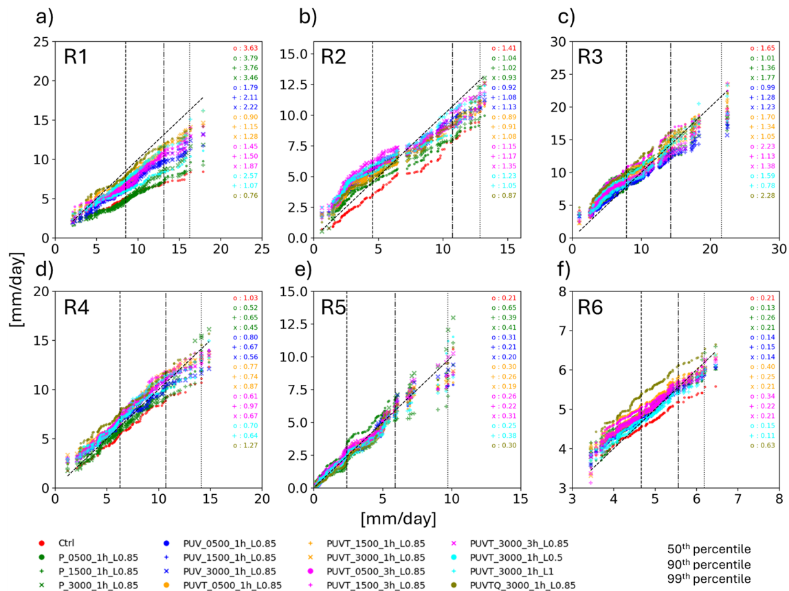
Figure 9. Quantile–quantile plots of regionally averaged daily precipitation ( \text{mm d}^{-1} ) against IMERG for six subregions. Coloured symbols denote different CCAM simulations (see legend). The dashed 1 : 1 line represents perfect agreement with observations. The numbers indicate the area formed by the 1 : 1 and model line. Numbers on the top right of each panel indicate the area between IMERG and CCAM in which the larger the number, the larger the difference between the two.
