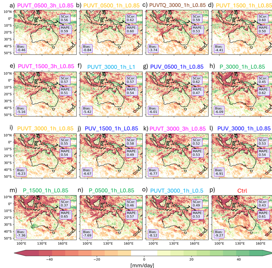
Figure 10. Bias of monthly maximum 1 d precipitation ( Rx1day ; mm\ d^{-1} ) from December 2010 to March 2011 relative to IMERG. Each panel shows one CCAM spectral nudging simulation (see labels), with shading indicating spatial bias across the CORDEX–Australasia domain. Statistics included in each panel are the spatial correlation (SCor), mean absolute percentage error (MAPE), and domain-averaged bias. Panels (a–p) are ordered from the wettest to driest model configurations.
