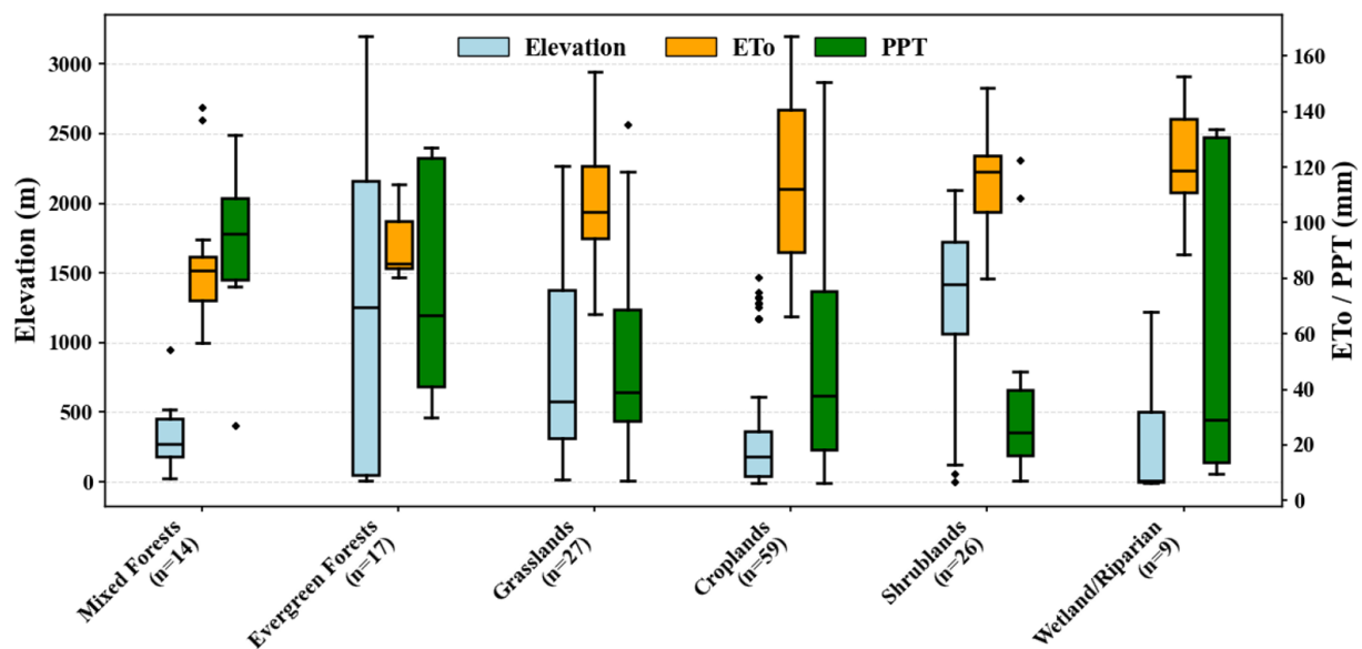
Figure 4. Box plots of describing range of elevation, average precipitation and reference ET from 2016 to 2022 at ground observation sites used in the model evaluation, separated by vegetation type.
