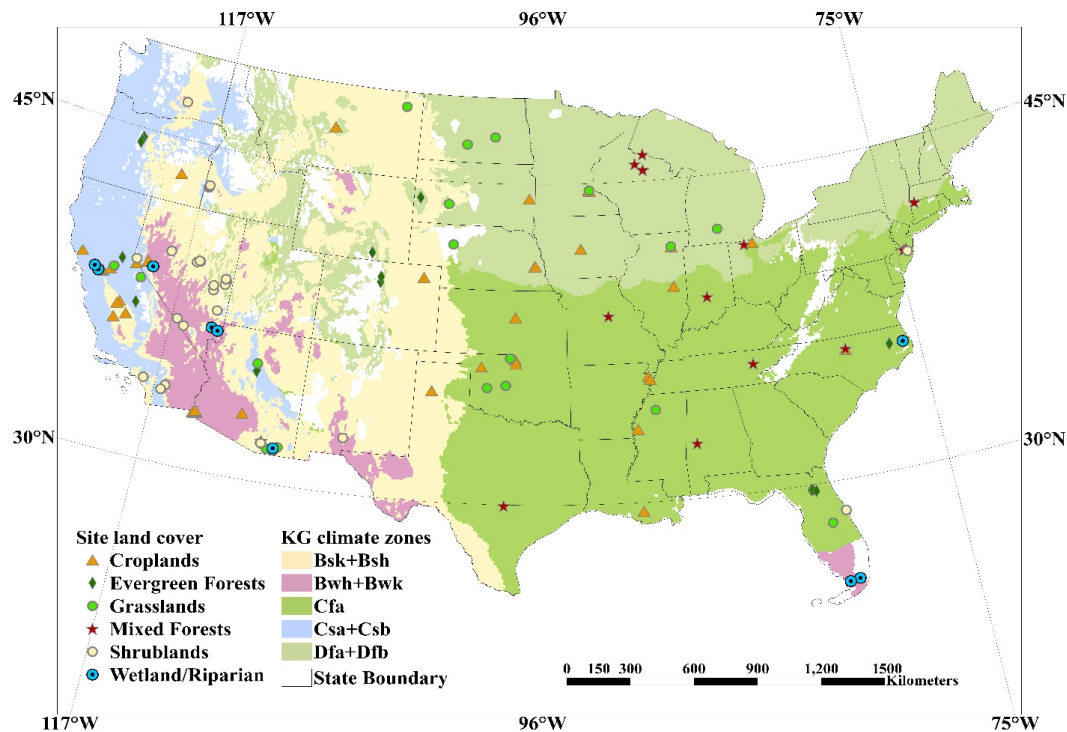
Figure 3. Locations and dominant vegetation type associated with ground observations used in the evaluation, overlaid on Köppen–Geiger climate zones.
