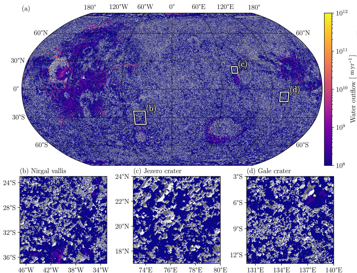
Figure D2. Water overflow at steady state with a GEL = 1 m and E = 1 \text{ m yr}^{-1} . The color bar represents the water flow accumulation. The areas where there is no outflow are symbolized by white shaded areas and sky blue areas represent the watershed and lake/ocean areas. The first line of zoomed plots shows the raw output data of the hydrological model which represents the water overflow associated to the watershed area.
