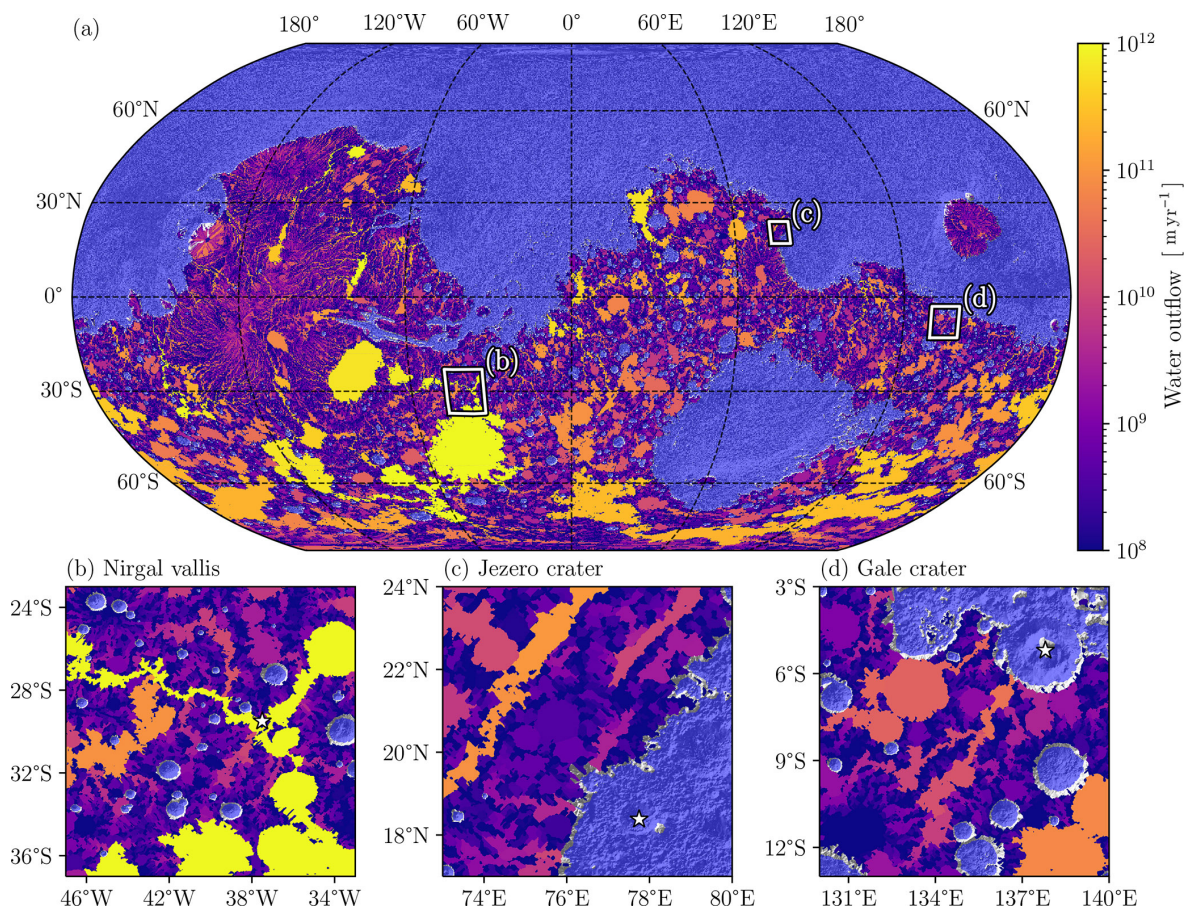
Figure D6. Water overflow at steady state with a GEL = 1000 m and E = 1 \text{ m yr}^{-1} . The color bar represents the water flow accumulation. The areas where there is no outflow are symbolized by white shaded areas and sky blue areas represent the watershed and lake/ocean areas. The first line of zoomed plots shows the raw output data of the hydrological model which represents the water overflow associated to the watershed area.
