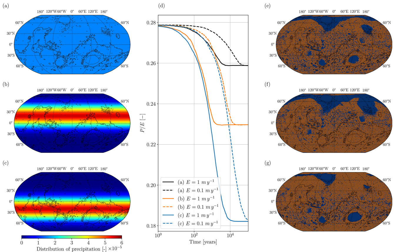
Figure C1. Simulations at steady state for a GEL = 100 m with a varying precipitation pattern: (a) homogeneous precipitation pattern, (b) precipitation is concentrated around 20° N and (c) precipitation concentrated around 20° S. Simulations were performed with a degraded MOLA topography at 1 pixel per degree resolution. (d) Evolution of the ratio P/E for the three precipitation rate patterns and two homogeneous evaporation rate: 1 \text{ m yr}^{-1} (solid curves) and 0.1 \text{ m yr}^{-1} (dashed curves). Distribution of water reservoirs at steady state for the three precipitation patterns: (e) homogeneous precipitation pattern, (f) precipitation is concentrated around 20° N and (g) precipitation concentrated around 20° S.
