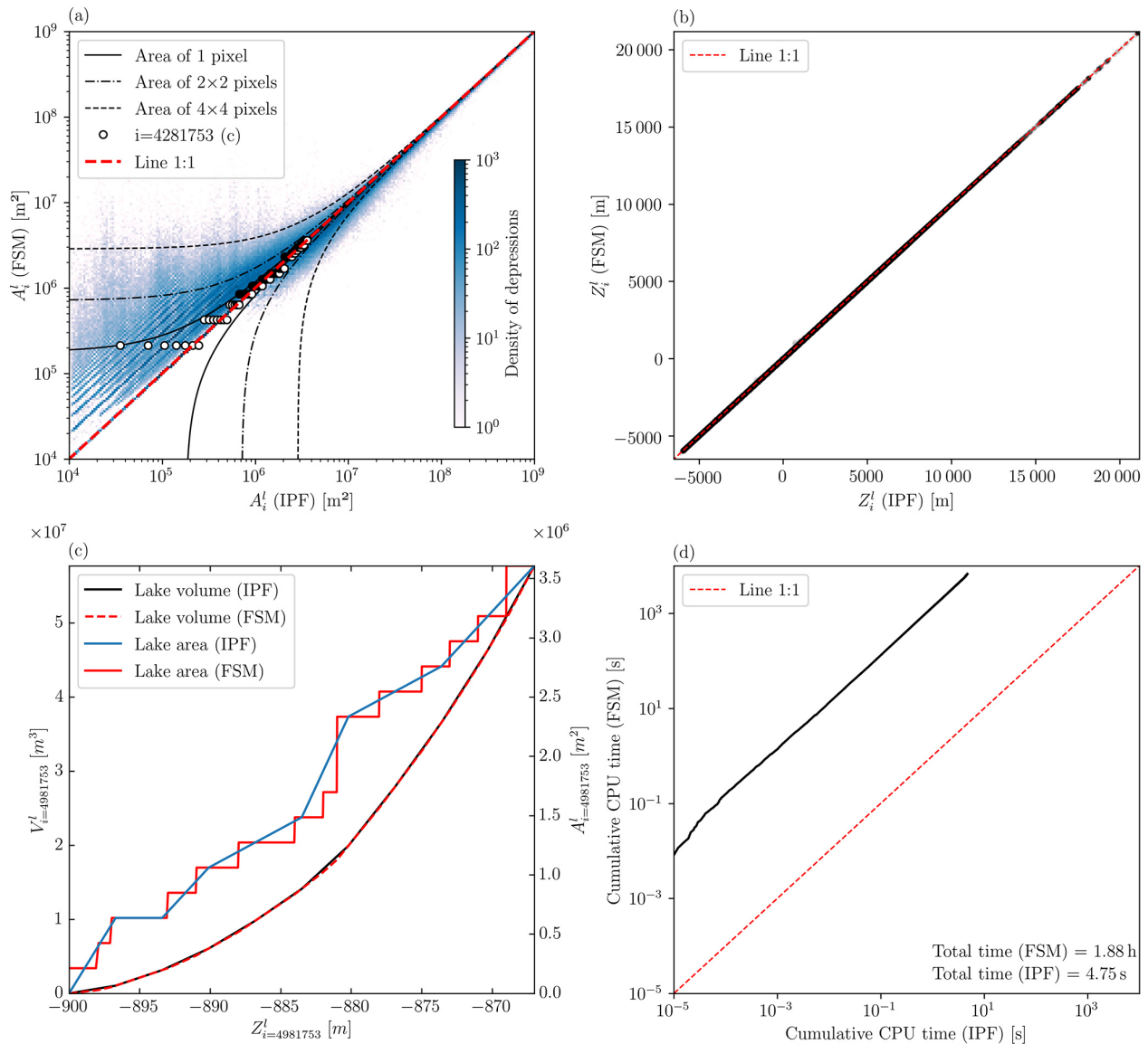
Figure A1. (a) Comparison of the lake area A_i^l computed using the interpolation of pre-computed lake functions (IPF) and the Fill-Spill-Merge (FSM) algorithm. The comparison is performed for all active depressions (2 059 551 depressions) shown in Fig. 5 (100 m GEL simulation). The color bar indicates the density of depressions. The three black lines (solid, dashed, and dash-dotted) represent errors of 1 pixel (423 × 423 m), 4 pixels, and 16 pixels, respectively. The white dots indicate the comparison between the blue and red solid curves in panel (c) for depression i = 4281753 . (b) Comparison of the lake elevation Z_i^l computed using the interpolation of pre-computed lake functions (IPF) and the Fill-Spill-Merge (FSM) algorithm. (c) Pre-computed hydrological functions (IPF) and functions computed with the Fill-Spill-Merge (FSM) algorithm for a single depression ( i = 4281753 ) shown in Fig. 3. (d) Comparison of computation times for the two algorithms. The total CPU time for the 2 059 551 depressions is 1.88 h for the Fill-Spill-Merge algorithm, compared with 4.75 s for the interpolation of pre-computed functions (IPF).
