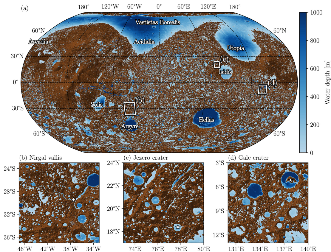
Figure 6. Distribution of water reservoirs (blue areas) at steady state with a GEL equal to 100 m. The color bar represents the water depth. The brown shaded areas represent the areas where the water cannot be accumulated. The white squares are zoomed areas on Nirgal Vallis' watershed (b), Jezero' watershed (c) and Gale' watershed (d). The white stars localized the Nirgal Vallis outlet (b), Jezero crater (c) and Gale crater (d).
