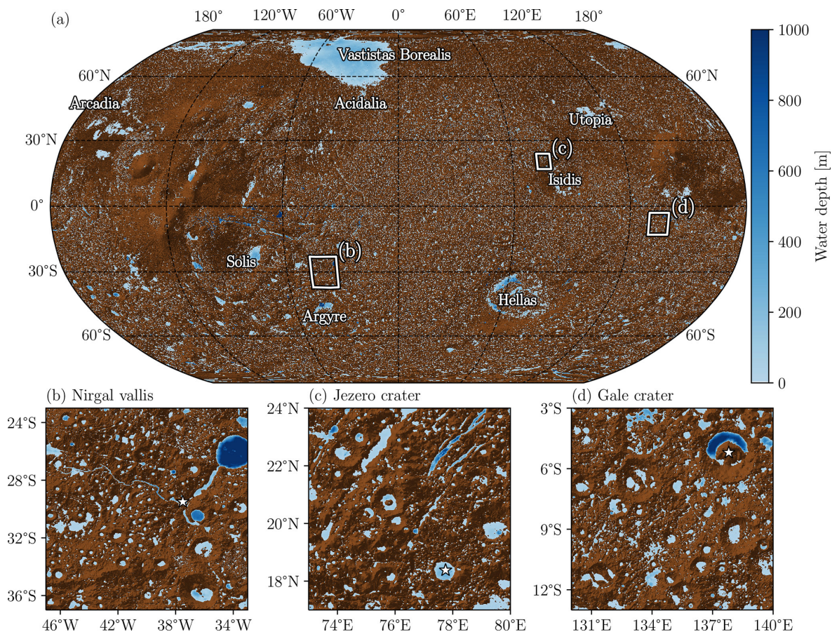
Figure D3. Distribution of water reservoirs (blue areas) at steady state with a GEL equal to 10 m. The color bar represents the water depth. The brown shaded areas represent the areas where the water cannot be accumulated. The white squares are zoomed areas on Nirgal Vallis' watershed (b), Jezero' watershed (c) and Gale' watershed (d). The white stars localized the Nirgal Vallis outlet (b), Jezero crater (c) and Gale crater (d).
