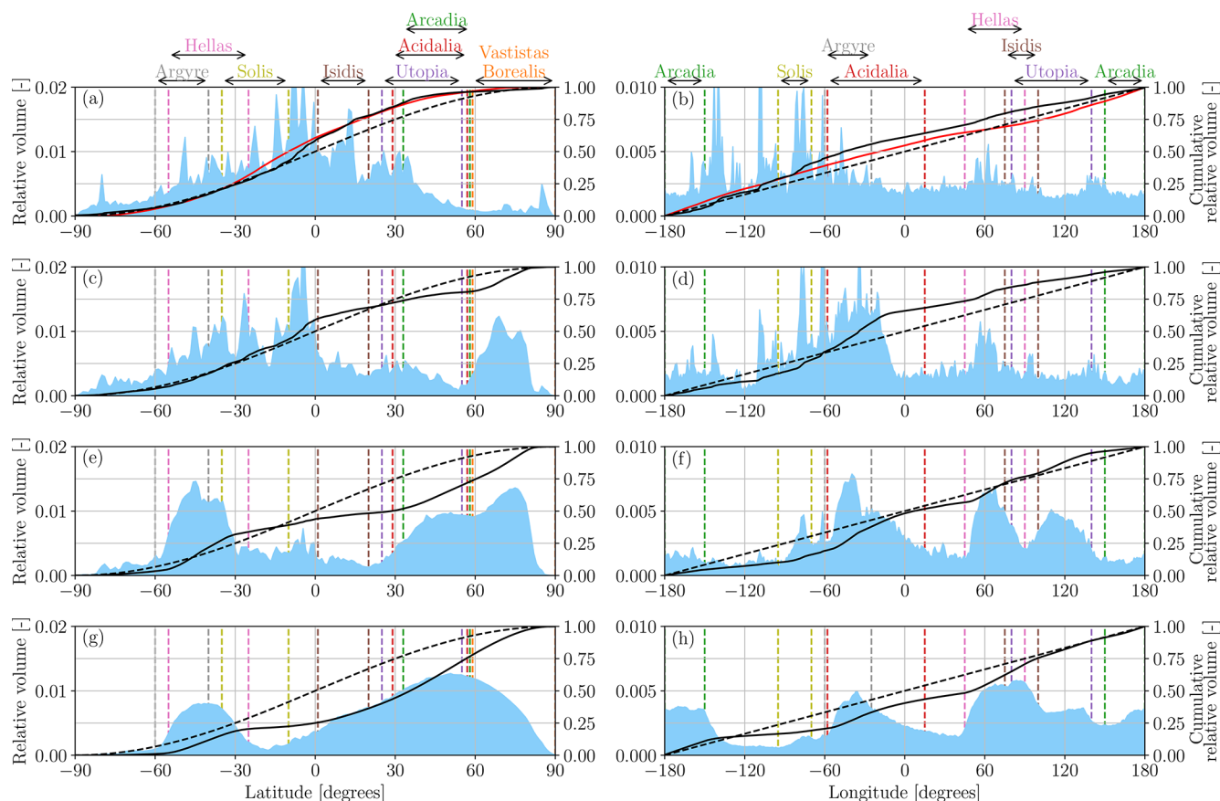
Figure 5. Distribution of water reservoirs at steady state for each GEL: 1 m (a, b), 10 m (c, d), 100 m (e, f), 1000 m (g, h). The blue areas represent the proportion of water relative to the total water volume (left y-axis) per degree of latitude (left column) and longitude (right column). The solid black lines show the cumulative relative water volume (right y-axis). The dashed black lines represent the cumulative relative water volume for a conceptual homogeneous distribution of water. The red curves on panels (a) and (b) represent the cumulative distribution of crater density (right y-axis) from Robbins and Hynek (2012).
