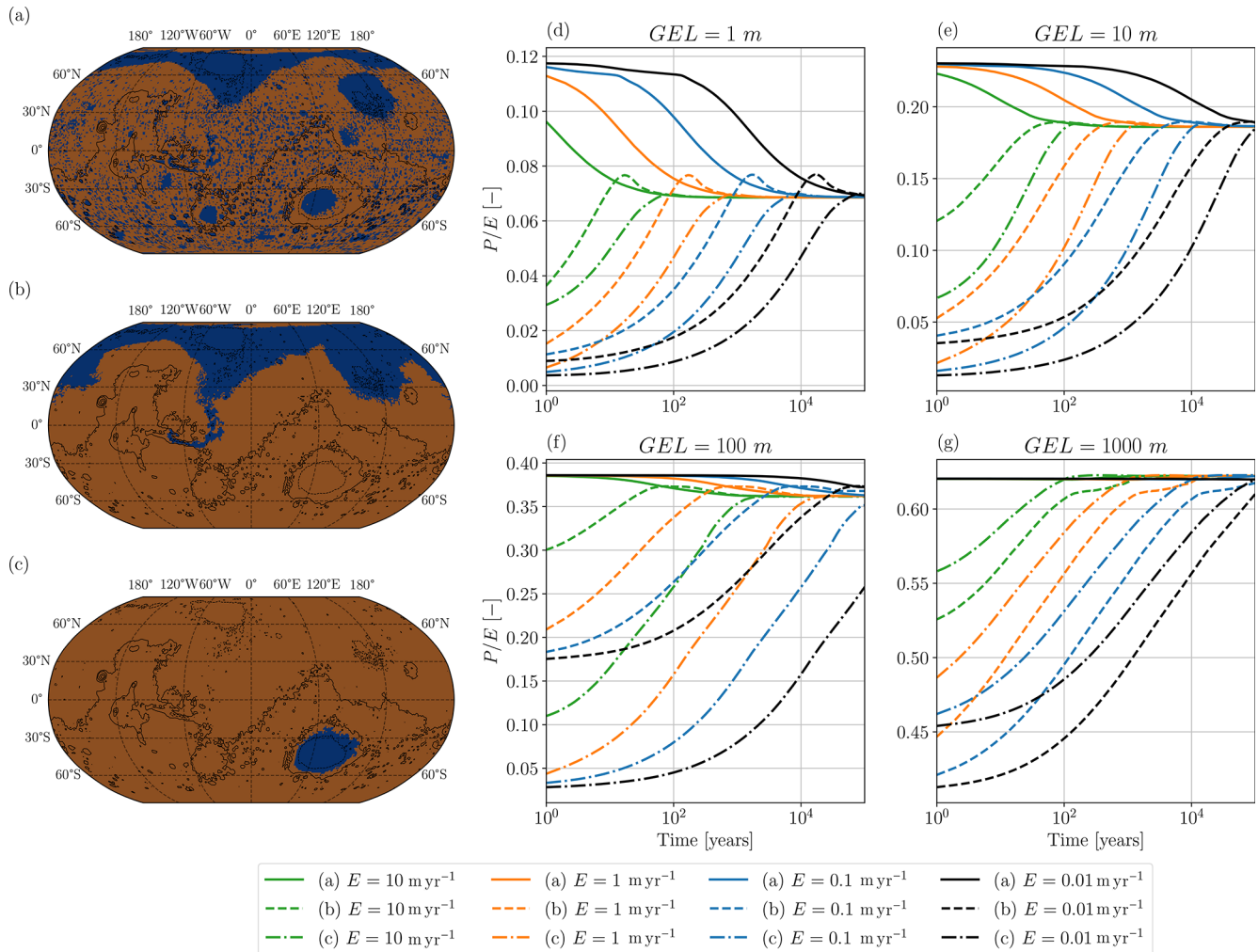
Figure 4. The three maps represent the initial states tested for a GEL = 100 m. The water is either distributed homogeneously (a), in the northern lowlands (b), or in the Hellas crater (c). The blue areas show the location of water reservoirs. The plots show the evolution of the P/E ratio over time for different GEL: 1 m (d), 10 m (e), 100 m (f), and 1000 m (g). Solid lines, dashed lines, and dotted-dashed lines represent simulations with homogeneous water distribution (a), distribution in the northern lowlands (b), and in the Hellas crater (c), respectively. Green, orange, blue, and black lines represent simulations with fixed evaporation rates of 10, 1, 0.1, and 0.01 \text{ m yr}^{-1} , respectively.
