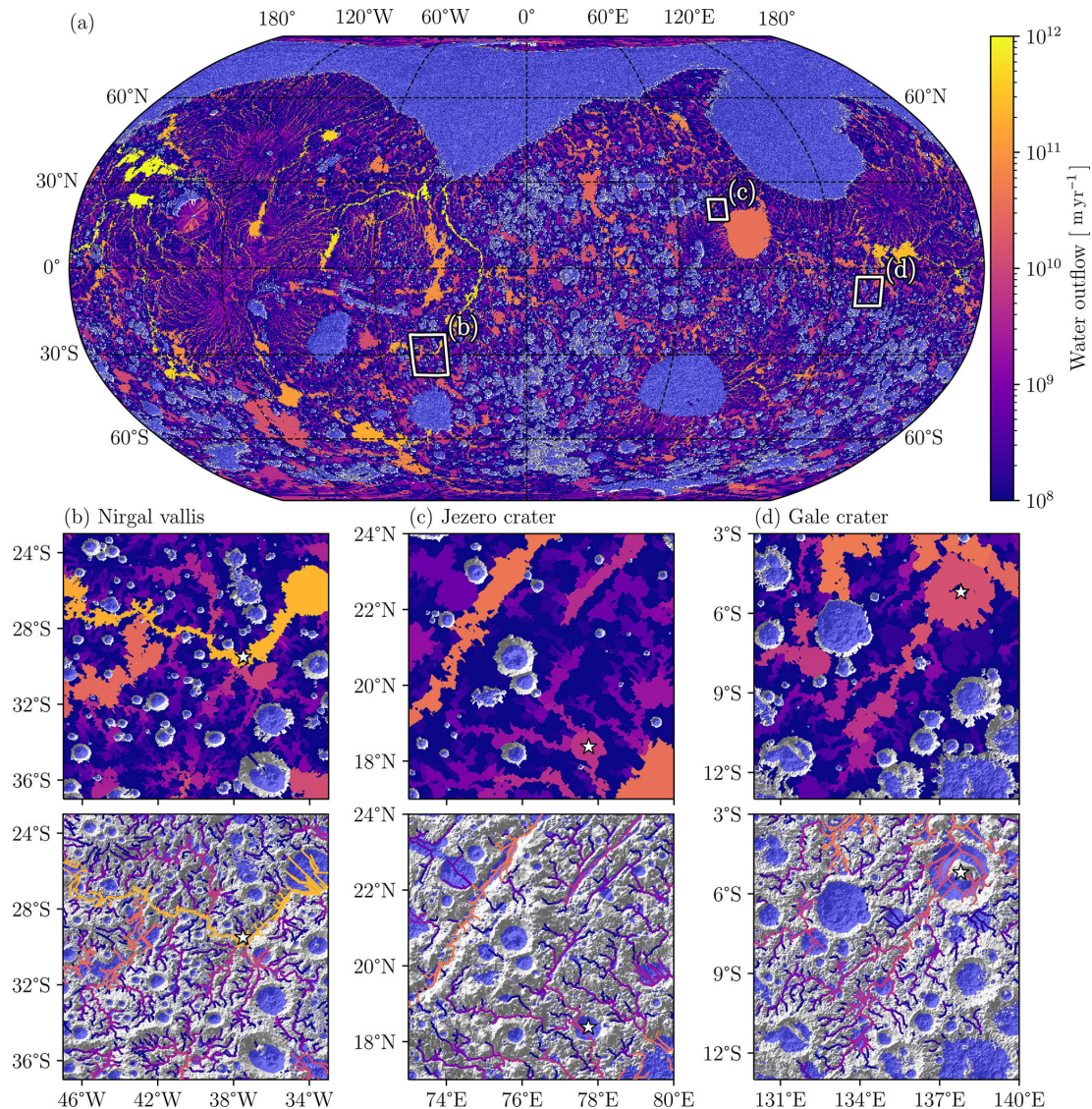
Figure 7. Water overflow at steady state with a GEL = 100 m. The color bar represents the water flow accumulation. The areas where there is no outflow are symbolized by white shaded areas and sky blue areas represent the watershed and lake/ocean areas. The first line of zoomed plots shows the raw output data of the hydrological model which represents the water overflow associated to the watershed area. The second line of zoomed plots shows the water overflow associated to the valley network, after post-processing explained in Sect. 2.4.
