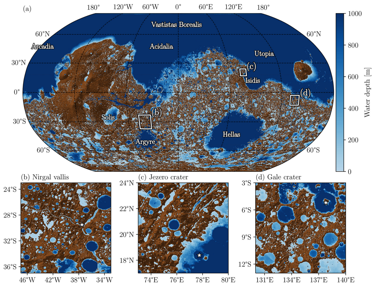
Figure D5. Distribution of water reservoirs (blue areas) at steady state with a GEL equal to 1000 m. The color bar represents the water depth. The brown shaded areas represent the areas where the water cannot be accumulated. The white squares are zoomed areas on Nirgal Vallis' watershed (b), Jezero' watershed (c) and Gale' watershed (d). The white stars localized the Nirgal Vallis outlet (b), Jezero crater (c) and Gale crater (d).
