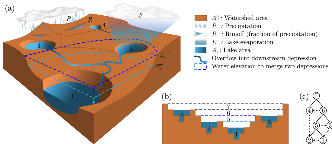
Figure 1. Representation of the water cycle on a conceptual topography with 4 leaf depressions. (a) 3D block represents the water flow from upstream to downstream. The links between the depressions, which represent streams, are symbolized by full blue curves. The sky blue dotted line represents the lake elevation where a depression No.1 can merge with a depression No.2 and create a new depression No.5. The dark blue dotted line represents the lake elevation where the depression No.5 merge with the depression No.3. The merge lines (blue and black dotted lines) are projected on the cross-section (b) of the 3D block diagram. (b) The dashed lines represent the minimum and maximum elevation limits of the depressions. (c) Binary tree of the depression hierarchy. Nodes No.1–4 are leaf depressions and nodes No.5–7 are meta-depressions. The black lines represent the merge into a new depression. The dotted arrows show the link with downstream depression. Adapted from Barnes et al. (2020).
