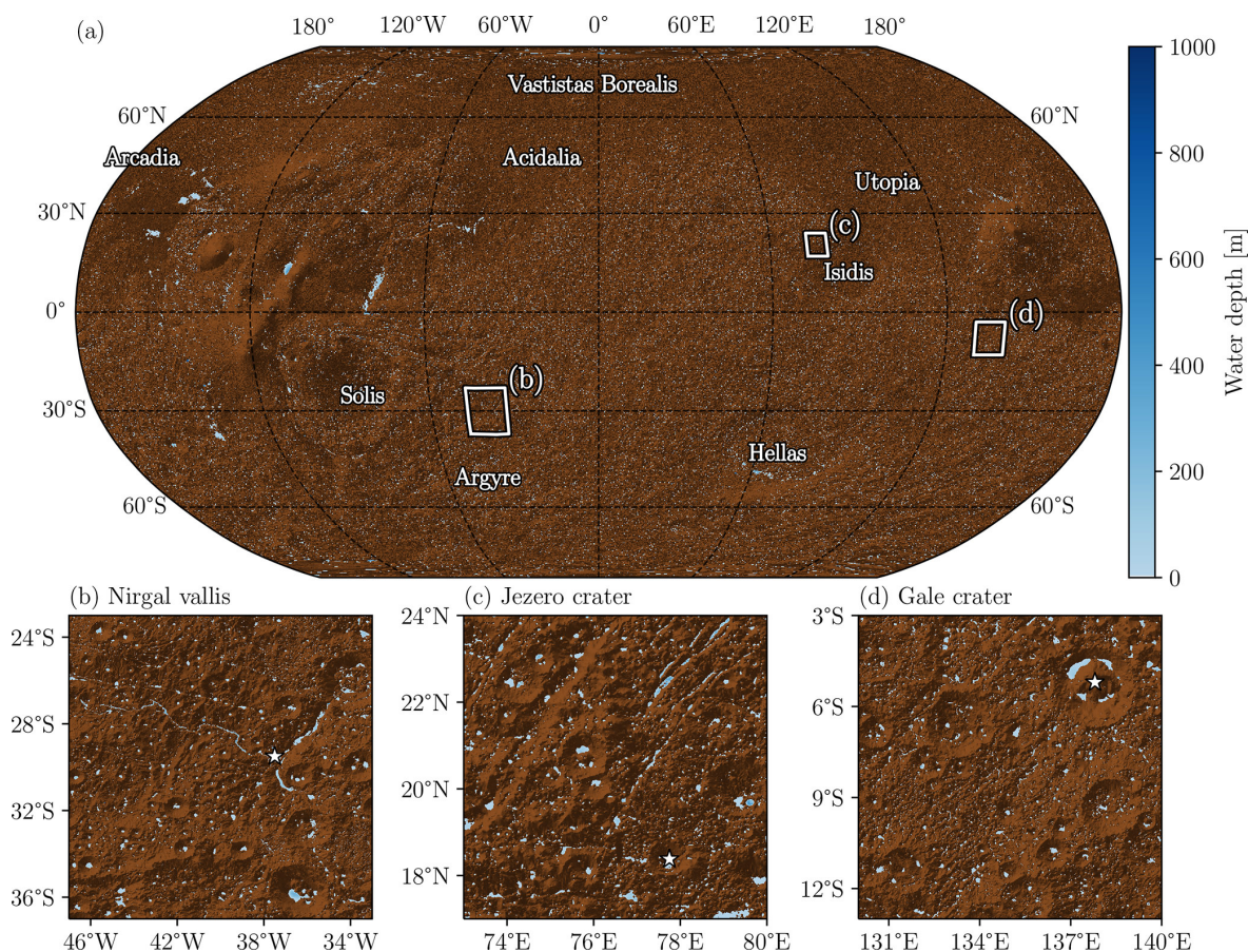
Figure D1. Distribution of water reservoirs (blue areas) at steady state with a GEL equal to 1 m. The color bar represents the water depth. The brown shaded areas represent the areas where the water cannot be accumulated. The white squares are zoomed areas on Nirgal Vallis' watershed (b), Jezero' watershed (c) and Gale' watershed (d). The white stars localized the Nirgal Vallis outlet (b), Jezero crater (c) and Gale crater (d).
