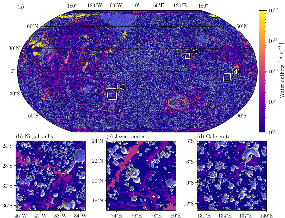
Figure D4. Water overflow at steady state with a GEL = 10 m and E = 1 \text{ m yr}^{-1} . The color bar represents the water flow accumulation. The areas where there is no outflow are symbolized by white shaded areas and sky blue areas represent the watershed and lake/ocean areas. The first line of zoomed plots shows the raw output data of the hydrological model which represents the water overflow associated to the watershed area.
