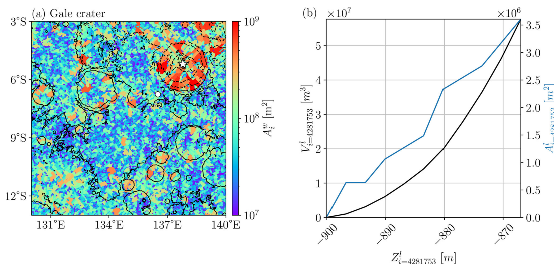
Figure 3. (a) 9777 watersheds of leaf depressions are represented on the zoomed area of the Gale crater watershed (Fig. 2d). Gale crater is localized by the white star. The color bar represents the watershed area A_i^w . (b) Example of pre-computed hydrological functions for a random depression ( i = 4281753 ) localized near to the Gale watershed by the white point (a). Evolution of the lake volume V_i^l (black line) and the lake area A_i^l (blue curve) as functions of the lake elevation Z_i^l .
