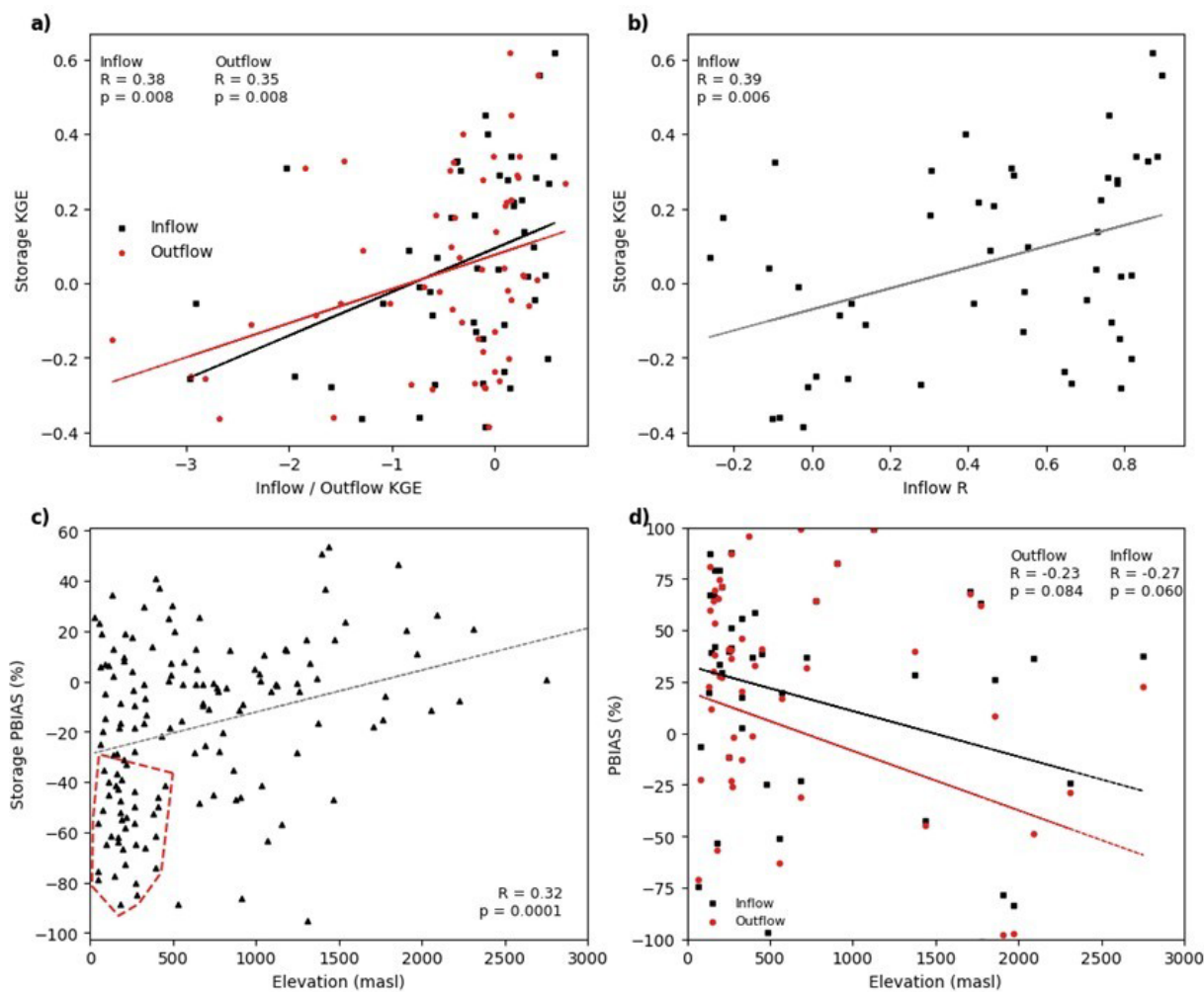
Figure B2. Scatter plots showing relationships between reservoir performance metrics, inflow characteristics, and elevation. Panels (a) and (b) include only reservoirs with monthly storage KGE greater than -0.42 , comparing monthly storage KGE with (a) monthly inflow.
