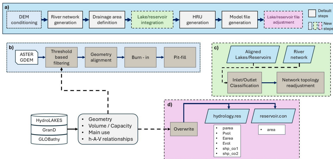
Figure 2. Overview of the (a) CoSWAT framework for model structure generation, with three new components introduced in this study: (b) DEM conditioning and preprocessing, (c) lake and reservoir integration into the network topology, and (d) adjustment of model files for reservoirs and lakes using global datasets (HydroLAKES, Grand, GLOBathy).
