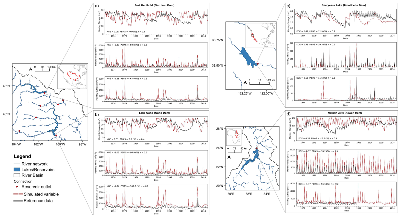
Figure 6. Simulated and reference data comparison for monthly storage (top), monthly inflow (middle), and monthly outflow (bottom) for four selected reservoirs: (a) Fort Berthold, (b) Lake Oahe in the Mississippi River system, (c) Berryessa Lake in the Sacramento River Basin, and (d) Nasser Lake in the Nile River Basin. Shaded areas in storage indicate periods with multiple observational sources differing in absolute value.
