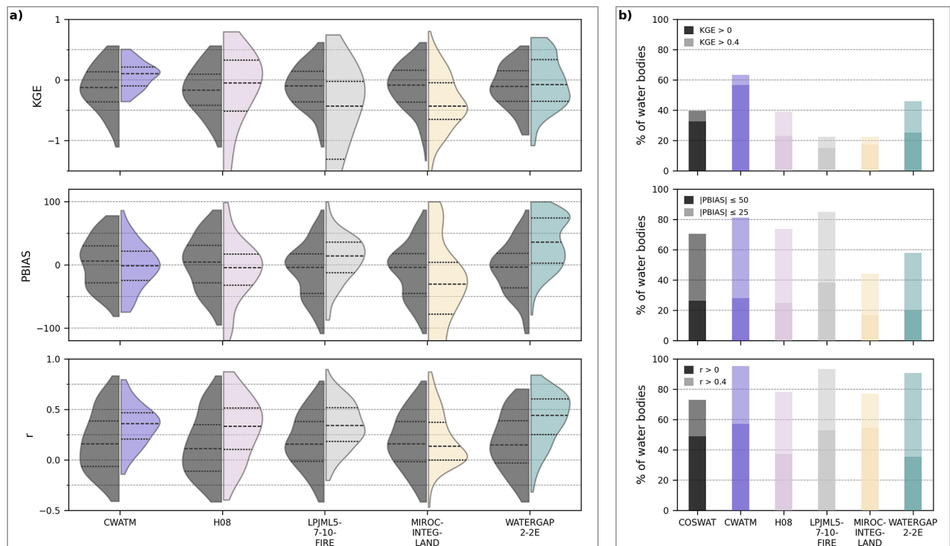
Figure 7. Performance comparison for mean monthly storage representation between CoSWAT with new implementations and five ISIMIP Global Water Sector models. Box (a) shows violin plots with the KDE distribution of CoSWAT (left panels) and the other models (right panels) for KGE, PBIAS, and r , considering only the water bodies available in the ISIMIP reference model. A dashed line represents the median, while dotted lines represent the first and third quartiles. Box (b) shows, for each model, the percentage of water bodies exceeding the “satisfactory” and “good” performance thresholds for KGE, PBIAS, and r , normalized by the total number of reservoirs represented by that model. For each model, the lighter shade corresponds to the “good” threshold and the darker shade to the “satisfactory” threshold. Outliers were not considered.
