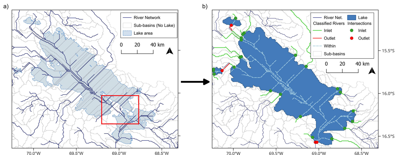
Figure 4. Example of Lake Titicaca in the model structure, (a) before network integration process, and (b) after integration, showing classified river network elements and points of intersection at the water body limits to define inlets and outlets. Rivers classified as “Within” are eventually excluded from the model structure. The area marked in red on box (a) represents the Lago Menor division, an example where complex topography leads to a network in which the lake cannot be integrated without the new integration approach.
