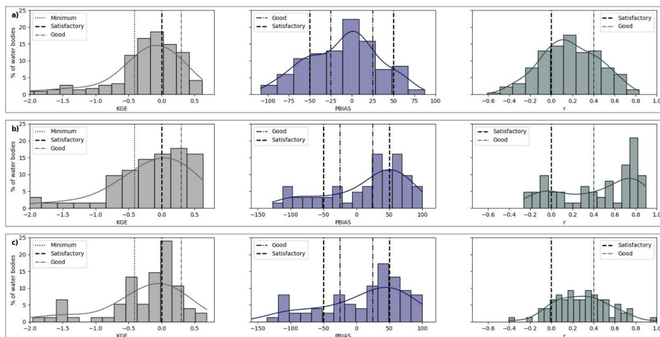
Figure 5. Distribution of KGE, PBIAS, and R related to model performance for monthly mean (a) storage, (b) inflow, and (c) outflow, using normalized histograms expressed as a percentage of evaluated water bodies for the corresponding variable. A kernel density estimate (KDE) curve is overlaid on each histogram to provide a continuous representation of the underlying probability distribution. Vertical reference lines indicate the established adequacy classifications for performance thresholds.
