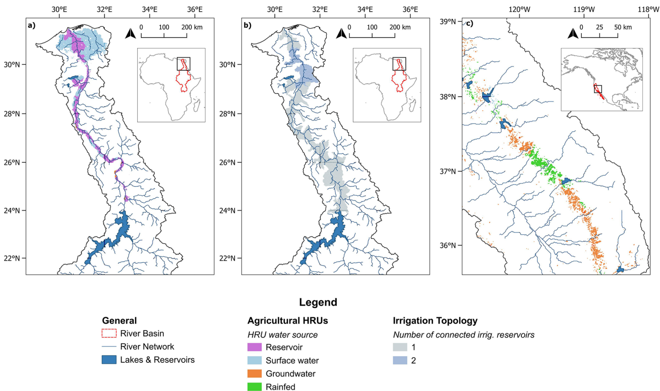
Figure 3. Irrigation water source assignment for agricultural HRUs and irrigation topology, illustrated for two contrasting regions: (a) a predominantly irrigated downstream section of the Nile River Basin, (b) the corresponding irrigation topology showing the number of connected irrigation reservoirs per sub basin, and (c) a section of the Pacific Seaboard in North America, where agricultural HRUs rely predominantly on groundwater or are rainfed.
