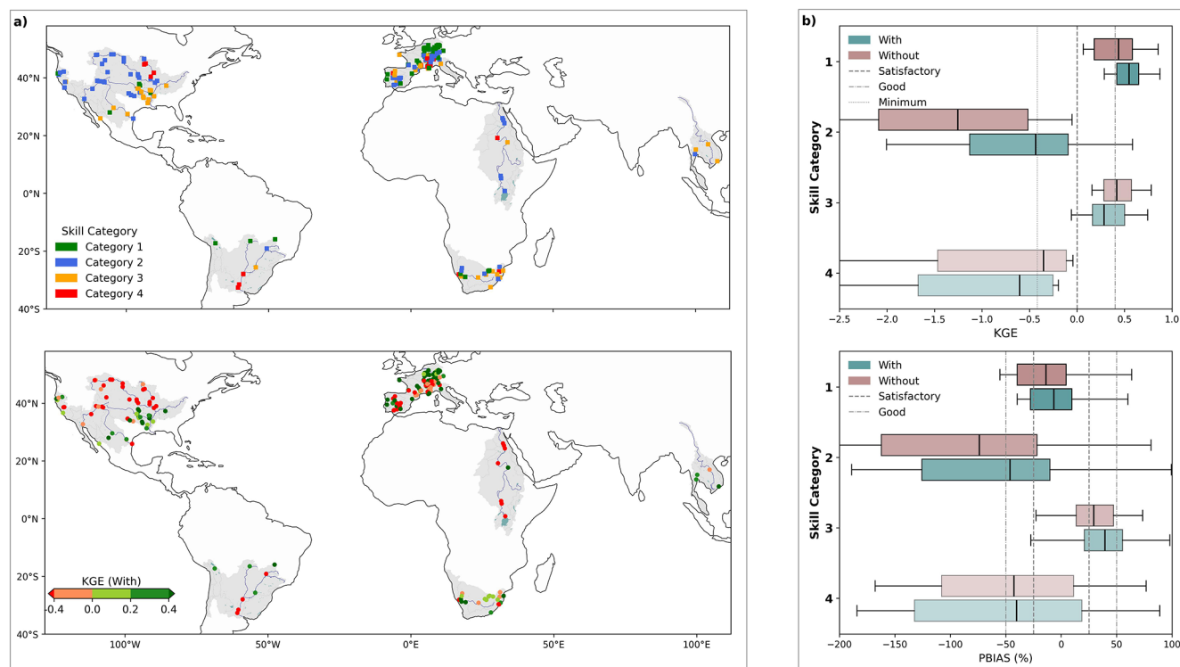
Figure 8. Monthly streamflow performance assessment. Box (a) shows the spatial distribution of stations with their corresponding skill category (top panel) and the KGE value of the model with new implementations (bottom panel). Box (b) shows the distribution of performance per skill categories for KGE (top panel) and PBIAS (bottom panel) with and without new implementations, as well as the performance classification thresholds.
