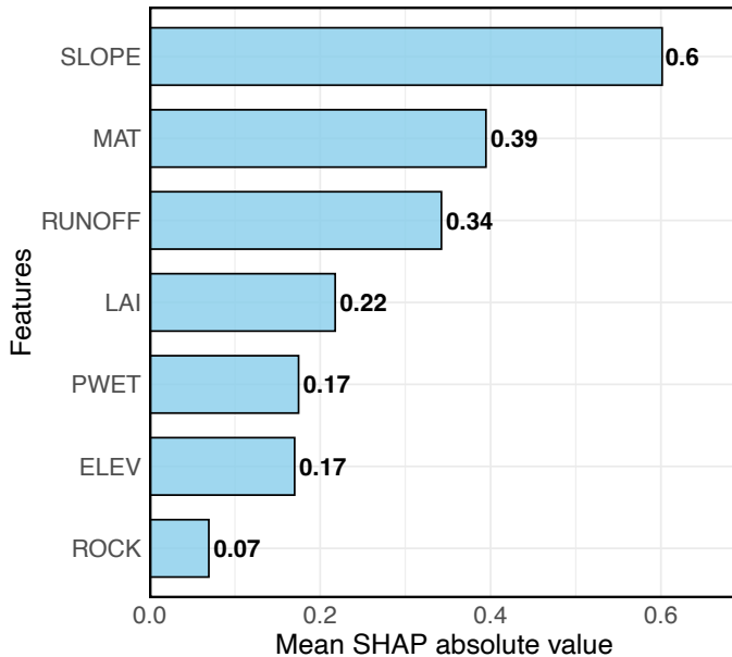
(a) SHAP Feature Importance
