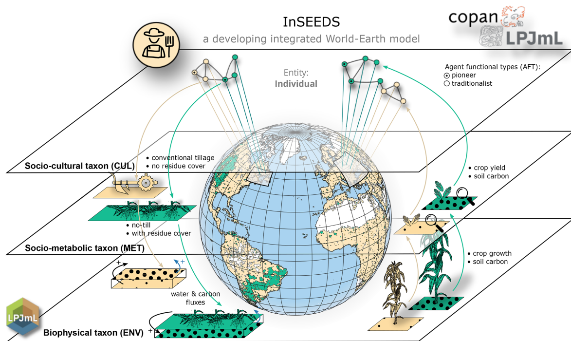
Figure 3. Detailed scheme of InSEEDS highlighted in Fig. 1 representing the feedback mechanisms among the taxons ENV, MET and CUL. Individuals who are either of type pioneer or of type traditionalist observe crop yields and soil carbon and make decisions on conservation/-conventional tillage to then be re-evaluated again.
