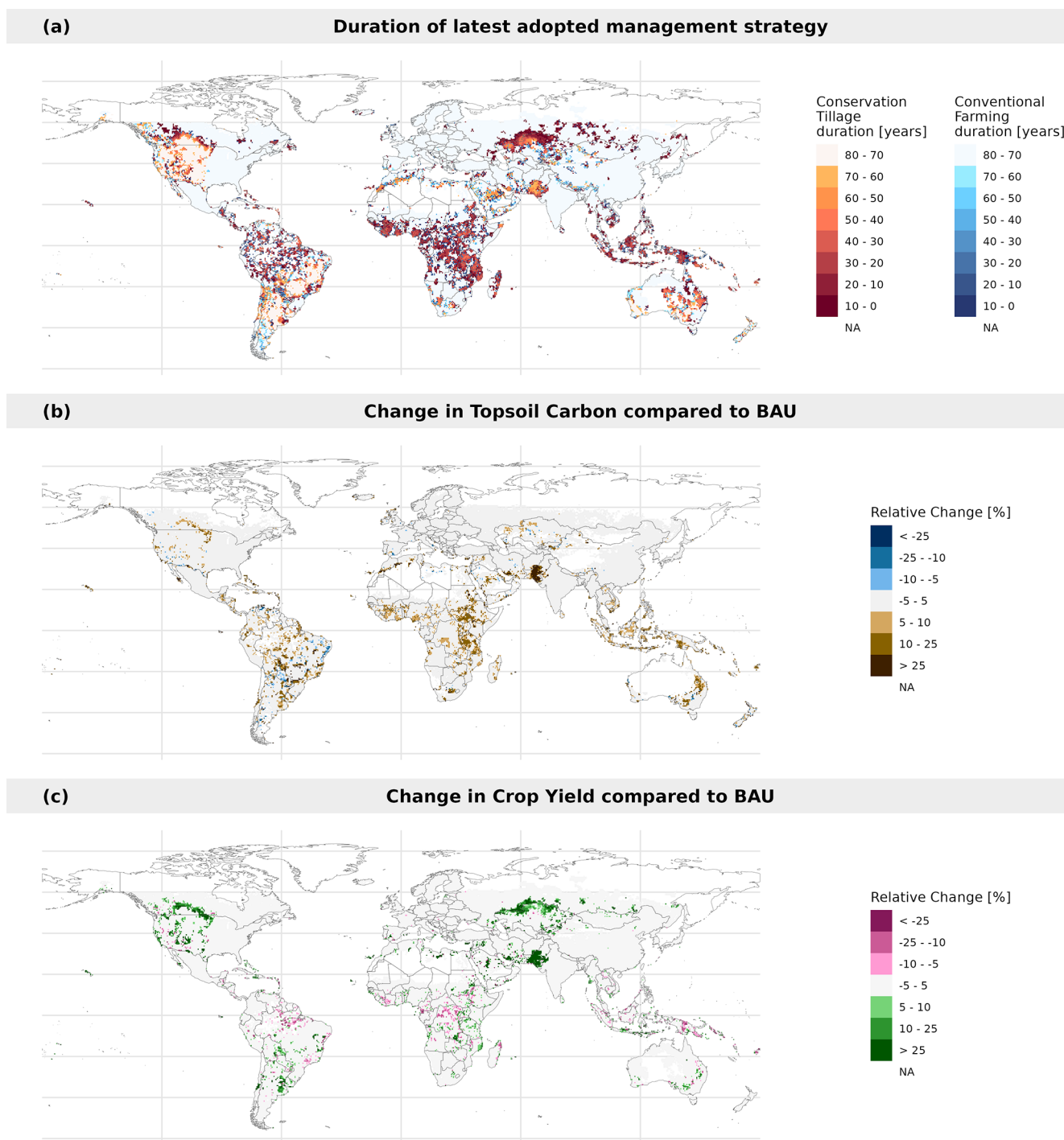
Figure 5. InSEEDS simulation of (a) global spreading of conservation tillage represented as years since last management switch (backwards from simulation end year 2100). The adoption and spatial spreading of conservation tillage is depicted in orange, and conventional farming adoption in blue. If the saturation of both colours decreases over time, this indicates that there will be no further change in strategy. Vice versa, the more saturated the colour, the more recent the change. (b) and (c) show the corresponding changes in topsoil carbon content and average crop yield in 2100 compared to a simulation without management changes (business-as-usual) until 2100.
