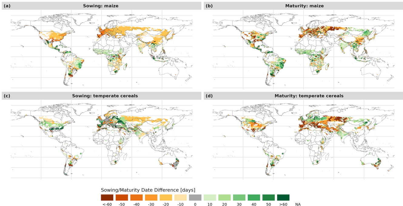
Figure 7. Recreated figure after Minoli et al. (2022a) (Fig. 1) showing the difference in simulated sowing (a) and maturing (b) between no adaptation and timely adaptation for a climate period 2080–2099 in an SSP460 scenario using ISIMIP3b data (Lange et al., 2024).
