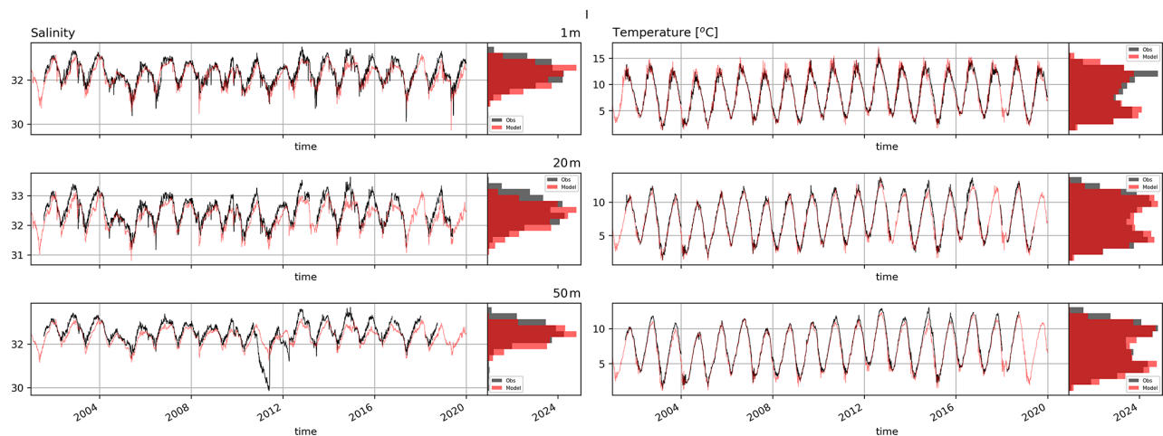
Figure A10. Time series of salinity in temperature of MOM6 (red) and NERACOOS mooring measurements (black) at buoy I.
