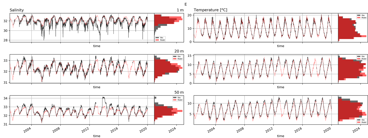
Figure A8. Time series of salinity in temperature of MOM6 (red) and NERACOOS mooring measurements (black) at buoy E.
