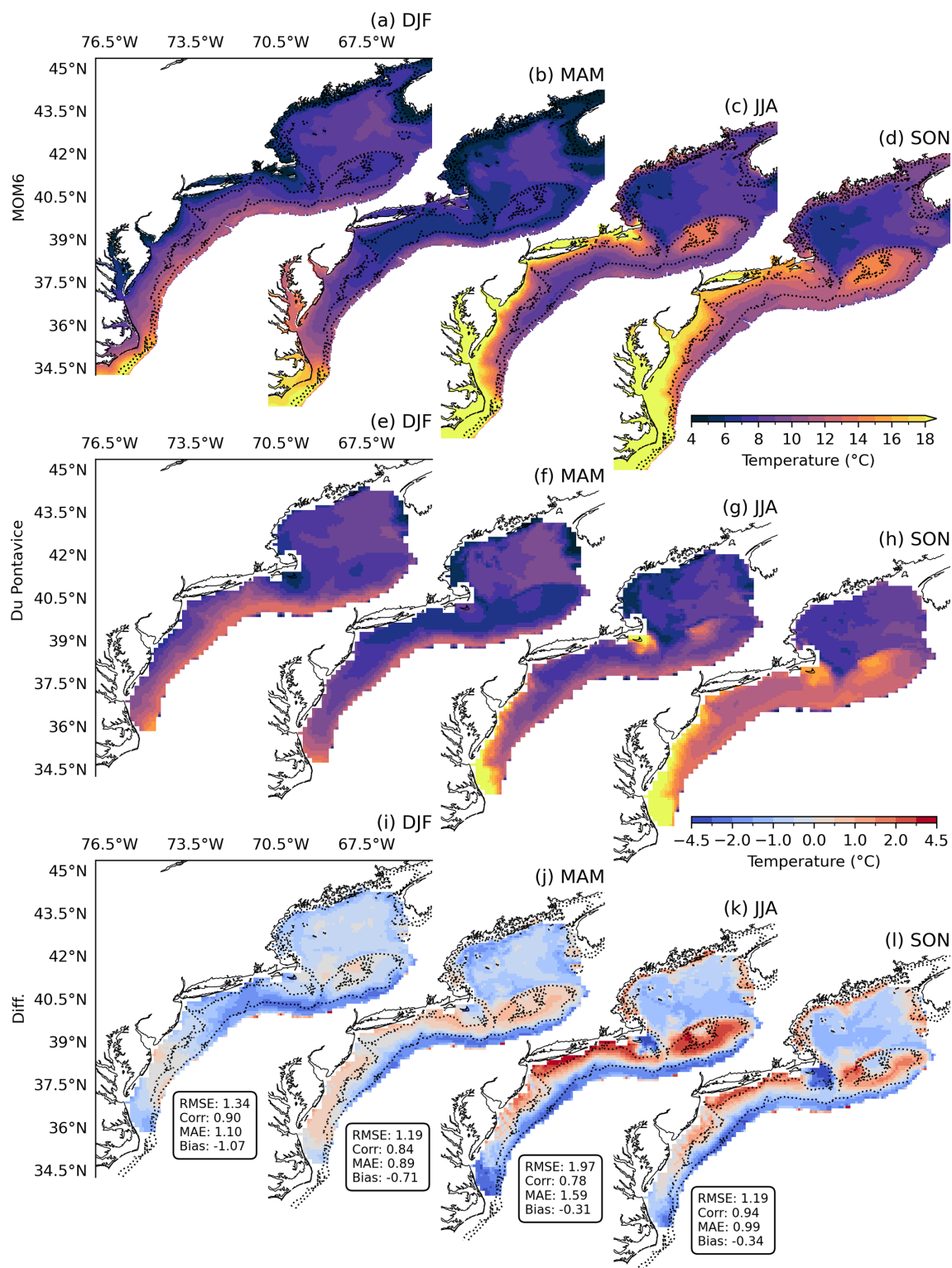
Figure 8. Seasonal averages of bottom temperature in MOM6 (a–d), Du Pontavice bottom temperature dataset (e–h), and their difference (MOM6 – duPontavice, i–l) considering the period between 1993 to 2019. Dotted lines correspond to the isobaths of 40 and 80 m. MOM6 results were upscaled to Du Pontavice’s resolution ( 1/12^\circ ) by binning corresponding areas and calculating averages.
