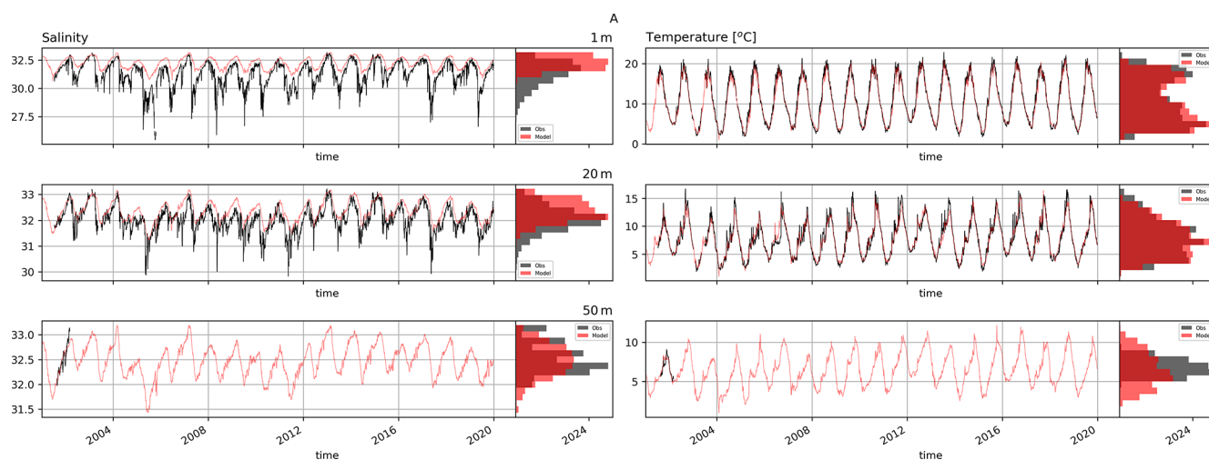
Figure A6. Time series of salinity in temperature of MOM6 (red) and NERACOOS mooring measurements (black) at buoy A.
