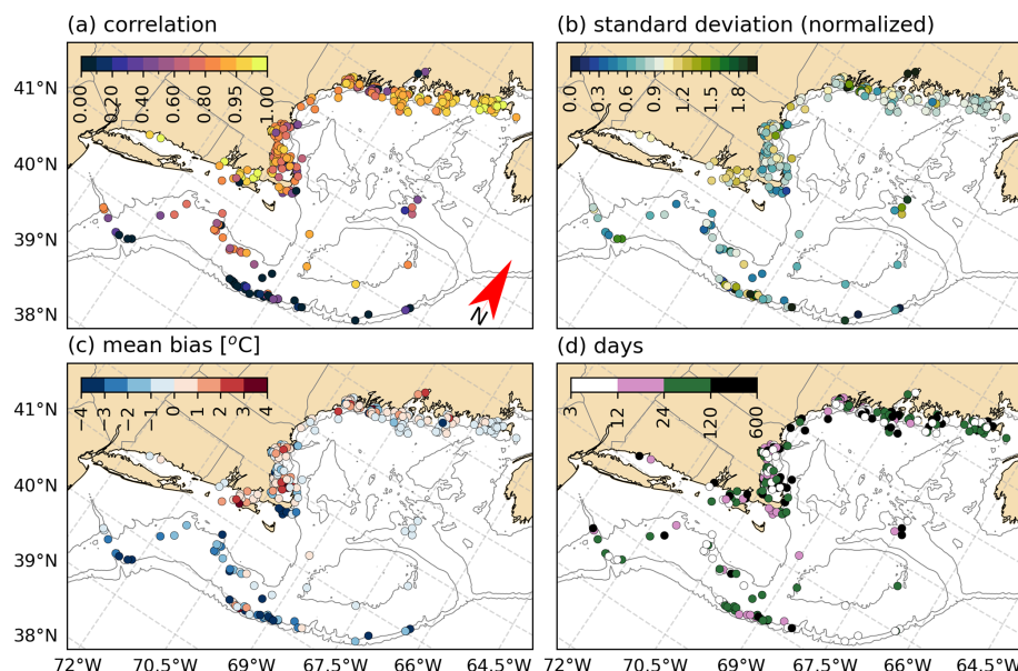
Figure 9. Daily averaged bottom temperature statistics between MOM6 results and eMOLT dataset corresponding to (a) correlation, (b) standard deviation, (c) mean bias and (d) number of days available (log scale). The contours represent depths of 60, 200, and 1000 m.
