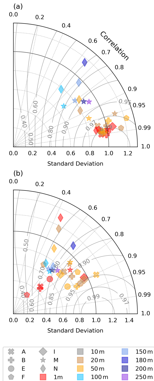
Figure 11. Taylor diagram evaluating MOM6 daily temperature (a) and salinity (b) performance against NERACOOS measurements. Gray shapes in the legend represent the mooring identification, while colors represent measurement depths. The standard deviation of the model results is normalized by the standard deviation of the observations. Curved contours represent isolines of skill score (Willmott, 1981).
