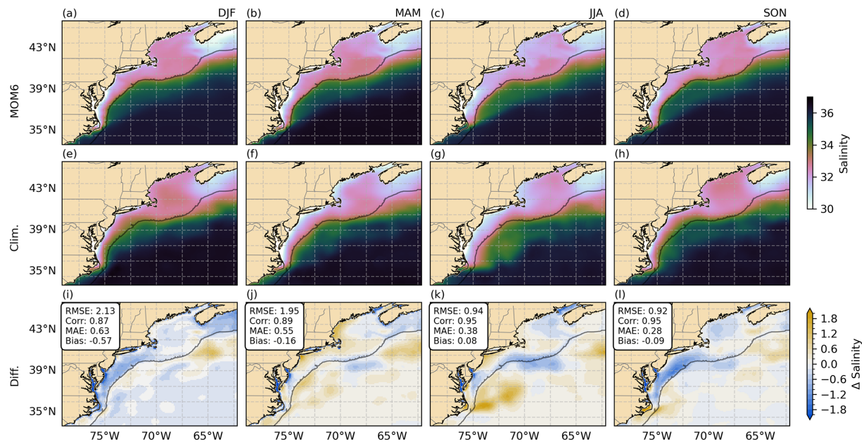
Figure 7. Seasonal averages of sea surface salinity from MOM6 (a–d) and NCEI regional climatologies (Clim., e–h) and seasonal differences (MOM6 – Clim., i–l). Black contour indicates the 400 m isobath, roughly representing the position of the shelf break. MOM6 results were upsampled to NCEI climatologies resolution ( 0.1^\circ ) by binning corresponding areas and calculating averages.
