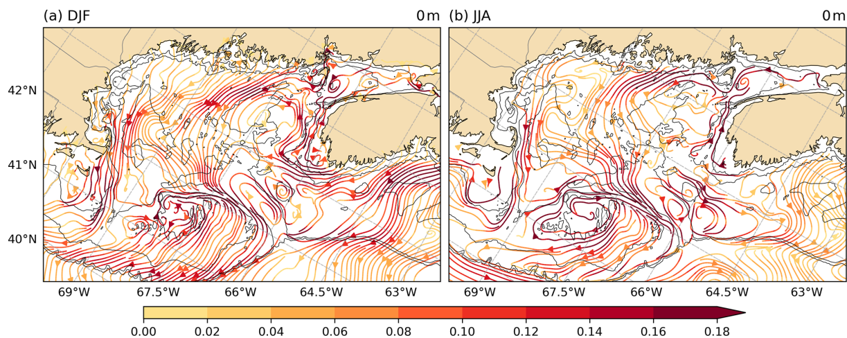
Figure 4. Winter (a) and summer (b) integral curves of the instantaneous MOM6 surface velocity field, computed via numerical integration of the tangent vector field.
