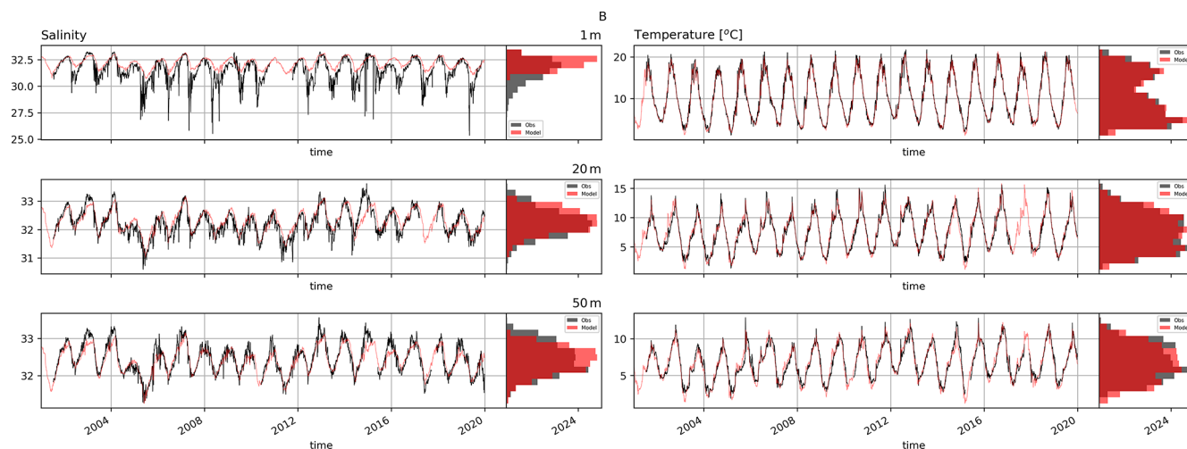
Figure A7. Time series of salinity in temperature of MOM6 (red) and NERACOOS mooring measurements (black) at buoy B.
