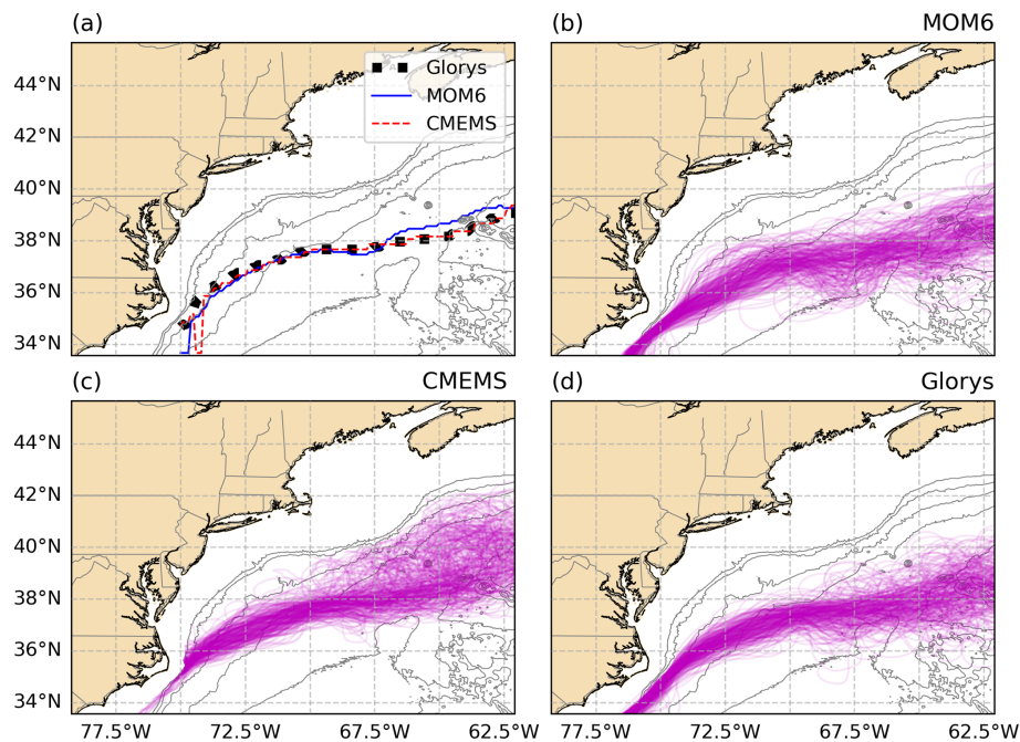
Figure 2. Path comparison of the Gulf Stream for the period between the years of 1993–1994 across MOM6, CMEMS satellite SSH L4 product and GLORYS. Position of the Gulf Stream based on the maximum standard deviation of SSH (a). In the remaining panels (b–d), magenta lines represent the 0 m contour of monthly SSH anomaly. Gray lines represent isobaths of 1000, 2000, 3000, 4000, and 5000 m
