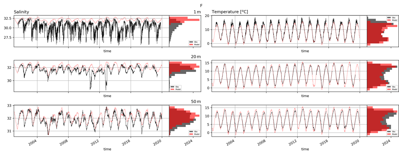
Figure A9. Time series of salinity in temperature of MOM6 (red) and NERACOOS mooring measurements (black) at buoy F.
