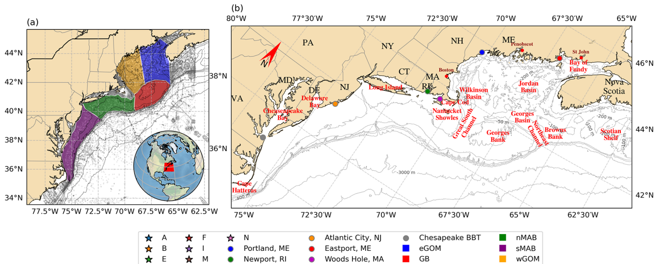
Figure 1. Model domain, Bathymetry, Observations (a), and locations references (b): Stars represent NERACOOS moorings, circles indicate CO-OPS tide gauges, and gray dots show high-resolution CTD data from the World Ocean Database. Colored shapes mark the locations of eastern Gulf of Maine (eGOM), western Gulf of Maine (wGOM), Georges Bank (GB), northern Mid-Atlantic Bight (nMAB), and southern Mid-Atlantic Bight (sMAB).
