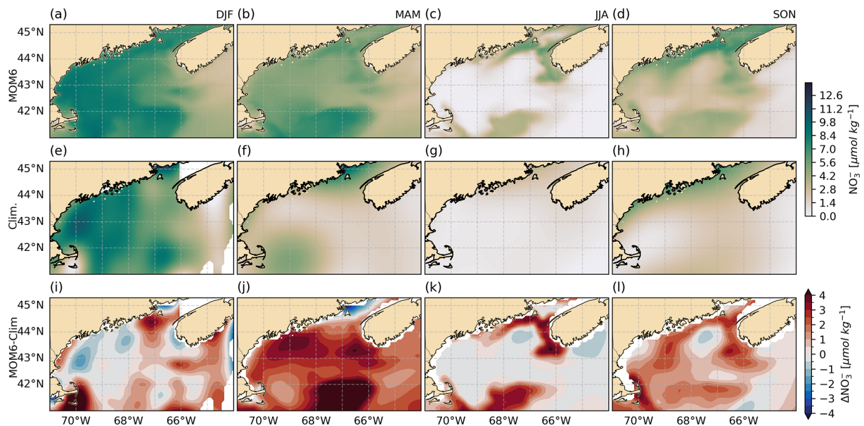
Figure 14. Seasonal surface distribution of nitrate in the Gulf of Maine region considering the climatology of surface concentrations from MOM6 (a–d), a seasonal climatology calculated from Rebeck’s dataset (e–h), and their difference (i–l) (MOM6 – Climatology). Columns represent seasons: DJF, MAM, JJA, SON.
