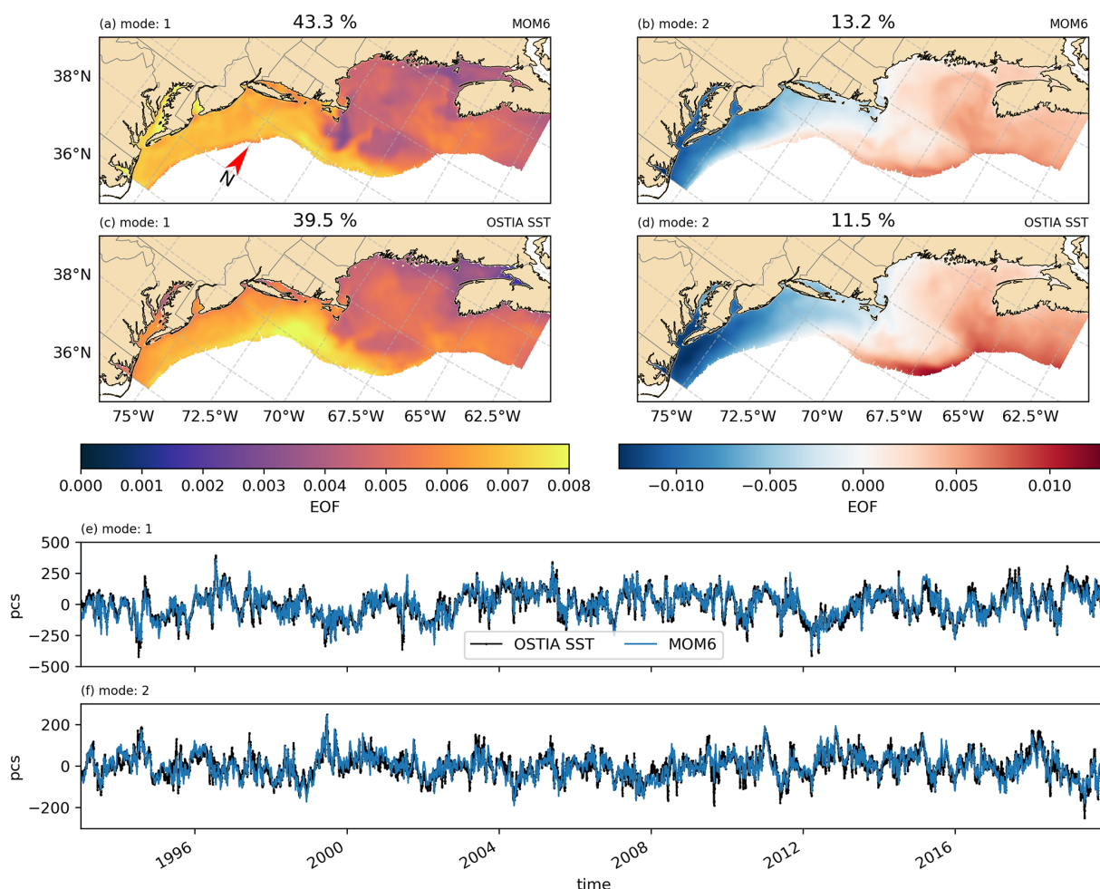
Figure 12. First (a, c, e) and second (b, d, f) modes of empirical orthogonal functions and principal component time series considering SST detrended daily anomalies of MOM6 (a, b) and OSTIA SST (c, d). For the first (second) mode of principal components correlation, normalized standard deviation, mean bias and mean absolute error are 0.94, 1.04, 0.4487, and 167.73 (0.88, 1.02, -0.08 , 27.74), respectively. The explained variance of MOM6 (OSTIA SST) first mode is 43.3 % (39.5 %), while the second mode has 13.2 % (11.5 %).
