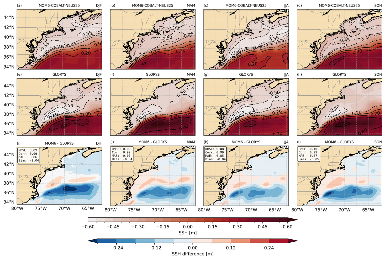
Figure 3. Seasonal averages of SSH considering MOM6-COBALT-NEUS25 (a–d), GLORYS (e–h) and their difference, MOM6-COBALT-NEUS25 – GLORYS (i–l). Black contours and filled contours represent SSH intervals.
