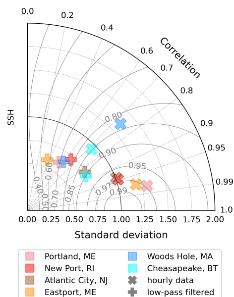
Figure 13. Taylor diagram of hourly SSH data at tide gauges at multiple coastal areas in the Gulf of Maine and Mid-Atlantic Bight alongside low-pass data with a cutoff period of 24 h (Lanczos filter). The standard deviation of the model results is normalized by the standard deviation of the observations. Curved contours represent isolines of skill score (Willmott, 1981).
