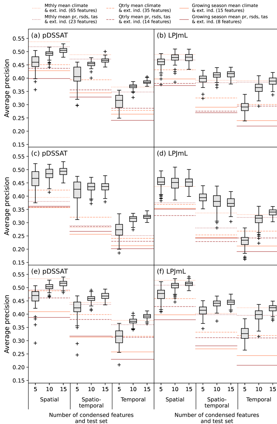
Figure A7. As in Fig. A6 but for average precision (higher is better).
