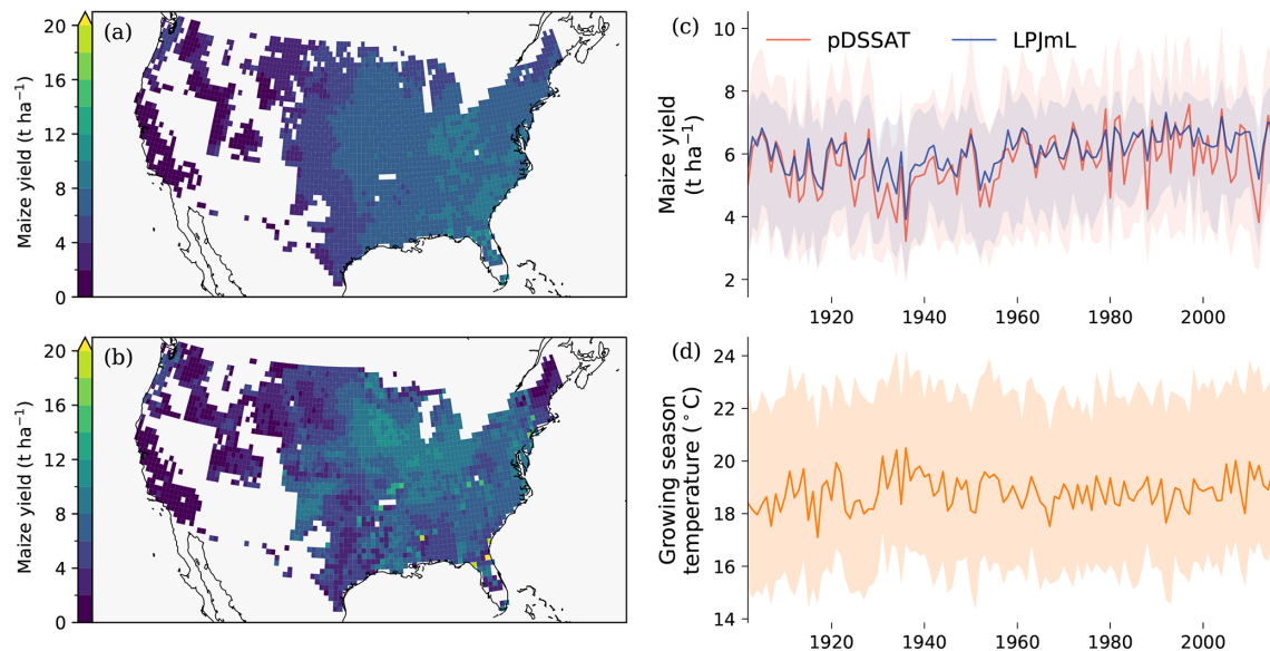
Figure 2. Overview of the rainfed maize yield simulations from both crop models. (a, b) Average yields over the entire time period studied, for LPJmL and pDSSAT respectively, for grid cells included in the dataset. (c) Distributions of yields from year to year, with darker lines denoting the median yield across all grid cells for each crop model, and shaded regions covering the interquartile ranges. (d) Distribution of annual growing season temperatures (here defined as the average daily mean temperature in the first 180 d after planting) in the corresponding climate forcing data.
