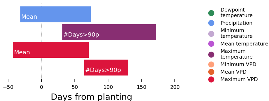
Figure 8. Four identified climate drivers of US county-level maize yield failure, for predominantly-rainfed counties, based on using 20 sampled time periods to generate 100 pools of candidate features, using ten-fold temporal cross-validation to select ten features from each pool, and condensing the resulting 1000 features.
