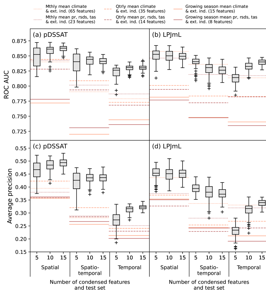
Figure 7. Comparison of the spatial, spatiotemporal and temporal test-set performance of Lasso models for pDSSAT (a, c) and LPJmL (b, d). Box plots show the scores for models using sets of five, ten or fifteen drivers using our proposed method, and horizontal lines denote the scores for the same models using baseline feature sets as predictors (made up of mean aggregate climate variables over the growing season or in monthly/quarterly intervals as well as five extreme indicators).
