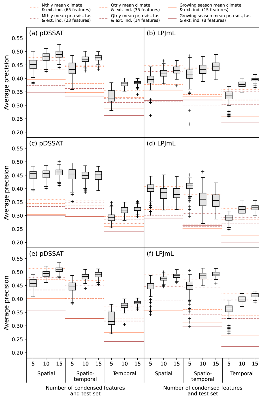
Figure B9. As Fig. A7, when yields are detrended.
