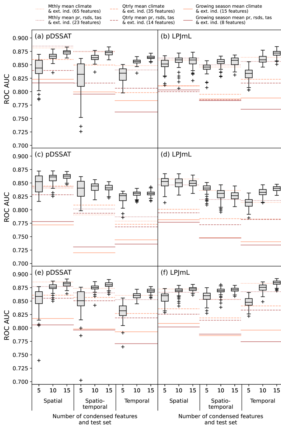
Figure A6. ROC AUC scores on test sets for models trained on training set, using feature sets derived from training set data (higher is better). (a, c, e) show scores for pDSSAT and (b, d, f) show LPJmL. (a, b) use LASSO logistic regression and include interaction terms; (c, d) use LASSO without interaction terms, (e, f) use extra trees.
