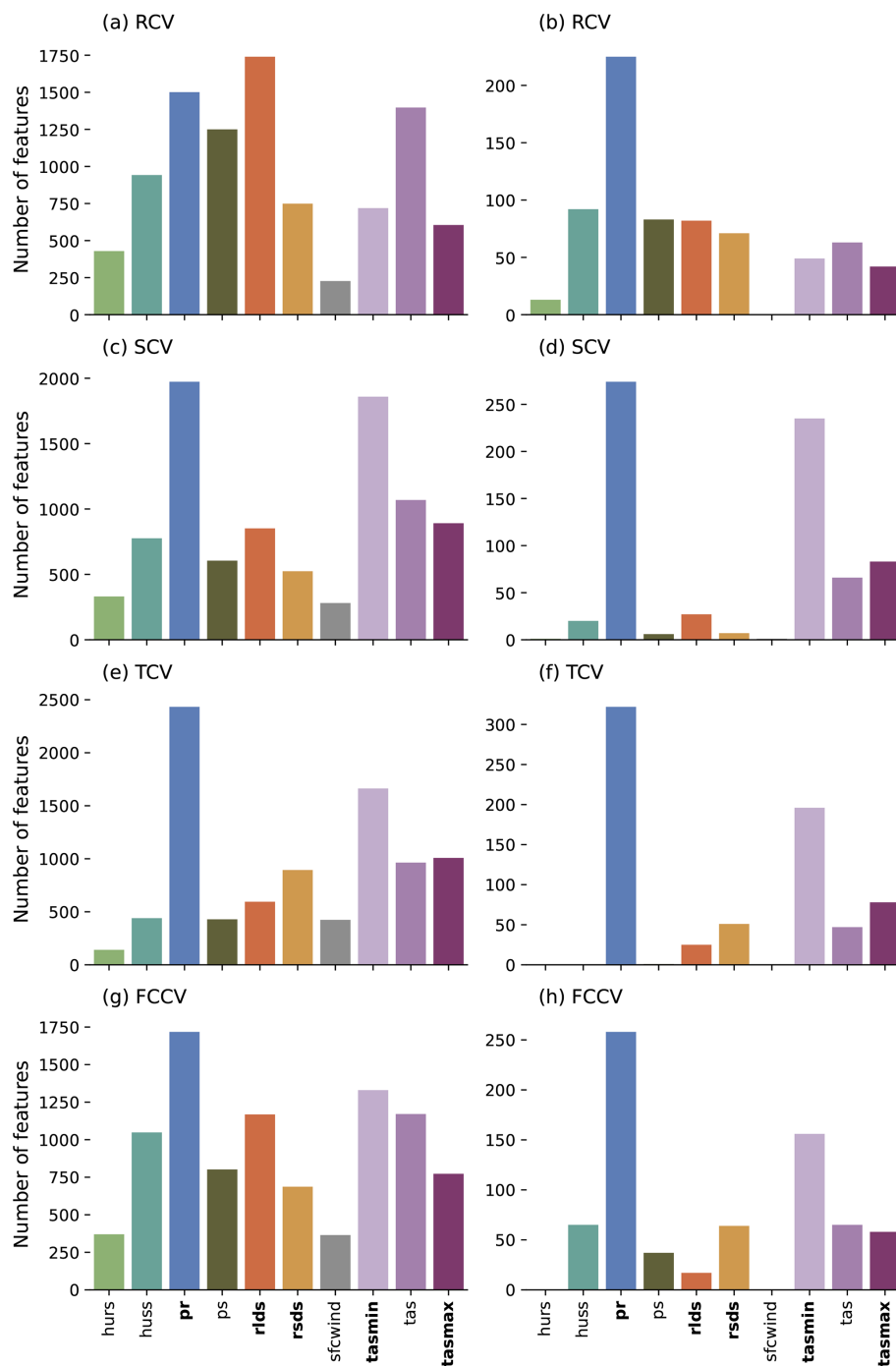
Figure D1. Climate variables used by features selected in Step 2 (a, c, e, g) and in drivers identified in Step 3 (b, d, f, h) for pDSSAT without detrending, depending on cross-validation strategy used to select features: random (RCV), spatial clusters (SCV), temporal (TCV) and feature-based clusters (FCCV). An exhaustive grid parameter sweep is performed (sampling 10, 20 or 30 time intervals in each pool; selecting 10, 20 or 30 features from each pool; and using 5, 10 or 15 cross-validation folds), using 20 pools per unique parameter combination, and sets of 5, 10 and 15 drivers are extracted. Features and drivers resulting from all parameter combinations are grouped by variable and counted.
