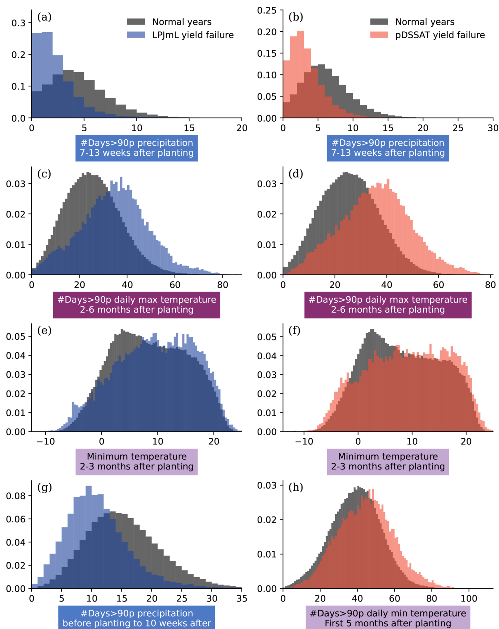
Figure 6. Distributions for normal and yield-failure years of some of the identified climate drivers of maize yield failure shown in Fig. 5, for LPJmL (a, c, e, g) and pDSSAT (b, d, f, h).
