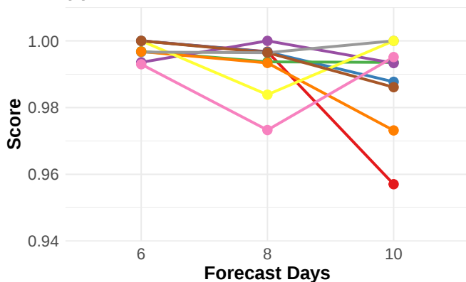
(a) PSS
