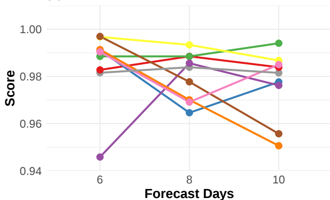
(e) PSS
