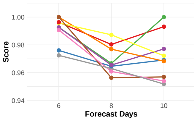
(c) PSS
