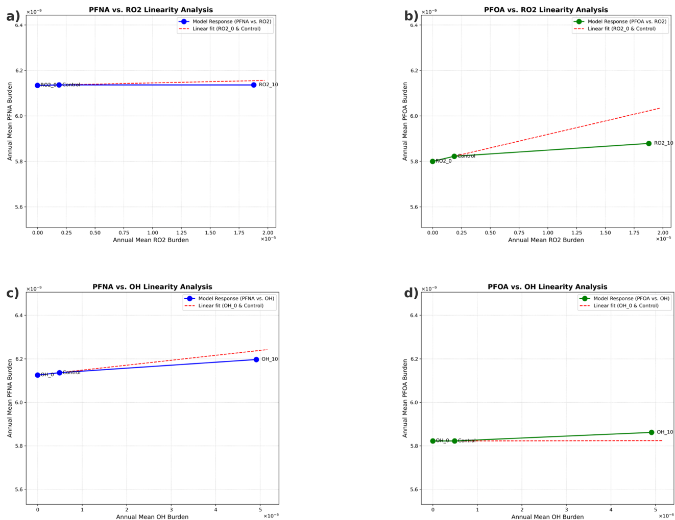
Figure E5. Linearity analysis of global annual mean burdens of PFNA and PFOA. Panels (a)–(b) show the response to RO 2 and (c)–(d) to OH. The model response (solid line) is compared against a linear fit (dashed red line) across three points: radical removal ( \times 0 ), base case (control), and a ten-fold increase ( \times 10 ). The deviation of the solid line from the dashed line represents the non-linear chemical feedback of the system.
