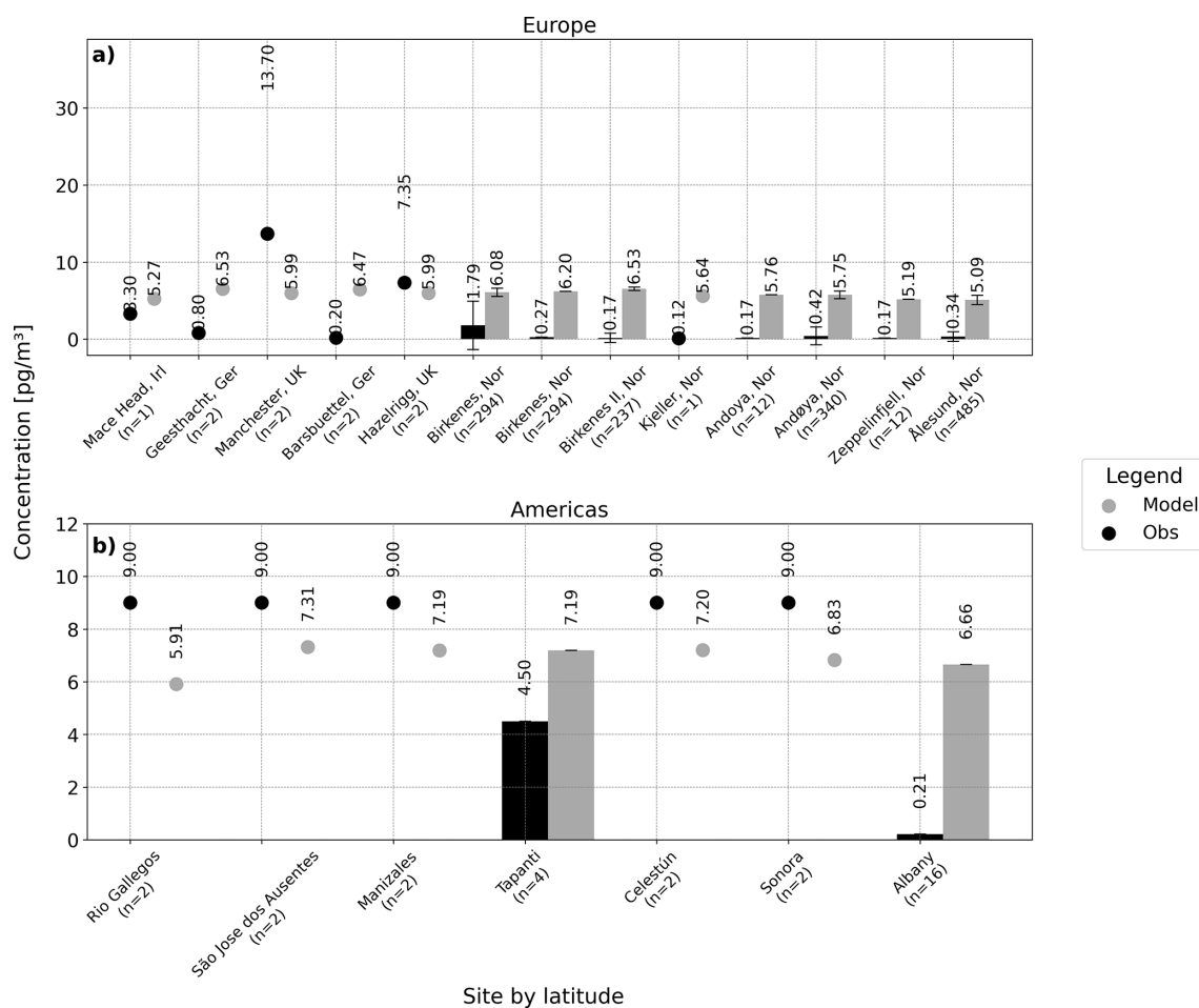
Figure 4. PFNA observed and simulated atmospheric concentrations [ \text{pg m}^{-3} ] in Europe and the Americas. Observed (black), Modeled (gray). Number of observations next to site.
