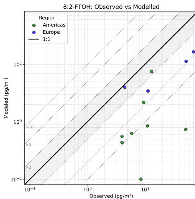
Figure D3. Comparison of observed versus modeled 8:2 FTOH concentrations ( \text{pg m}^{-3} ) by region on a log-log scale. The solid line represents 1, 1 agreement, with dotted lines indicating deviations by factors of 2, 5, and 10.
