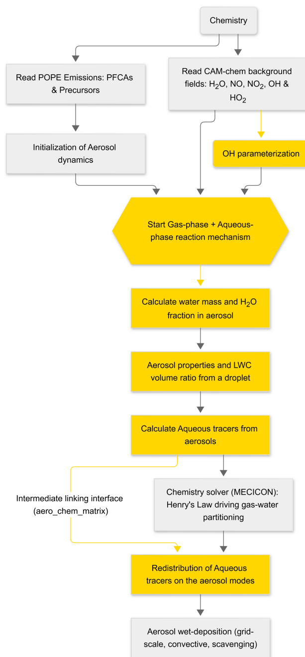
Figure 1. Flowchart showing the implemented chemistry processes for PFCA species and precursors in ICON-ART PRIEST. The parts marked in yellow correspond to the processes added to the complete chemistry module to extend ICON-ART.
