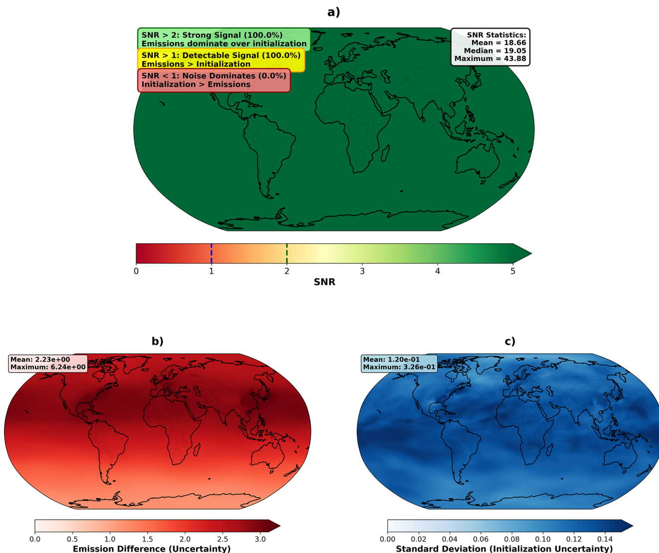
Figure E6. Signal to noise ratio analysis, emissions vs. initialization time (a) Signal to Noise Ratio (SNR): Emission sensitivity vs. initialization uncertainty. (b) Signal: Emission sensitivity, absolute value from differences of all UB initializations and LB initializations. (c) Noise: Internal variability, standard deviation from all the initializations.
