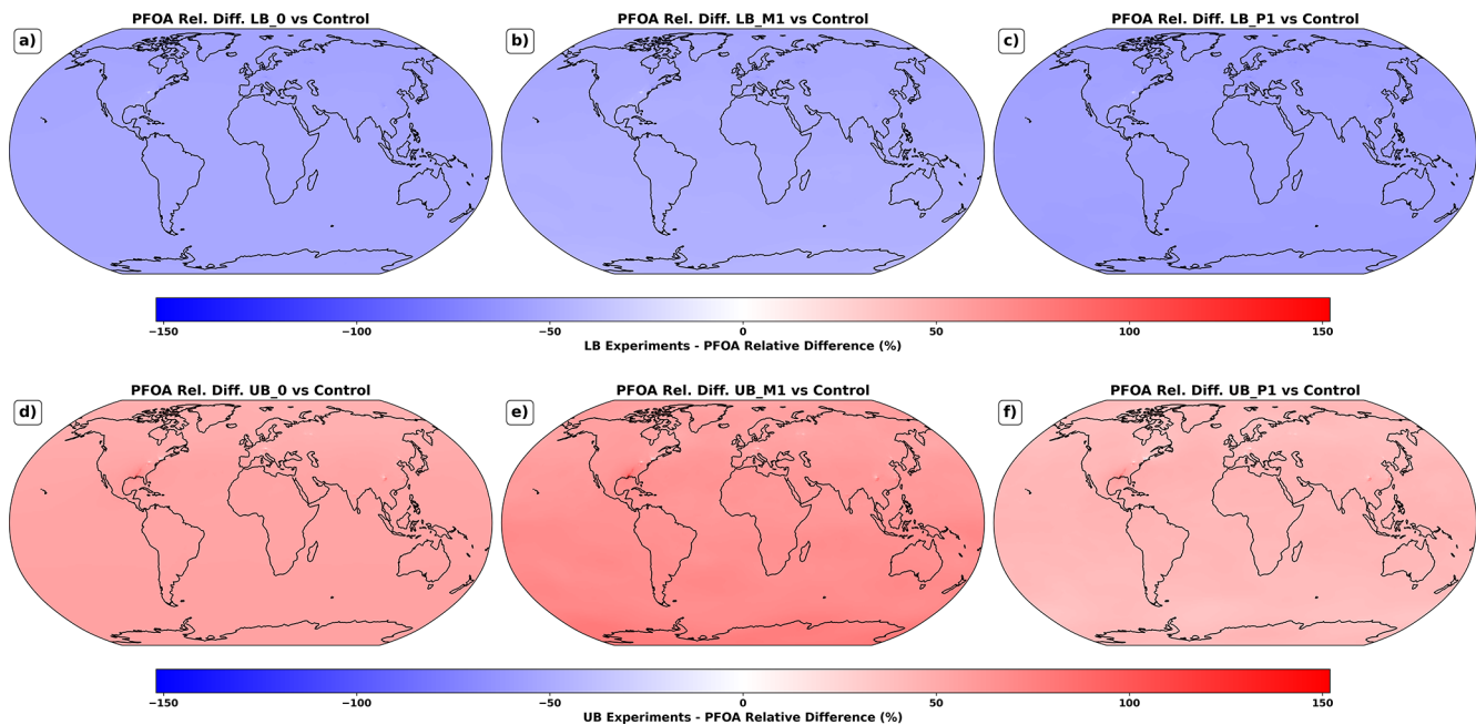
Figure E3. Relative mean differences PFOA from different initialization times. (a) LB 0 vs. Control, (b) LB M1 vs. Control, (c) LB P1 vs. Control, (d) UB 0 vs. Control, (e) UB M1 vs. Control, (f) UB P1 vs. Control.
