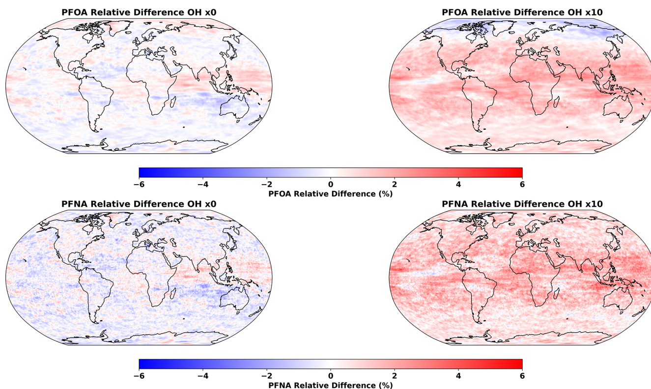
Figure E1. Relative Mean Differences (%) in annual mean atmospheric concentrations of PFOA (top) and PFNA (bottom). Panels show sensitivity experiments for OH × 0 (left) and OH × 10 (right) relative to the control simulation.
