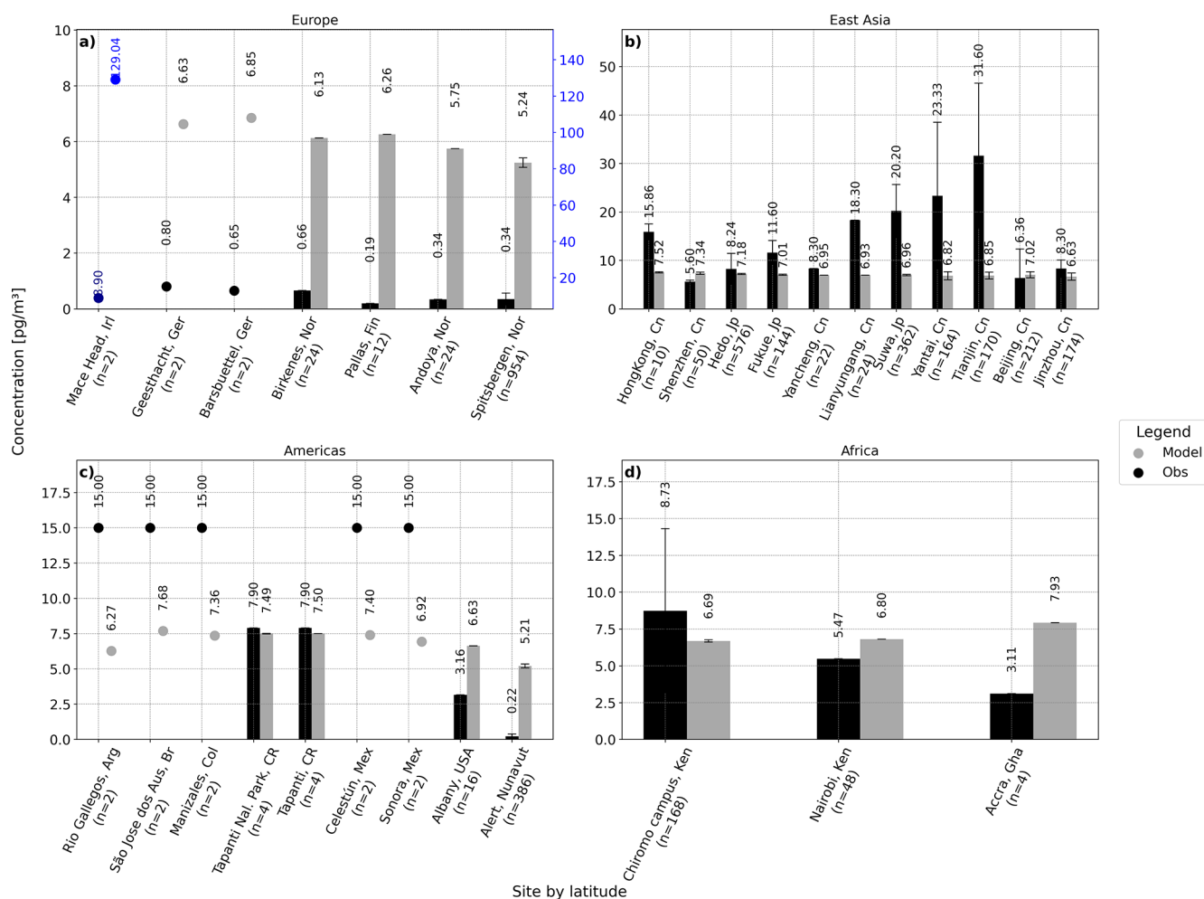
Figure 2. Observed and simulated atmospheric PFOA concentrations [ \text{pg m}^{-3} ] in (a) Europe, (b) East Asia, (c) Americas and (d) Africa. Observed (black), modeled (gray) and number of observations (down the site name). Panel (a) includes a secondary right-hand axis (blue) for the Mace Head site, due to its large magnitude values.
