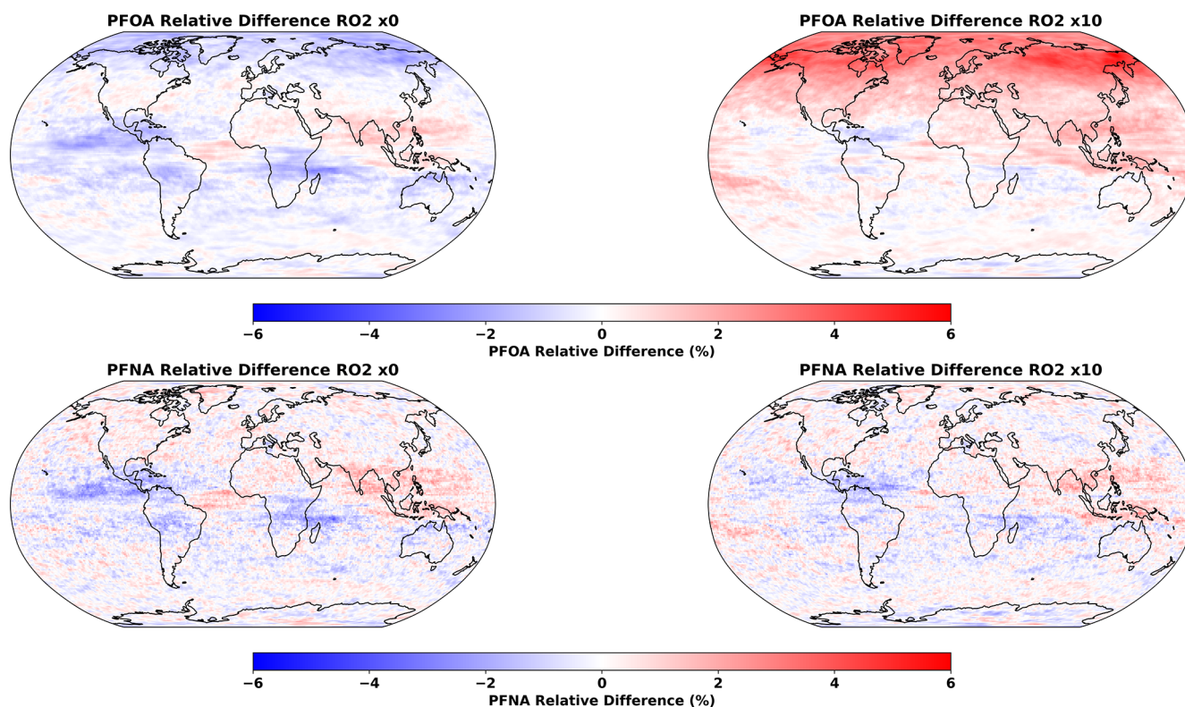
Figure E2. Relative Mean Differences (%) in annual mean atmospheric concentrations of PFOA (top) and PFNA (bottom). Panels show sensitivity experiments for RO 2 × 0 (left) and RO 2 × 10 (right) relative to the control simulation.
