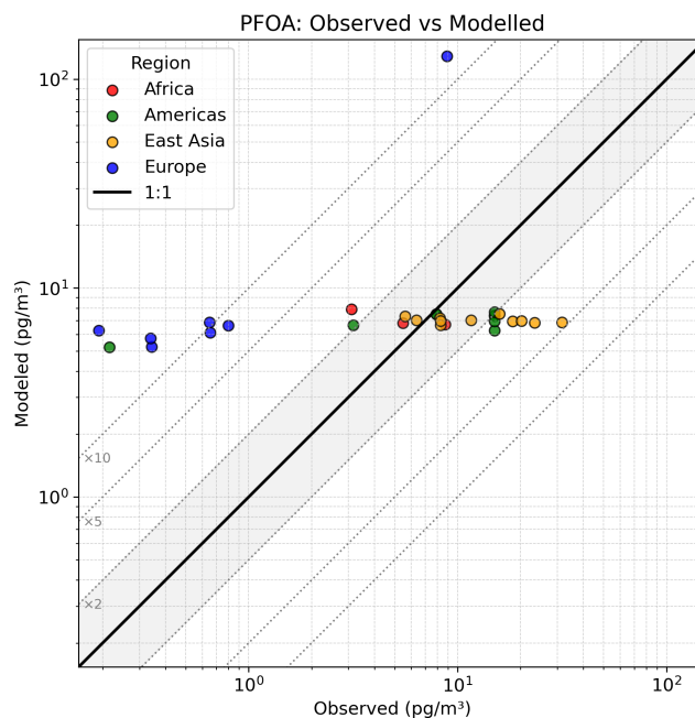
Figure D1. Comparison of observed versus modeled PFOA concentrations ( \text{pg m}^{-3} ) by region on a log-log scale. The solid line represents 1 : 1 agreement, with dotted lines indicating deviations by factors of 2, 5, and 10.
