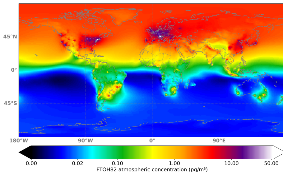
Figure 8. 8 : 2 FTOH mean atmospheric concentration over the period 2005–2019.
