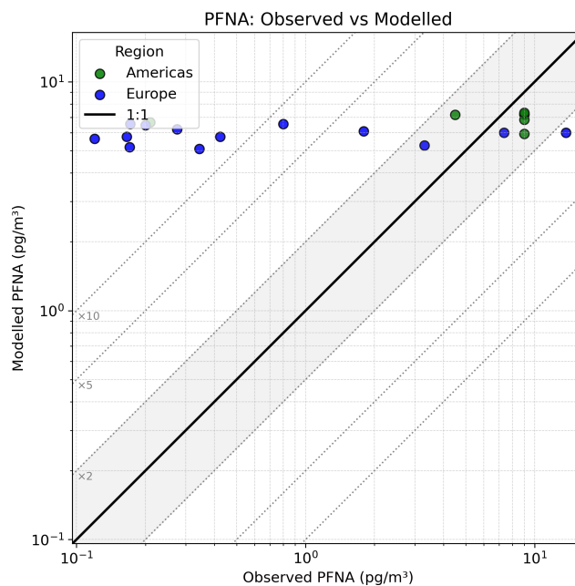
Figure D2. Comparison of observed versus modeled PFNA concentrations ( \text{pg m}^{-3} ) by region on a log-log scale. The solid line represents 1 : 1 agreement, with dotted lines indicating deviations by factors of 2, 5, and 10.
