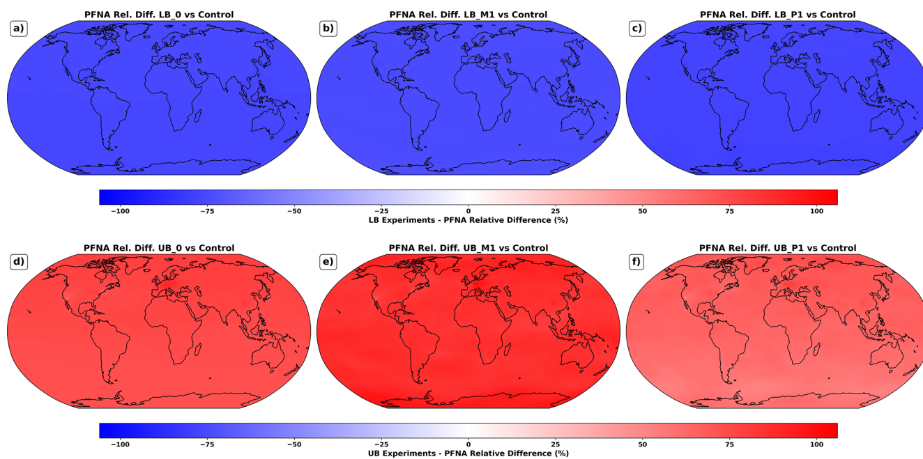
Figure E4. Relative mean differences PFNA from different initialization times. (a) LB 0 vs. Control, (b) LB M1 vs. Control, (c) LB P1 vs. Control, (d) UB 0 vs. Control, (e) UB M1 vs. Control, (f) UB P1 vs. Control.
