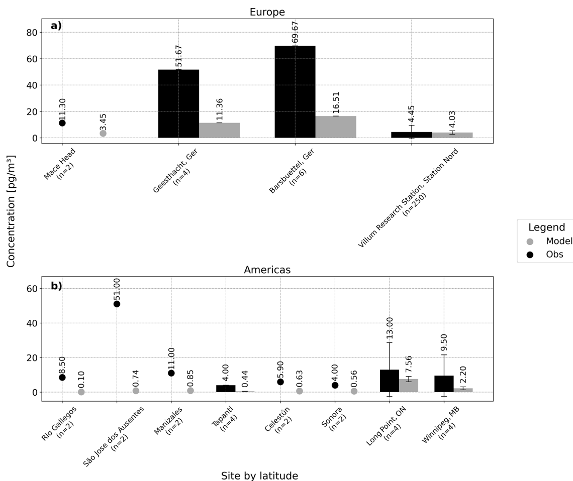
Figure 3. Observed and simulated atmospheric FTOH concentrations [ \text{pg m}^{-3} ] in Europe and the Americas. Observed (black), modeled (gray) and number of observations.
