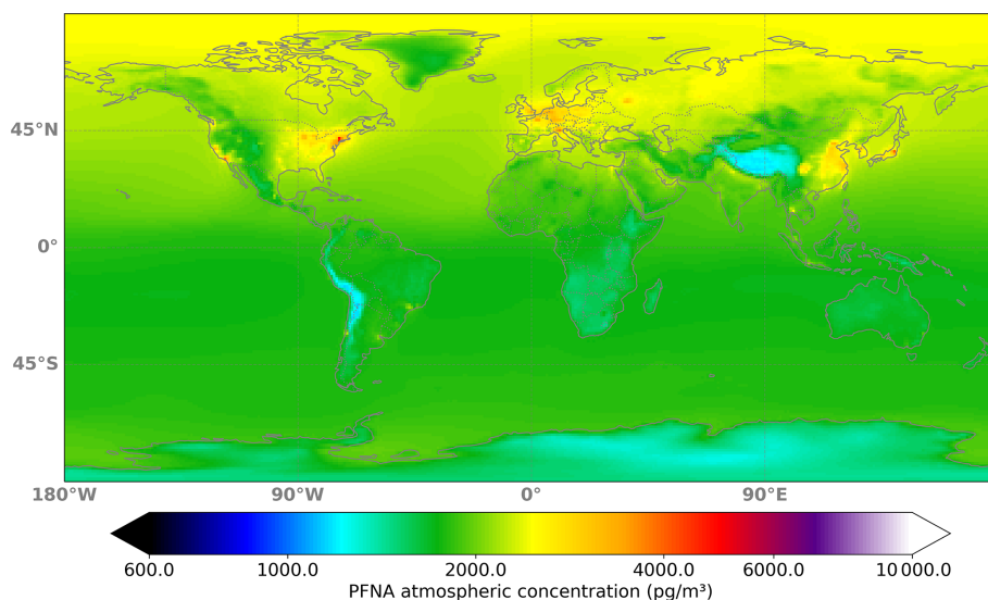
Figure 9. PFNA mean atmospheric concentration over the period 2005–2019.
