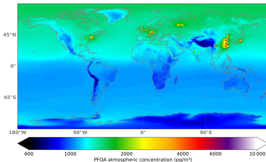
Figure 7. PFOA mean atmospheric concentration over the period 2005–2019.
