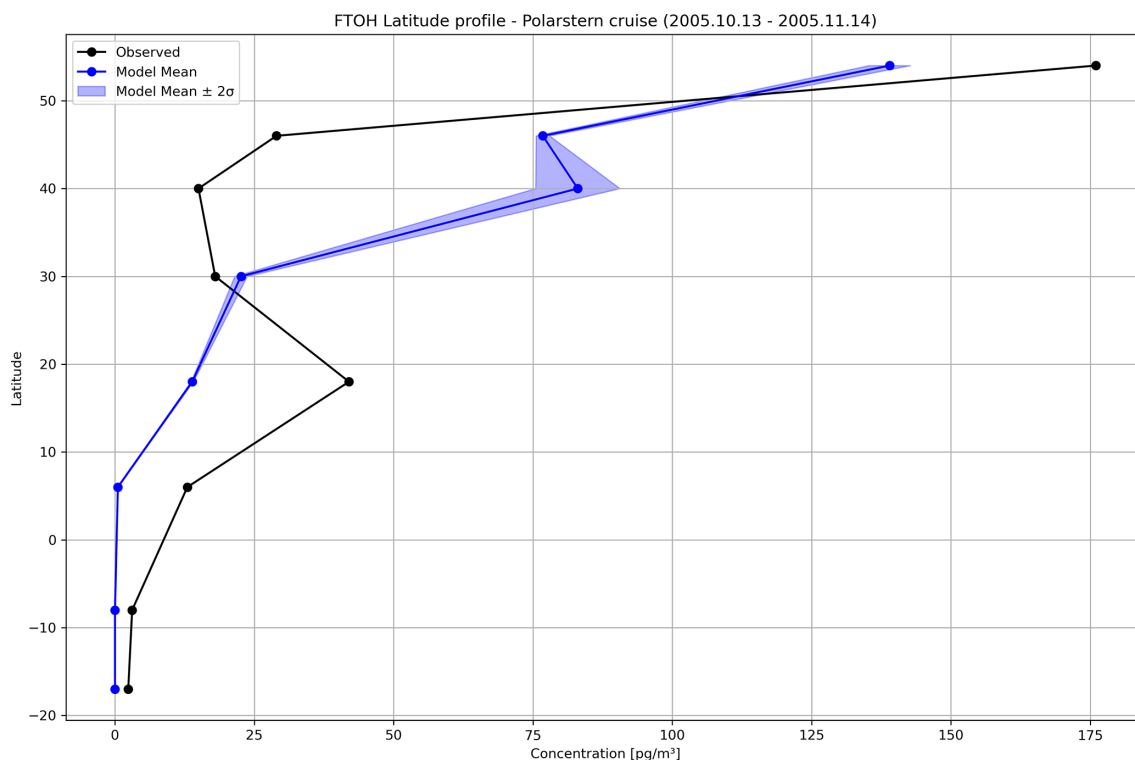
Figure 6. 8 : 2 FTOH latitudinal profile of atmospheric concentrations [ \text{pg m}^{-3} ]. Observed data (black) vs. Model (blue line). The shaded blue area indicates the model variability, defined as \pm 2 standard deviations calculated over the sampling period.
