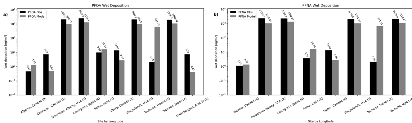
Figure 5. PFOA and PFNA wet deposition over different locations [ \text{ng m}^{-2} ]. Observed (black), Modeled (gray). Number of observations next to site.
