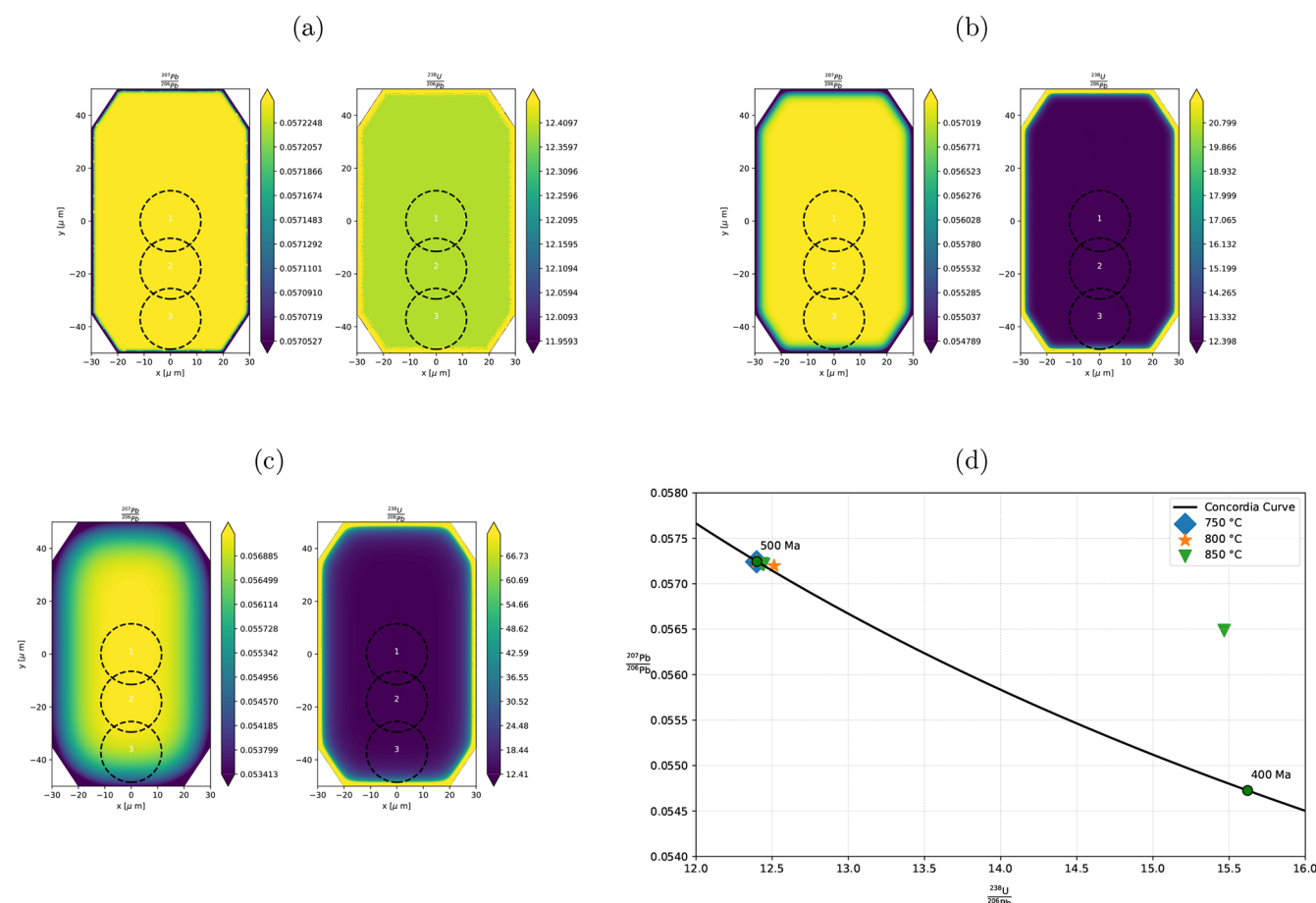
Figure 5. Diffusion-decay and diffusion-ingrowth test results in a zircon mesh geometry for a cell size of 0.01 and degree of 2 for uranium and lead. U–Pb isotope profiles after 500 Myr at (a) 750 °C, (b) 800 °C, (c) 850 °C. (d) Effect of sample location on age data. Discordance increases closest to the rims and at elevated temperatures for longer.
