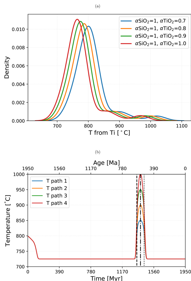
Figure 8. (a) Kernel density estimate (KDE) plot showing the bulk of zircons record a temperature of \sim 800 °C at formation based on the Ti-in-zircon thermometer. (b) Range of temperature-time paths tested for the Trivandrum block based on Ti-in-zircon thermometry and analytical data. Dotted lines represent the estimated start (600 Ma), peak (555 Ma) and end (520 Ma) of UHT metamorphism.
