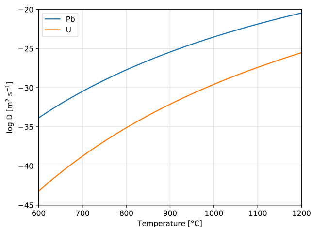
Figure 1. Diffusion coefficients for uranium (U) and lead (Pb) from values in Table 1 and Eq. (3) over a temperature range of 600 to 1200 °C.
