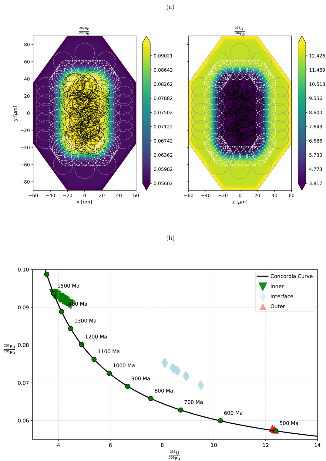
Figure 7. Effects of secondary zircon growth on U–Pb ratios and age based on sample location. (a) Dual growth zircon sample spot locations. (b) Tera-Wasserburg plot from sample spots.
