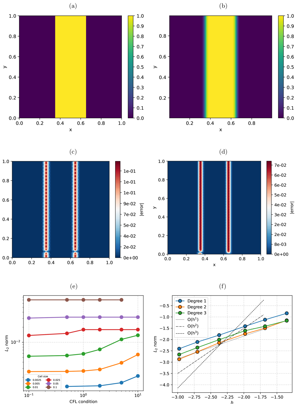
Figure 3. Diffusion convergence order from rectangular pulse benchmark. (a) Initial distribution of unknown at t = 0 . (b) Final distribution of unknown at t = 1 \times 10^{-4} . L2-norm when cell size is (c) 0.02 and (d) 0.01. (e) shows the L2-norm based on cell size and factor of CFL condition. (f) Shows the convergence of the solver.
