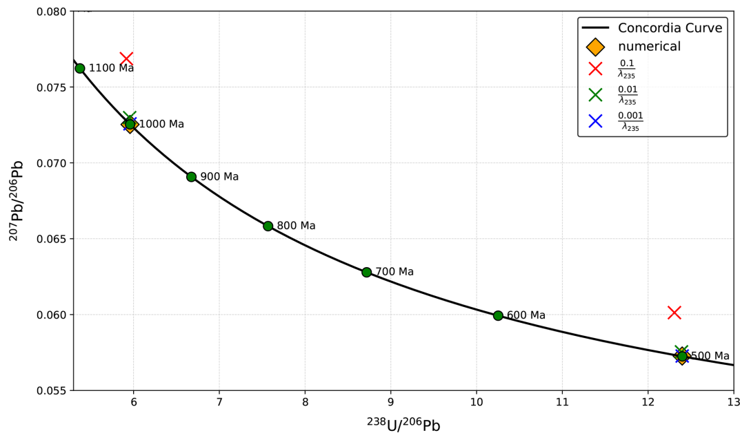
Figure 2. Tera-Wasserburg plot of \frac{^{238}\text{U}}{^{206}\text{Pb}} against \frac{^{207}\text{Pb}}{^{206}\text{Pb}} showing the concordia line (solid black line) 100 Ma increments between 1000 and 500 Ma (green dots) and results of models at 1000 and 500 Ma (various symbols) solving for the decay and ingrowth only plot on the concordia line based on different timesteps when including the decay and ingrowth as a source term (Eqs. 1a and 1b), or calculating it numerically (Eqs. 4 and 5).
