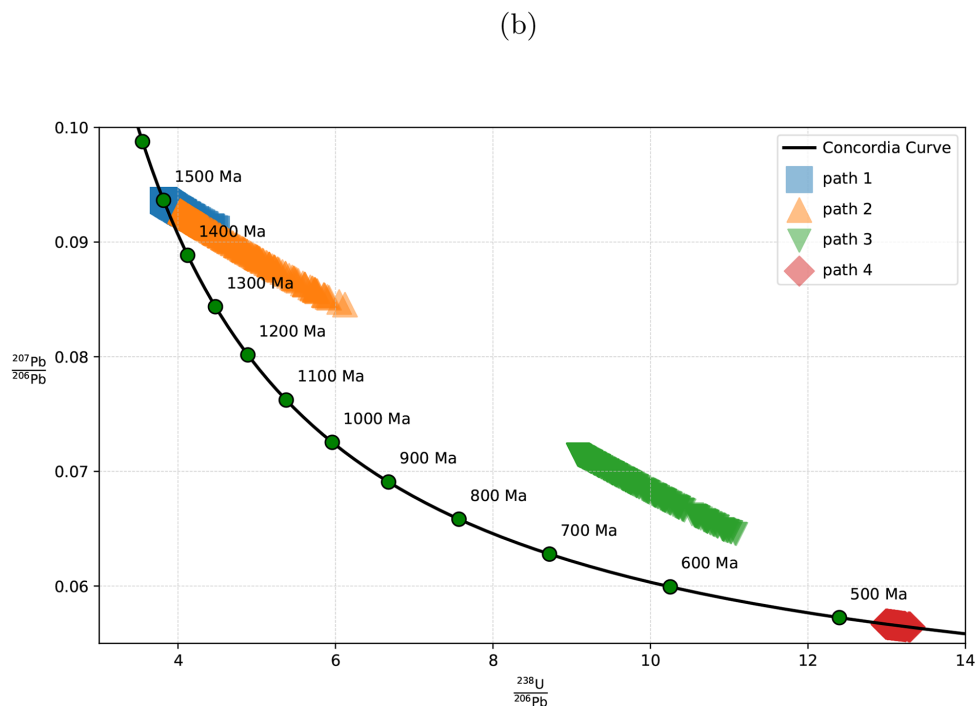
Figure 6. (a) Different temperature–time (Tt) paths tested. (b) Effects of different temperature–time paths on U–Pb ratios and ages based on sample location. Spot locations are presented in Fig. S1.
