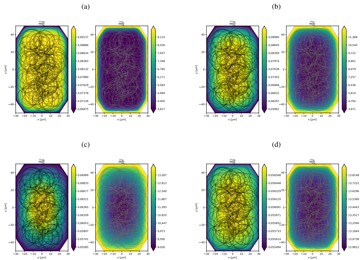
Figure S1. Plots of zircons after the temperature-time path tests showing the spot locations. a) T profile 1, b) T profile 2, c) T profile 3, d) T profile 4.
