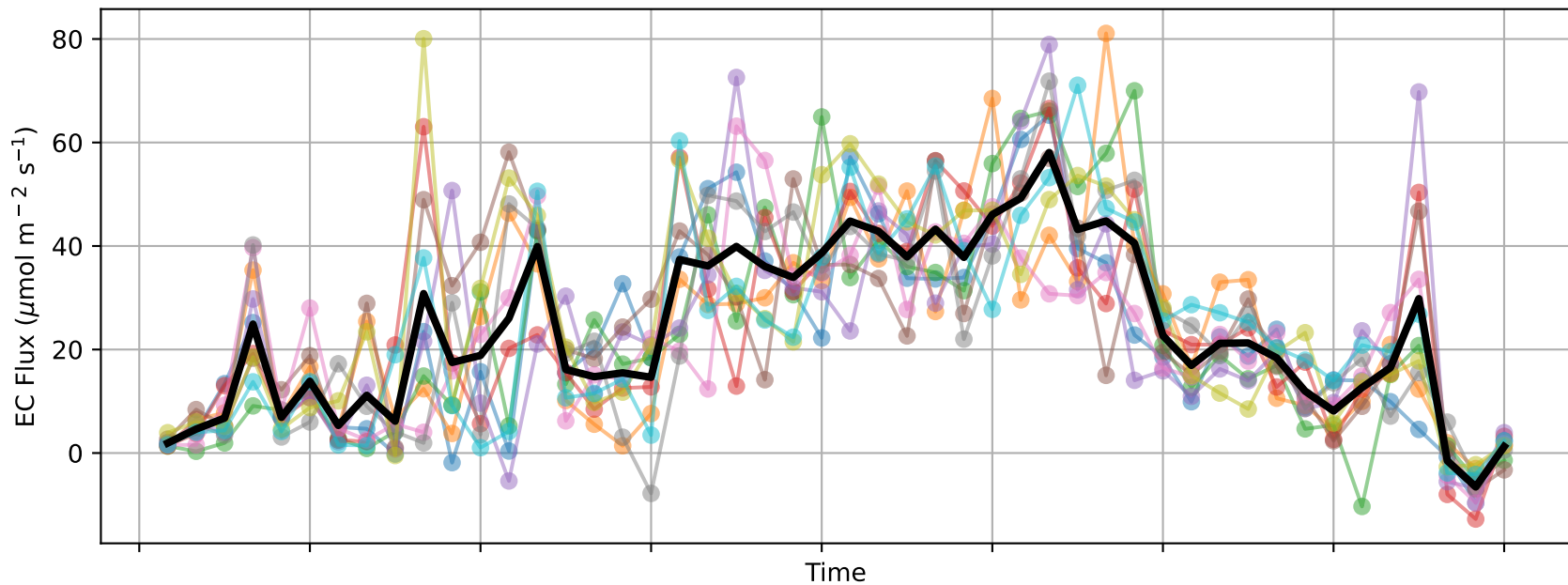
2h Rolling Mean of EC Flux for All Ensemble Members
