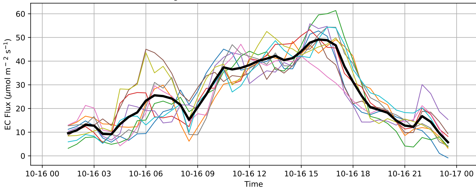
2h Rolling Mean of EC Flux for All Ensemble Members
