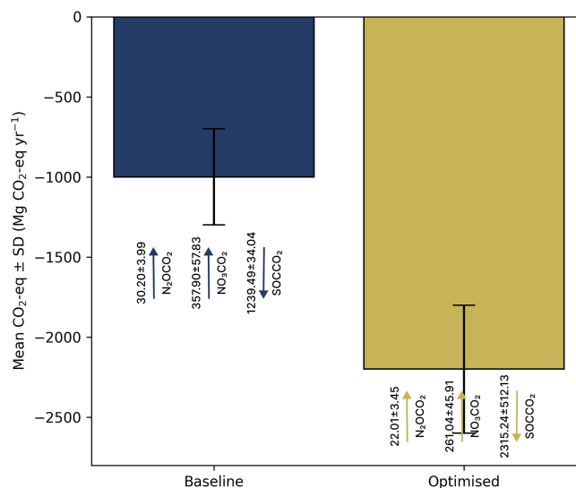
Figure 7. Soil-net GHG balance ( \text{Mg CO}_2\text{-eq yr}^{-1} ) under baseline and optimised management scenarios, averaged over the 10 year period 2011–2020; negative values indicate greater net climate-mitigation potential.
