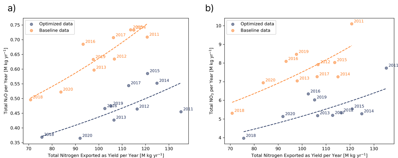
Figure 8. Total nitrogen exported as yield per year compared with (a) total \text{N}_2\text{O} emissions per year and (b) total \text{NO}_3^- leaching per year for baseline and optimised management.
