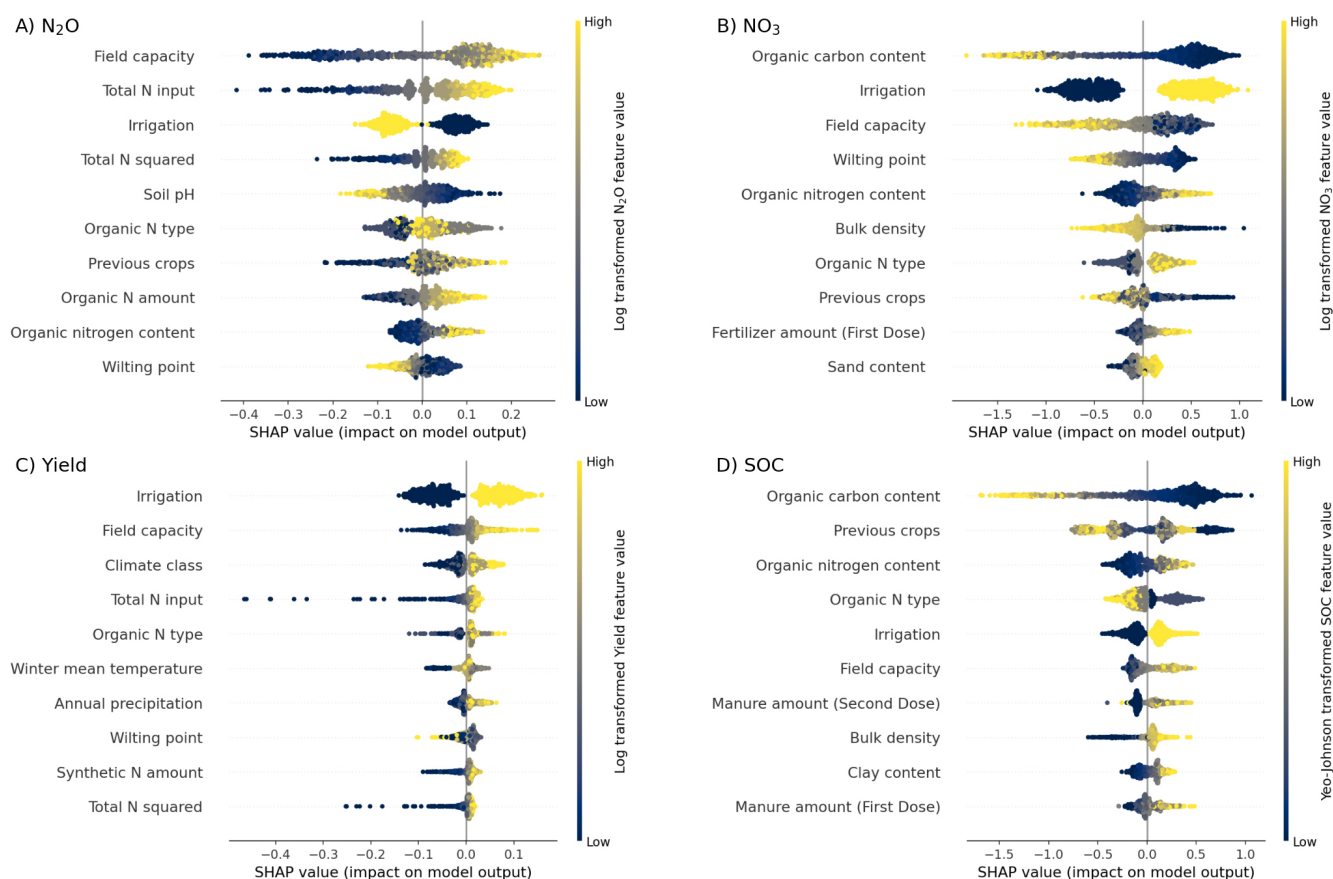
Figure 4. SHapley Additive exPlanations (SHAP) values of the four predicted variables ( \text{N}_2\text{O} , \text{NO}_3^- , Crop Yield and SOC). The vertical position of a feature reflects its overall importance, while the horizontal spread and colour show the direction and strength of its effect across all observations.
