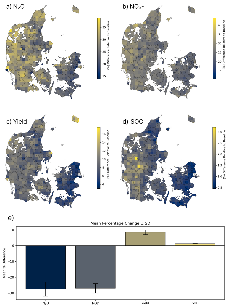
Figure 5. Panels (a)–(d) show the percentage difference between optimised management and the baseline scenario over the 10 year period from 2011–2020, aggregated to a 10 km \times 10 km grid, with decreases shown for N_2O emissions and NO_3^- leaching and increases shown for yield and soil organic carbon. Panel (e) presents the corresponding mean percentage change at the national scale.
