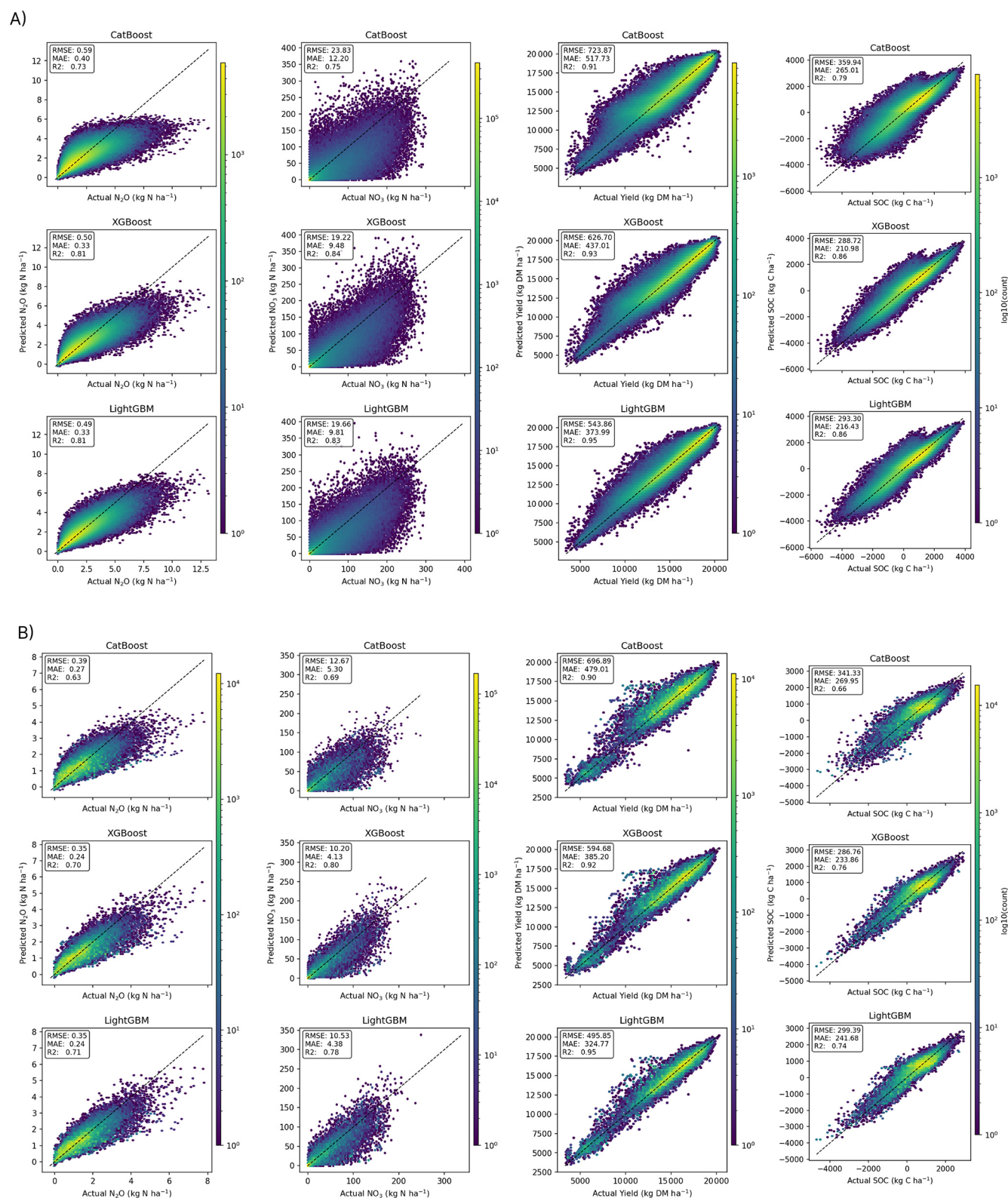
Figure 2. Performance metrics for CatBoost, XGBoost, and LightGBM across the four predicted variables (N 2 O, NO 3 - , SOC, and yield). Panel (A) shows RMSE, MAE, and R 2 in the possibility space, and (B) shows the corresponding metrics in the actual space.
