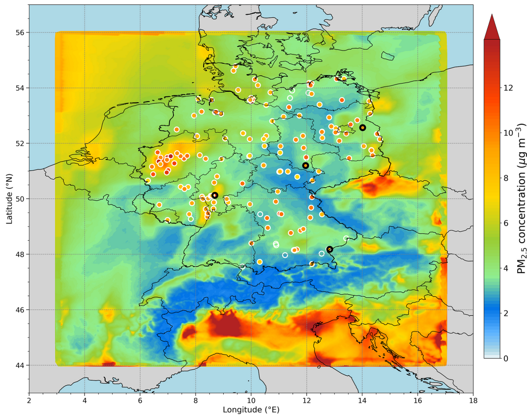
Figure 2. \text{PM}_{2.5} surface concentrations averaged over 3 to 11 March 2019 including contributions from carbonaceous aerosol (CA), sulfuric aerosol (SU), mineral dust (DU), and sea salt (SS) as computed by ICON-HAM-lite. Observations from the EEA air quality monitoring network are overlaid as circles, with black markers indicating the stations included in the time-series analysis in Fig. 3.
