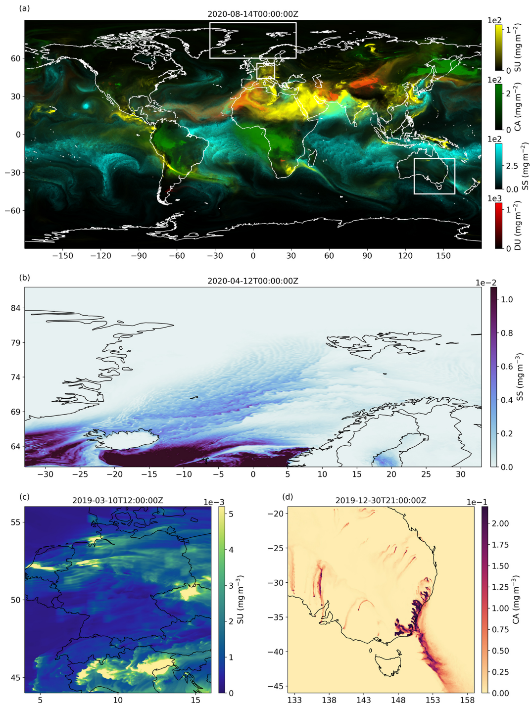
Figure 1. Scenes from a global simulation at a resolution of 5 km by Weiss et al. (2025) (a) and from the three regional simulations presented here at a resolution of 2.5 km (b–d). Panel (a) shows column burdens of dust (DU), sea salt aerosol (SS), carbonaceous aerosol (CA), and sulfuric aerosol (SU) as well as the boundaries of the three regional simulations. The panels below show snapshot surface concentrations for individual examples of (b) sea salt (SS) over the Arctic, (c) sulfuric aerosol (SU) over Germany, and (d) carbonaceous aerosol (CA) over Australia.
