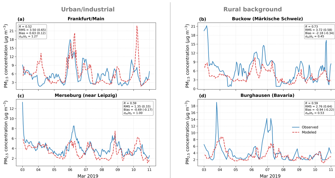
Figure 3. Hourly time series of observed and modeled PM_{2.5} surface concentrations at the urban/industrial sites (a) Frankfurt/Main and (c) Merseburg near Leipzig as well as the rural background sites (b) Buckow in the Märkische Schweiz and (d) Burghausen in Bavaria from 3 to 11 March 2019 (See the map in Fig. 2 for their geographic locations.). The observations are from the EEA air quality monitoring network. The model data are taken from ICON-HAM-lite simulations and include mass contributions from carbonaceous aerosol, sulfate, dust, and sea salt. For each panel the correlation coefficient R , the root mean square error RMS (normalized RMS in parenthesis), the absolute bias (normalized bias), and the ratio between simulated and observed standard deviation ( \sigma_m/\sigma_o ) are given.
