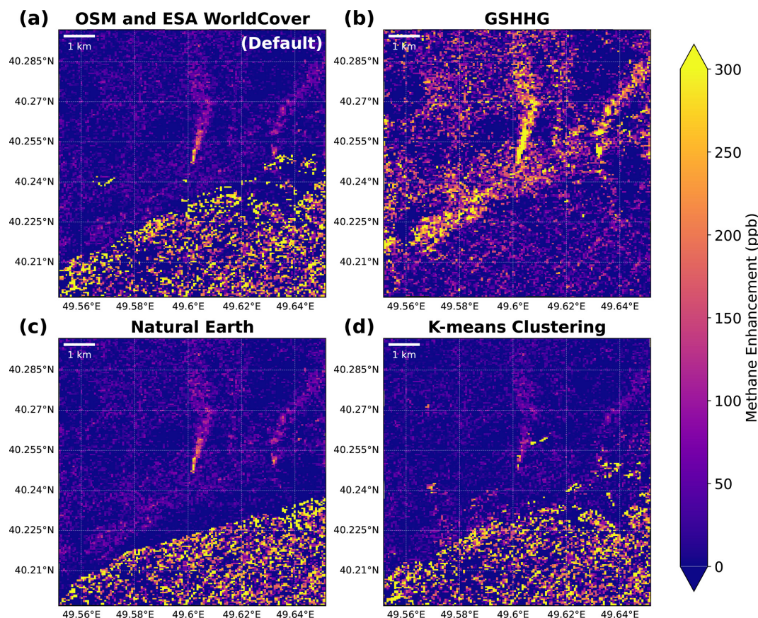
Figure 3. Retrieved methane enhancements from the EMIT observation over Azerbaijan on 21 April 2024, based on matched filter analysis applied to each pixel cluster as defined in Fig. 2.
