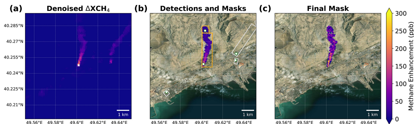
Figure 5. Plume mask creation process for the western plume from Fig. 3a. (a) The denoised methane enhancement ( \Delta X_{\text{CH}_4} ) field obtained by applying the Chambolle total variation (TV) denoising filter to \Delta X_{\text{CH}_4} within the 1300–2500 nm window. The white star marks the manually identified source location for the western plume. (b) Initial candidate masks derived from the watershed algorithm. White dots indicate high- \Delta X_{\text{CH}_4} locations, and colored rectangles represent the minimum rotated rectangles (oriented bounding boxes) for each mask. Orange rectangles denote masks with azimuth differences less than 30^\circ relative to the reference mask (containing the source marker of the western source) and are merged into a single plume. The gray rectangles are candidates excluded by the azimuth criterion. (c) The final \Delta X_{\text{CH}_4} plume mask for the western emission source after merging. Background imagery source: Esri|Powered by Esri.
