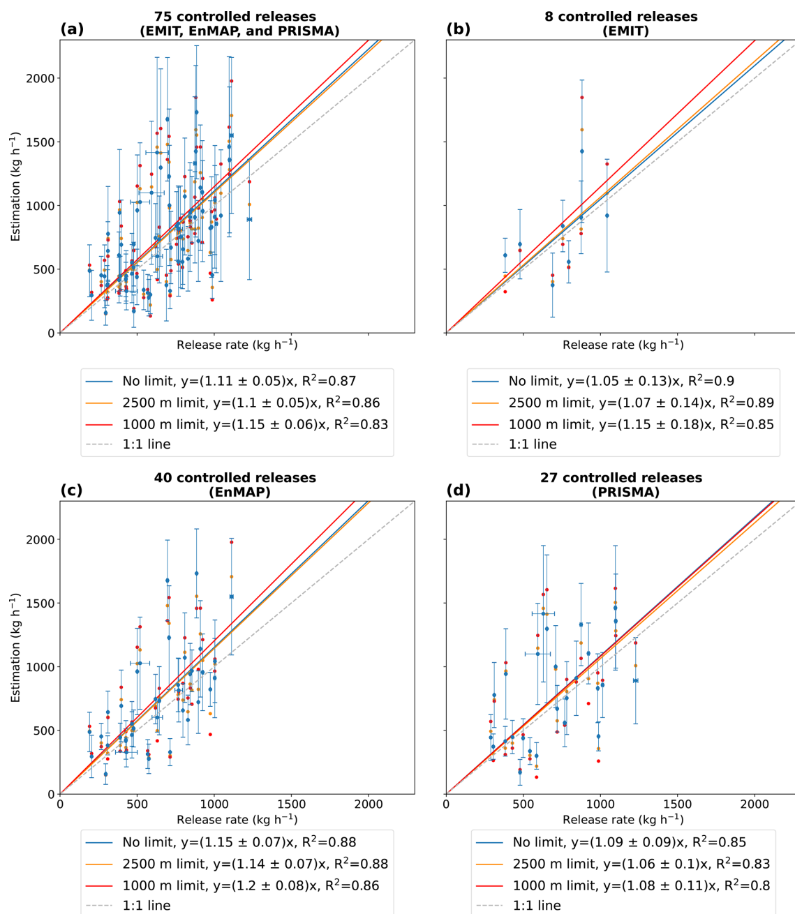
Figure 8. Quantification performance of methane-emission estimates using the IME method under different fetch limits (none, 2500, and 1000 m) with calibrations shown in Fig. 7a–c. (a) Controlled releases observed by EMIT, EnMAP, and PRISMA. (b) EMIT only. (c) EnMAP only. (d) PRISMA only. Regression lines are fitted with Ordinary Least Squares (OLS). Estimation errors are derived from HyperGas outputs. The release-rate errors are estimated as the standard deviation of mean emission rates released over consecutive time windows starting 1–5 min before and ending at the overpass time (i.e., [T - 1 \text{ min}, T] , [T - 2 \text{ min}, T] , ..., [T - 5 \text{ min}, T] ). For clarity, scatter points for the fetch-limited results are shown without error bars.
