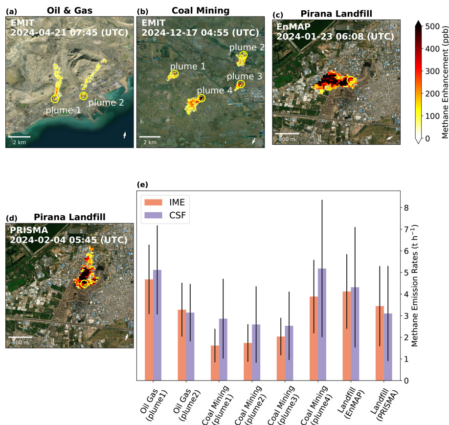
Figure 10. Methane plumes detected from various sectors using (a, b) EMIT, (c) EnMAP, and (d) PRISMA. Instrument and satellite overpass time are shown in white text at the top of each panel. Plume source locations are marked by yellow circles, with plume numbers annotated when multiple plumes are present in a single panel. ERA5 wind direction is indicated in the lower right corner of each image. (e) Methane emission estimates for the cases, derived using the IME and CSF methods. Background imagery source: Esri|Powered by Esri.
