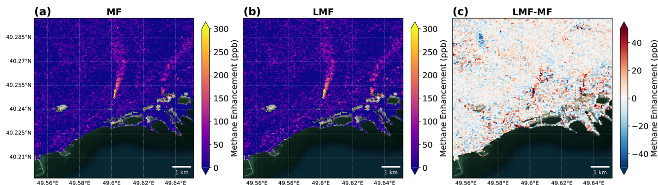
Figure 4. Retrieved methane enhancements from the EMIT observation over Azerbaijan on 21 April 2024, using (a) the matched filter method and (b) the lognormal matched filter method. Panel (c) shows the difference between the two retrievals. Water pixels are masked using the OSM and ESA WorldCover data sets. Background imagery source: Esri|Powered by Esri.
