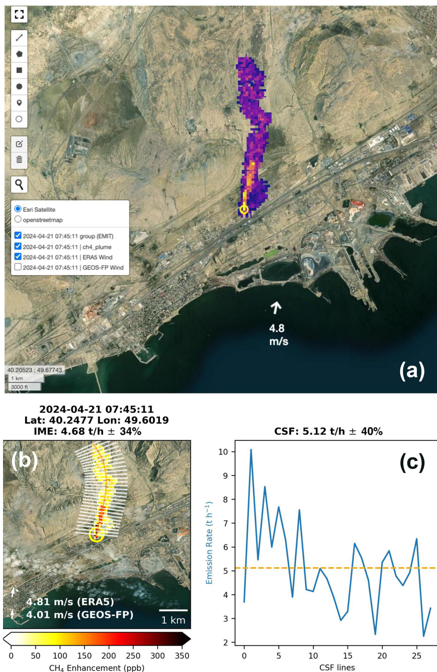
Figure 9. Example overview from the interactive application. (a) Methane plume overlaid on an ESRI basemap. Source: Esri|Powered by Esri. The emission source is marked with a yellow circle. Wind direction and speed based on ERA5 are indicated by the white arrow and text. (b) Overview of IME results. The title displays the satellite overpass time, source location, estimated emission rate, and associated uncertainty. Wind data from ERA5 and GEOS-FP are also shown. Background imagery source: Esri|Powered by Esri. (c) Emission rates along individual CSF lines, shown in white in panel (b) . The mean CSF emission rate and uncertainty are shown in the title.
