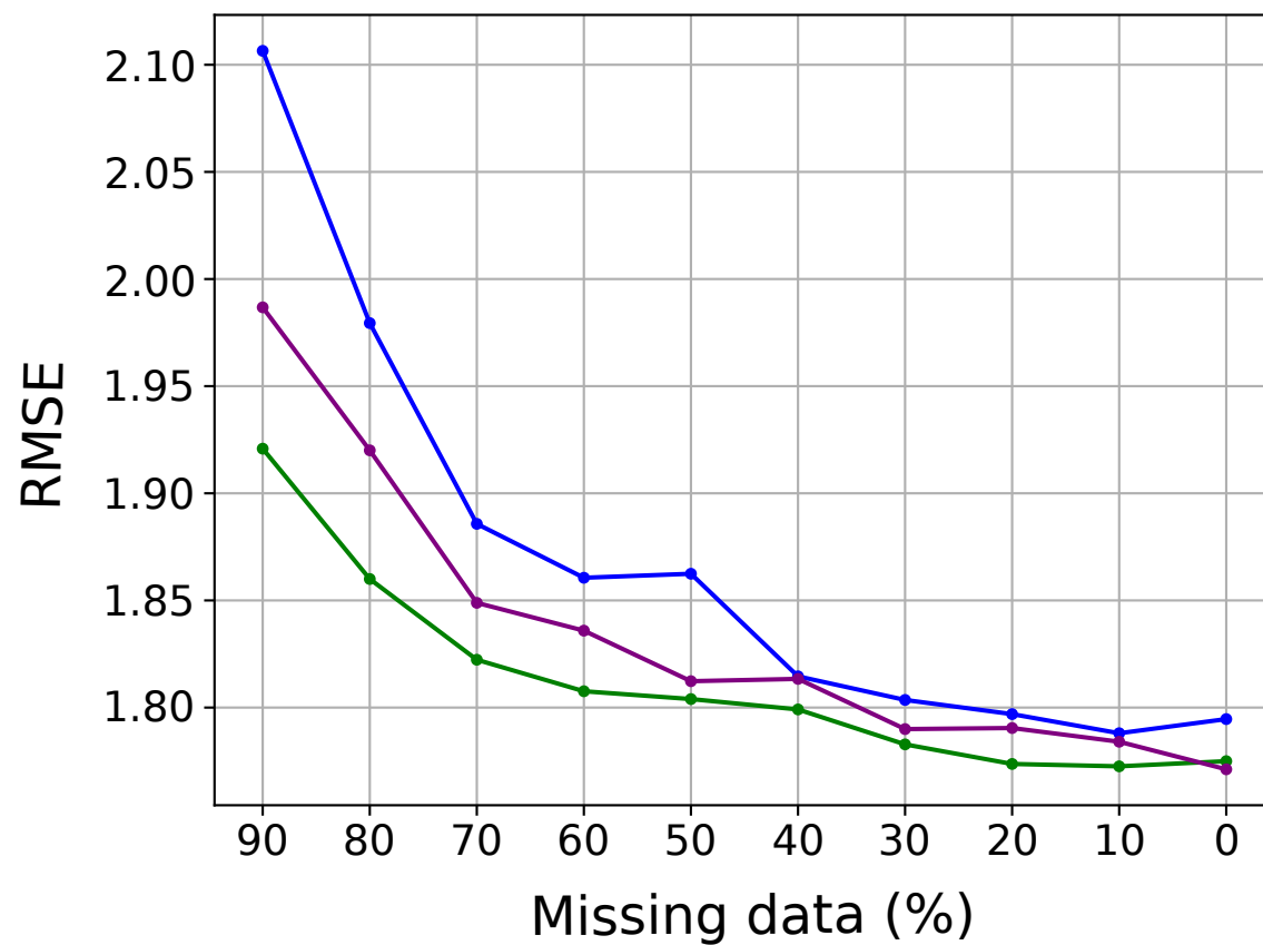
Maximum temperature
