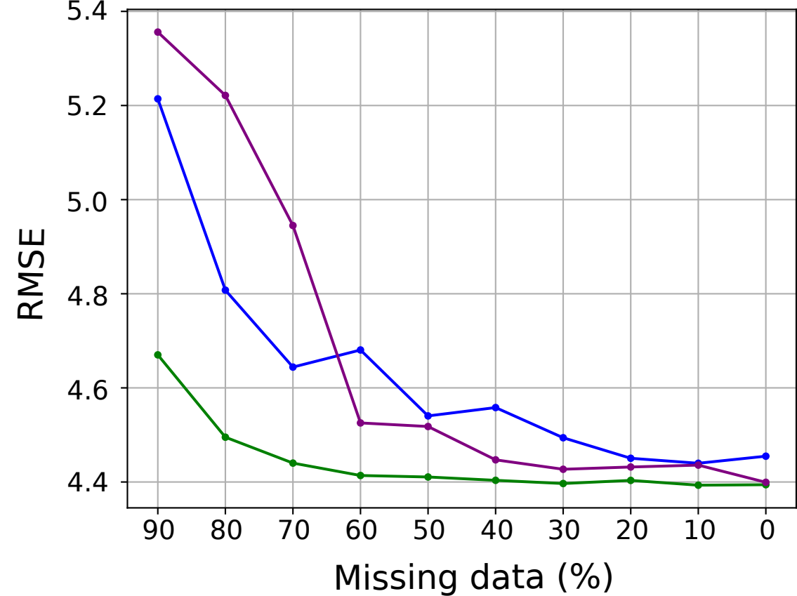
Precipitation
