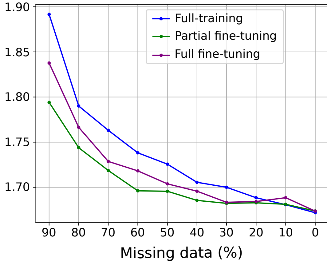
Minimum temperature
