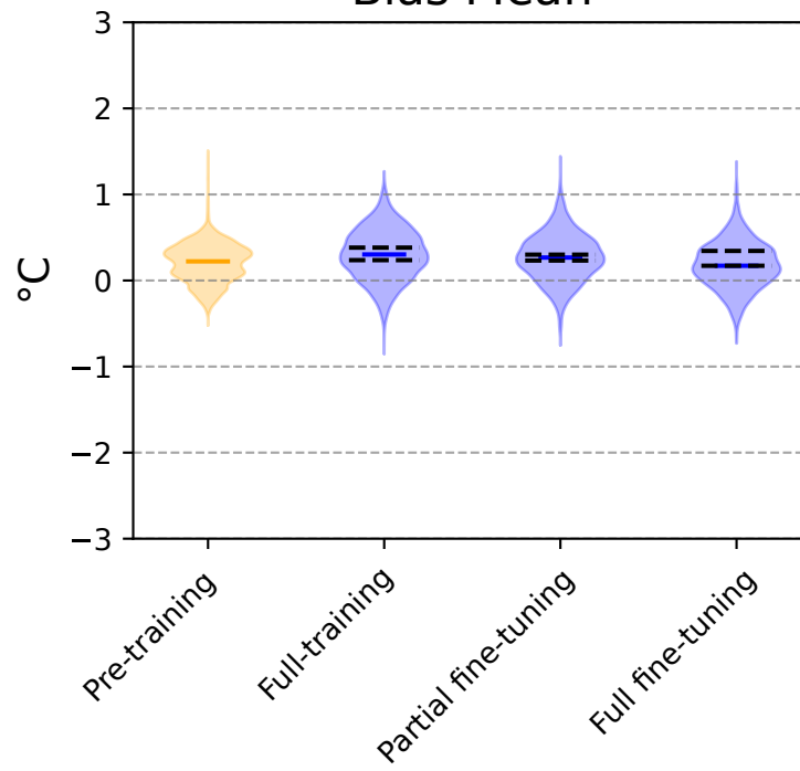
Bias Mean
