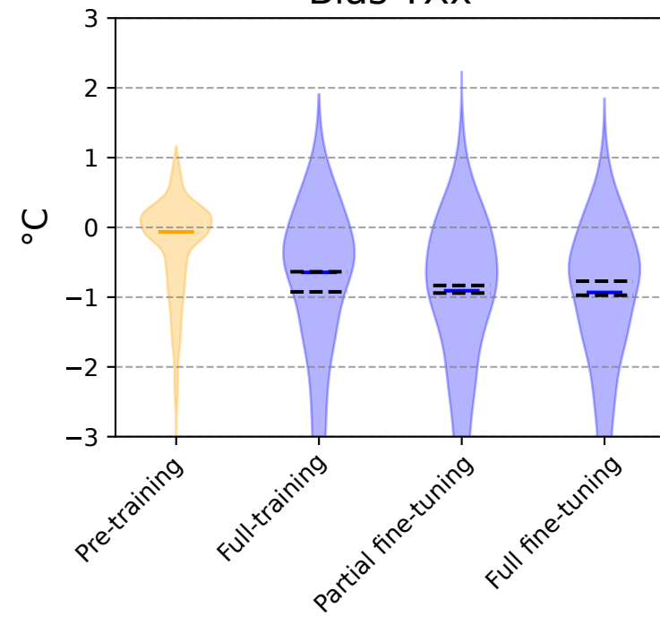
Bias TXx
