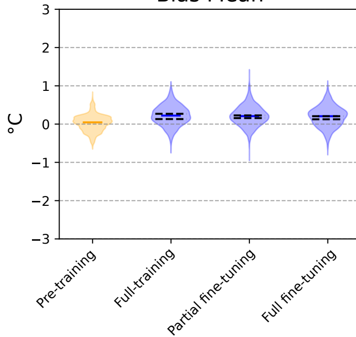
Bias Mean
