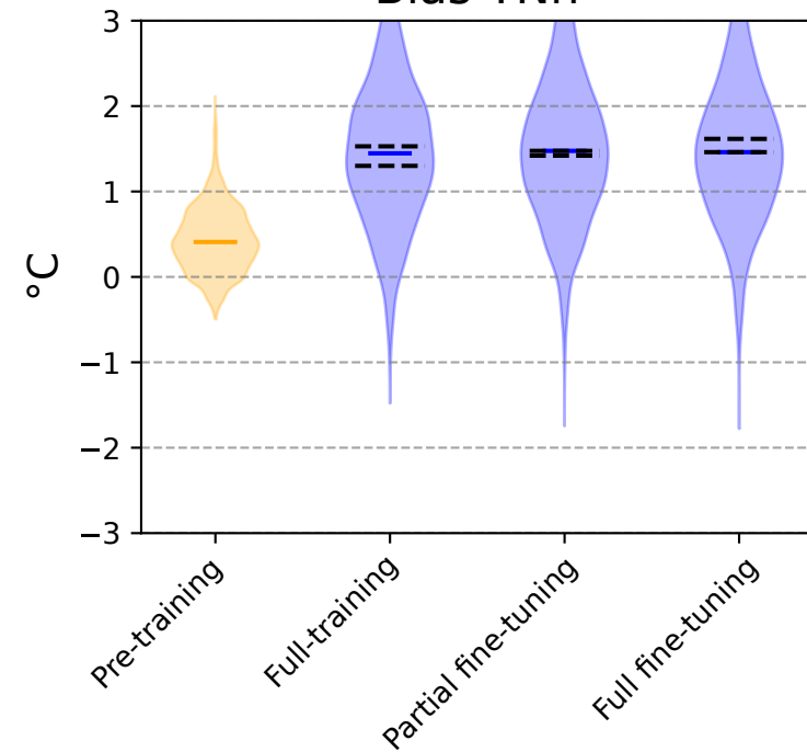
Bias TNn
