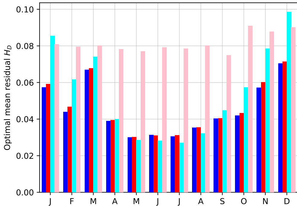
WRF-Chem
