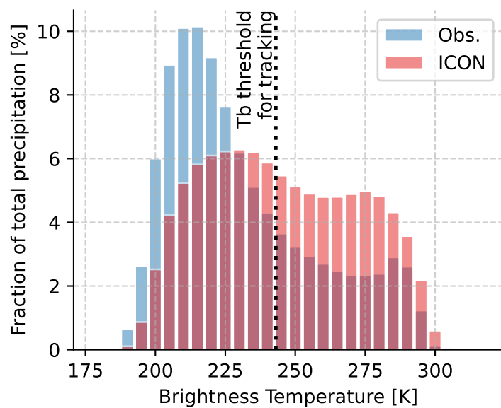
d) tropical pr contribution by Tb bins over all cells
