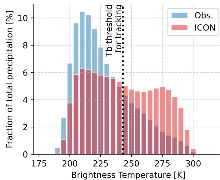
e) tropical pr contribution by Tb bins over land cells
