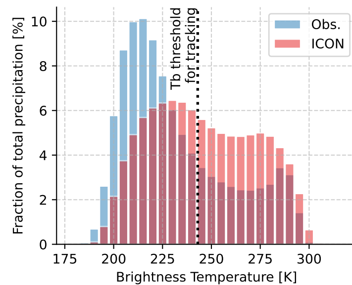
f) tropical pr contribution by Tb bins over ocean cells
