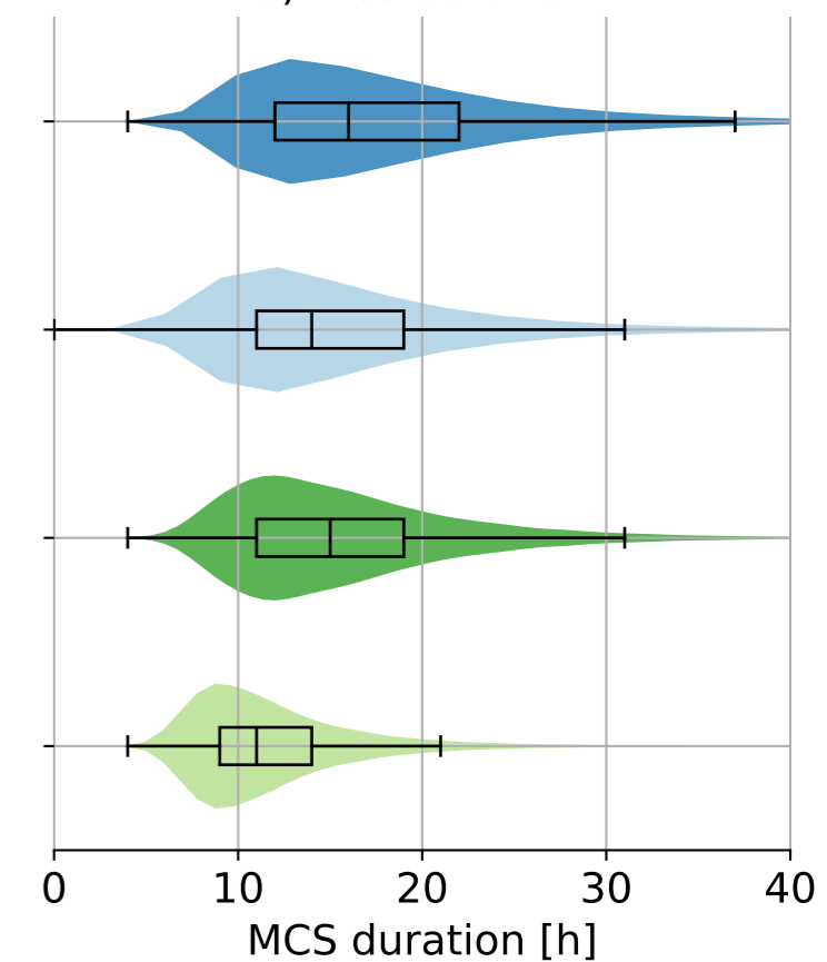
d) MCS duration
