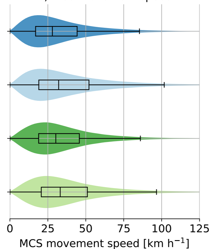
b) MCS movement speed
