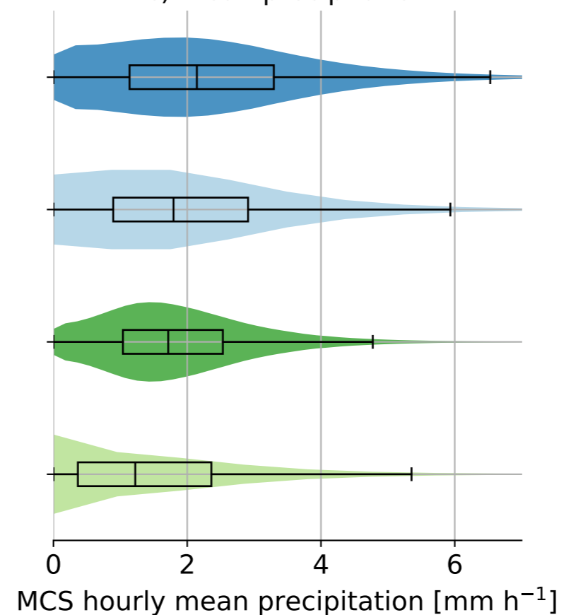
c) mean precipitation
