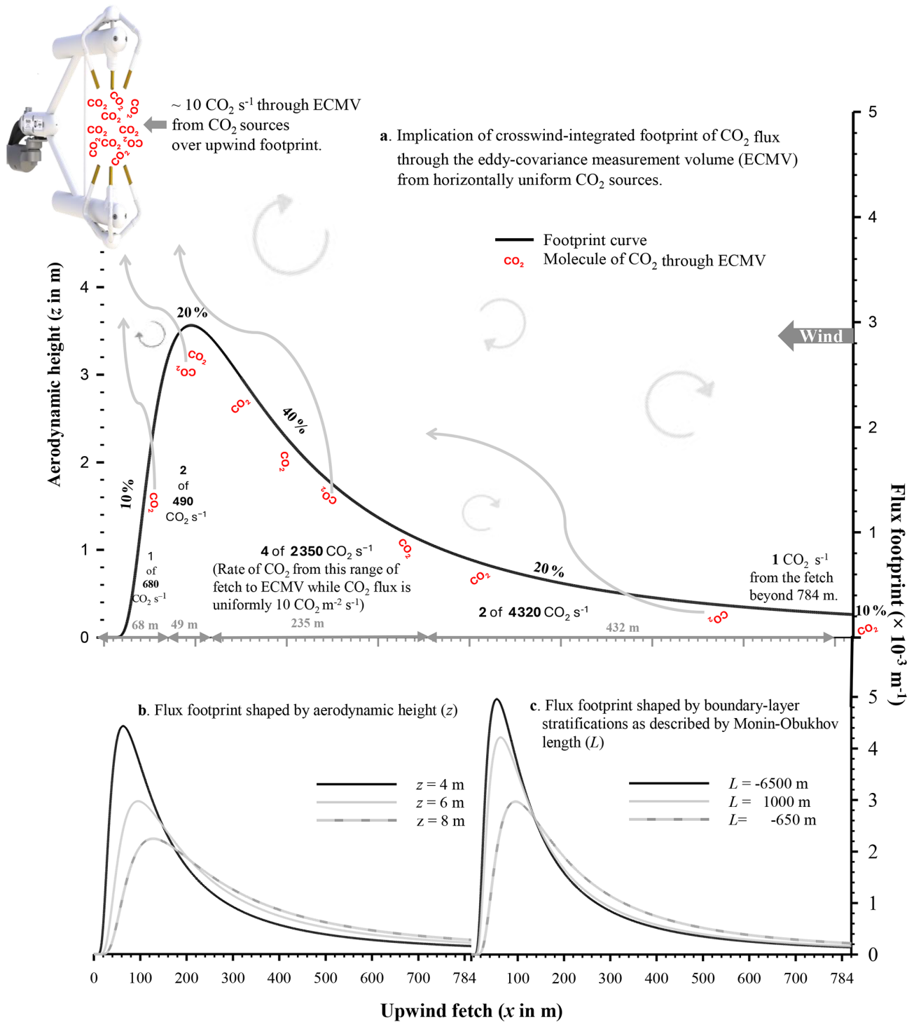
Figure 1. A flux footprint equation is displayed as a crosswind-integrated flux footprint, where the curve along the x axis shows the contribution of molecules originating at a particular value of x and for all values of y . (a) Crosswind-integrated flux footprint in a case where CO 2 flux sources are known to be uniform and emitted at a rate of 10 CO 2 molec. m -2 s -1 under convective conditions. The shape of the curve is affected by changes in sensor aerodynamic height z (i.e., height of center of measurement volume minus the zero-plane displacement height) (b) and by changes in atmospheric boundary-layer stability, as determined from the Monin–Obukhov length L and friction velocity u_* . (c) . All curves in this figure are computed using Eq. (21) in Kormann and Meixner (2001). For these curves, unless noted inside panels, z is 6 m, L is -650 m, wind speed is 5 m s -1 , u_* is 0.3–0.45 m s -1 , and the von Karman constant is 0.41.
