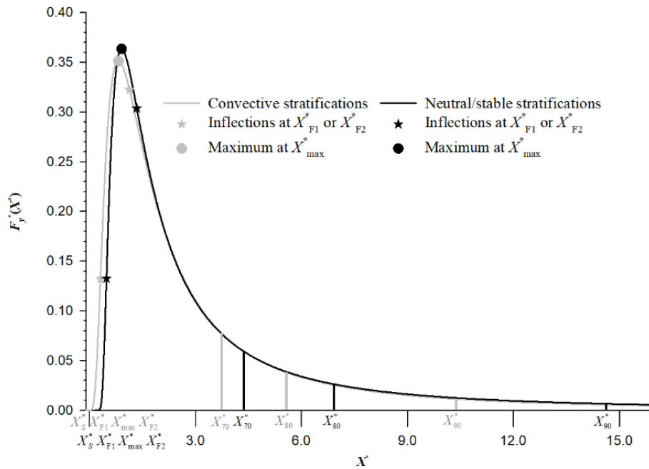
Figure 2. Nondimensional crosswind-integrated flux footprint F_y^*(X^*) as a function of nondimensional upwind fetch X^* . A vertical bar at X_p^* , where subscript “p” indicates the percent of 70, 80, or 90, is the boundary at which the integration of F_y^*(X^*) , as shown in Eq. (19), from its starting limit X_S^* is equal to p %. X_{max}^* is the location of the maximum value of F_y(X^*) . X_{F1}^* and X_{F2}^* are the 1st and 2nd inflections on a F_y(X^*) curve.
