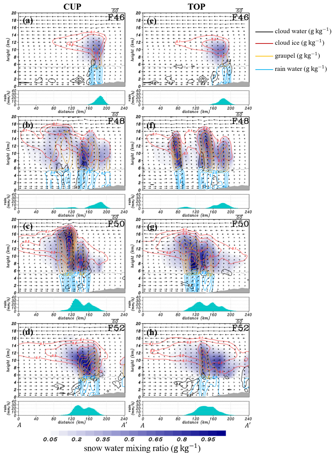
Figure 8. Vertical cross sections along the A–A′ line in Fig. 6d, e of hydrometeor mixing ratios ( \text{g kg}^{-1} ) and along-section vertical circulations (vectors; \text{m s}^{-1} ; scale shown in the top-right corner) for (a–d) CUP and (e–h) TOP at (a, e) 46 h, (b, f) 48 h, (c, g) 50 h, (d, h) 52 h forecasts. The cross sections are computed by averaging along the short axis of the dashed box denoted in Fig. 6d, e. Gray shading represents the averaged terrain height. Different contour colors represent the mixing ratios of cloud water (black; 0.2 \text{ g kg}^{-1} interval), rain water (blue; 0.3 \text{ g kg}^{-1} interval), cloud ice (red; 0.1 \text{ g kg}^{-1} interval), and graupel (yellow; 0.8 \text{ g kg}^{-1} interval), while the purple shading denotes the snow mixing ratio ( \text{g kg}^{-1} ). The greenish-blue histogram denotes the rain rate ( \text{mm h}^{-1} ).
