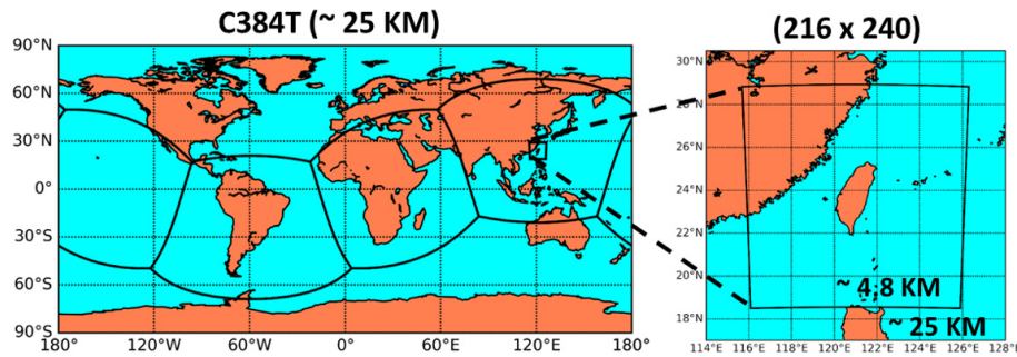
Figure 2. Illustration of TGFS tiles for global (left) and nested (right) domains. Thick black lines in the global domain indicate the boundaries of cubed-sphere tiles. The nested-grid tile, located at the center of one of the six tiles, covers the vicinity of Taiwan. The horizontal grid sizes in global and nested tiles are approximately 25 and 4.8 km, respectively.
