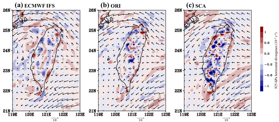
Figure 5. 925 hPa wind vectors ( \text{m s}^{-1} ) and 925 hPa horizontal divergence (shading; 10^{-5} \text{ s}^{-1} ) at 06:00 UTC 26 August 2023 from (a) ECMWF IFS analysis data and 6 h forecasts from the (b) ORI and (c) SCA experiments.
