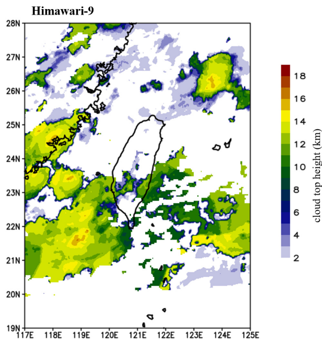
Figure 9. Cloud top height (km) derived from Himawari-9 satellite data at 23:00 UTC on 9 August 2023, corresponding to the time when the observed cloud top height reached its maximum.
