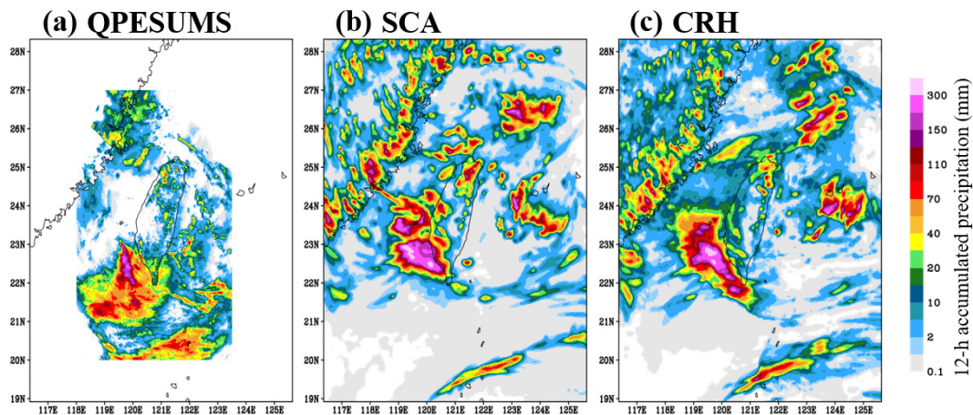
Figure 11. (a) 12 h accumulated precipitation (mm) from 00:00 to 12:00 UTC on 17 August 2023 based on QPESUMS observation. The 96–108 h accumulated precipitation forecasts valid at the same period from the (b) SCA and (c) CRH experiments.
