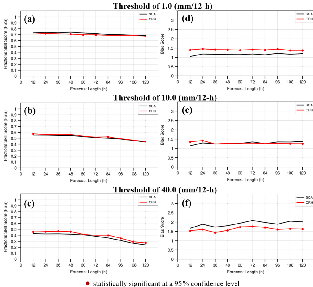
Figure 12. (a–c) Aggregated fractions skill scores, verified with a 20 km neighborhood size, and (d–f) bias scores of precipitation forecasts in the SCA (black lines) and CRH (red lines) experiments. The scores are calculated over Taiwan’s land area and for every 12 h accumulated amount within the 120 h forecasts at thresholds of (a, d) 1.0, (b, e) 10.0, and (c, f) 40.0 mm/12 h, respectively. Verifications are based on simulations initialized at 00:00 and 12:00 UTC daily from 1 July to 30 August 2023 (122 cases in total), compared against QPESUMS observations. Filled circles indicate that the differences between SCA and CRH are statistically significant at a 95 % confidence level, determined by a bootstrap test using 1000 resamples.
