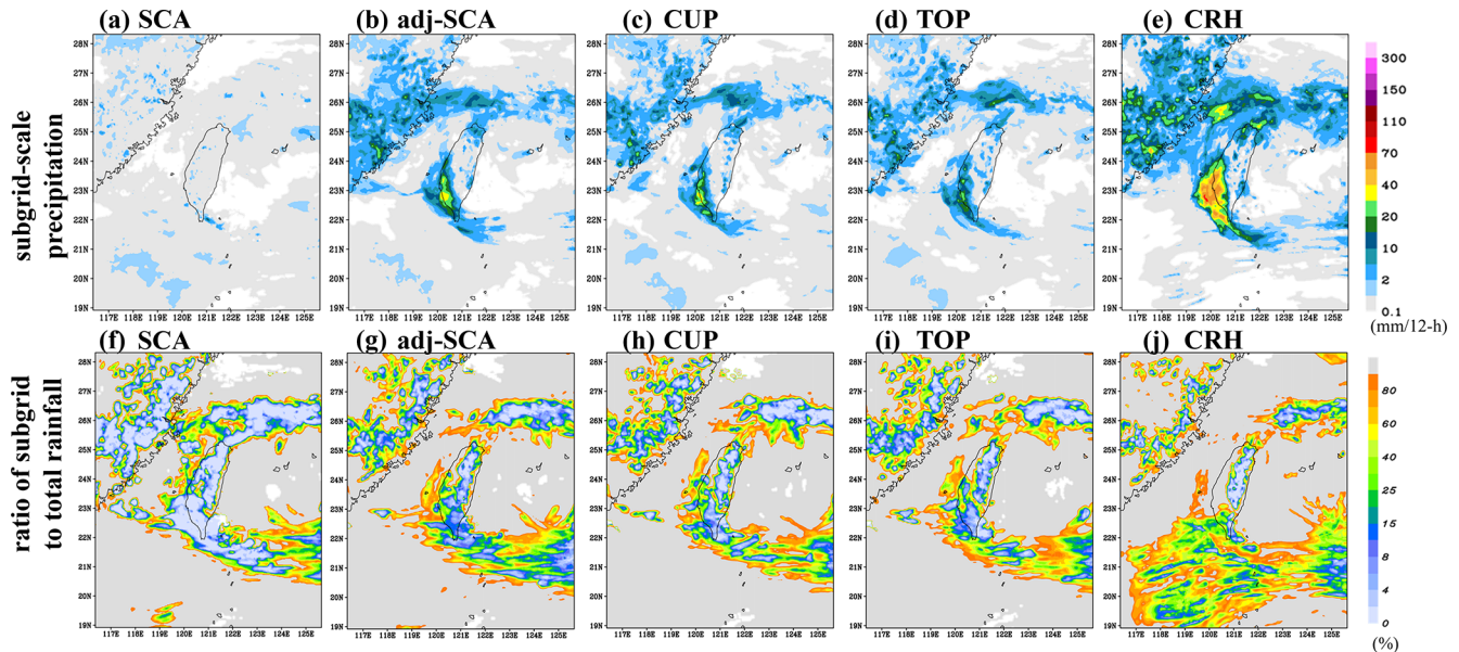
Figure 7. Same as the 48–60 h precipitation forecast in Fig. 6, but for (a–e) subgrid-scale precipitation (mm) and (f–j) the ratio (%) of subgrid-scale precipitation to total (subgrid + grid) precipitation from the (a, f) SCA, (b, g) adj-SCA, (c, h) CUP, (d, i) TOP and (e, j) CRH experiments.
