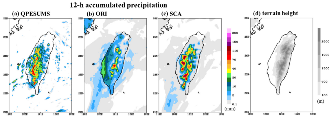
Figure 3. 12 h accumulated precipitation (mm) from 00:00 to 12:00 UTC on 26 August 2023 in (a) QPESUMS observation and TGFS nested-domain forecasts from the (b) ORI and (c) SCA experiments initialized at 00:00 UTC on 26 August 2023. (d) Terrain height (m) in the TGFS nested domain.
