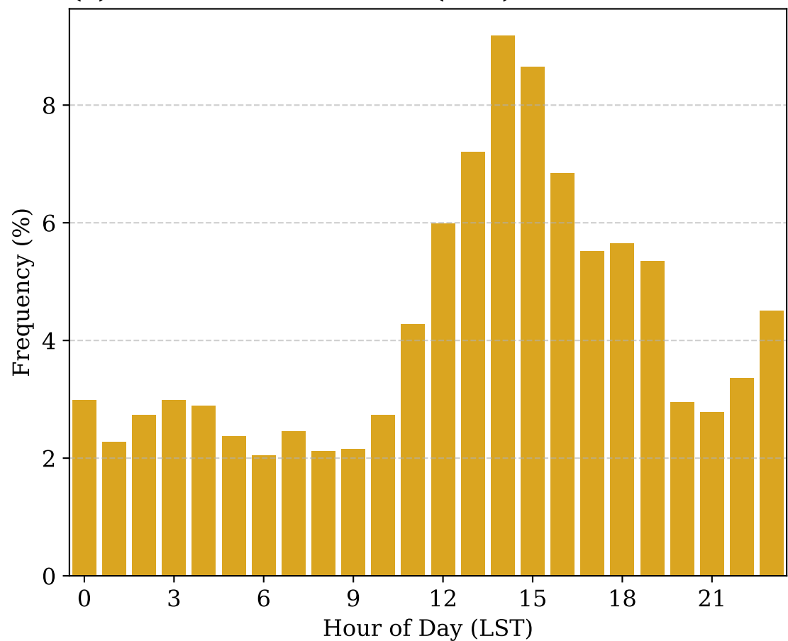
(c) MCS Initiation Time (LST)
