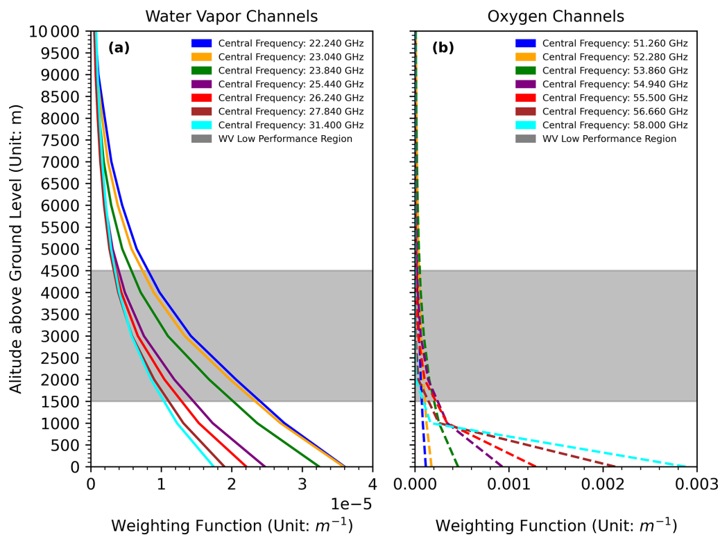
Figure 8. Weighting functions of temperature-sensitive (oxygen) and humidity-sensitive (water vapor) channels calculated with PyRTlib using the US Standard Atmosphere profile (U.S. Committee on Extension to the Standard Atmosphere, 1976) as background. The mismatch in vertical sensitivity between oxygen and water vapor channels is highlighted.
