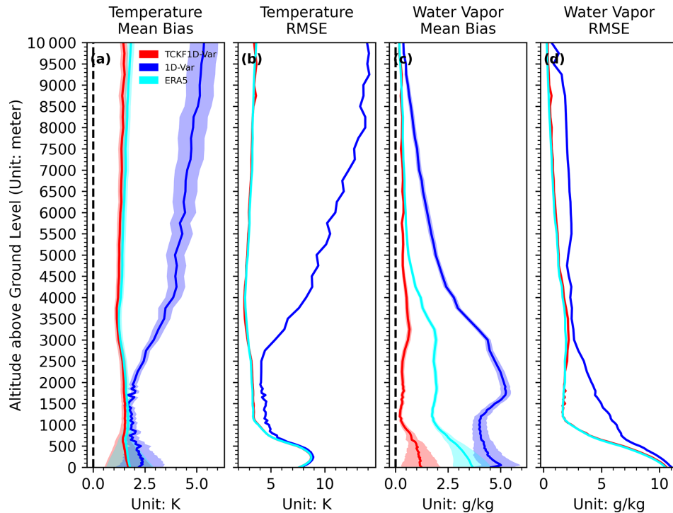
Figure 5. Validation of temperature and water vapor profiles retrieved by TCKF1D-Var (red), ERA5 a priori (cyan), and 1D-Var (blue) against radiosonde observations. The shaded areas denote the 95 % confidence intervals that have passed the significance test. For temperature, TCKF1D-Var reduces the mean bias (a) relative to the a priori and yields smaller overall random errors (b) than 1D-Var. For water vapor, TCKF1D-Var substantially decreases the mean bias (c) compared to the a priori, particularly below 5500 m, while its random errors (d) are smaller than 1D-Var near the surface but remain larger than the a priori aloft.
