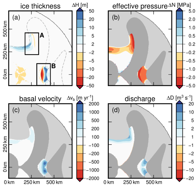
Figure 8. Result of the fully coupled (two-way) simulations using the Thule setup. Panels (a)–(d) show differences in the summer state (day 215 of year two) relative to the end of the spin-up. The panel layout is identical to Fig. 5, with ice-dynamical fields in the left column (a, c) and subglacial hydrological fields in the right column (b, d). Differences are evaluated on the common grounded domain, except for panel (a), where ice thickness differences are shown wherever ice thickness is defined. The maps show approximately one quarter of the model domain, exploiting symmetry along both horizontal axes. Rectangles (A, B) indicate regions of high activity referenced in the text.
