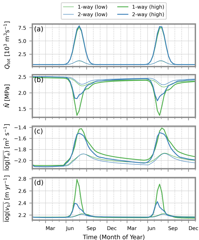
Figure 6. Time series of total water source Q_{\text{tot}} , mean effective pressure \bar{N} , mean effective transmissivity magnitude \log(T_e) , and mean basal velocity magnitude \log(v_b) for the four simulations: one-way coupling in green, two-way coupling in blue; high-amplitude forcing shown with thick lines, low-amplitude forcing with thin lines. The means are evaluated as spatial means on the time-dependent active CUAS mask.
