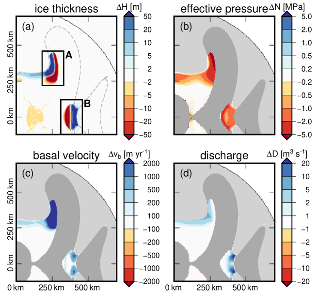
Figure 7. Results of the one-way coupled simulations using the Thule setup. Panels (a)–(d) show differences in the summer state (day 215 of year two) relative to the end of the spin-up. The panel layout is identical to Fig. 5, with ice-dynamical fields in the left column (a, c) and subglacial hydrological fields in the right column (b, d). Differences are evaluated on the common grounded domain, except for panel (a), where ice thickness differences are shown wherever ice thickness is defined. The maps show approximately one quarter of the model domain, exploiting symmetry along both horizontal axes. Rectangles (A, B) indicate regions of high activity referenced in the text.
