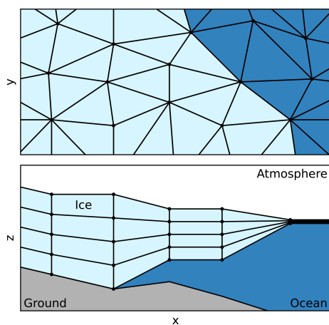
Figure 2. Schematic diagram of the ISSM mesh for 2D and 3D setups. The 2D mesh is an unstructured triangle grid covering the whole domain in the horizontal direction, even where there is no ice (top panel). Triangle elements are completely ice or completely ocean. The 3D mesh is generated by extruding the 2D mesh in multiple layers of triangle prism elements (bottom panel). The vertices in every layer have the same x and y coordinates. The z coordinate is set to match the ice's vertical extent and is updated when the ice thickness changes. In ice-free areas, the mesh collapses vertically to a minimum thickness.
