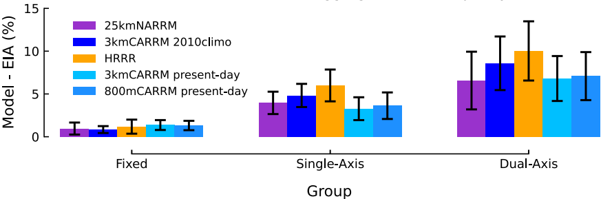
Absolute bias (relative to EIA) of aggregated solar capacity factor
