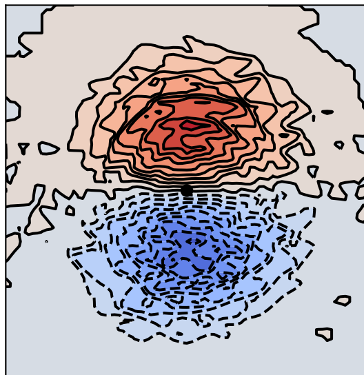
Eastward wind
