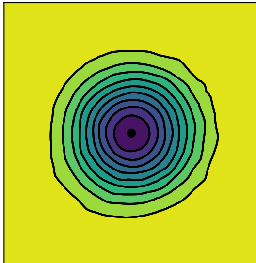
C0 interpolation
