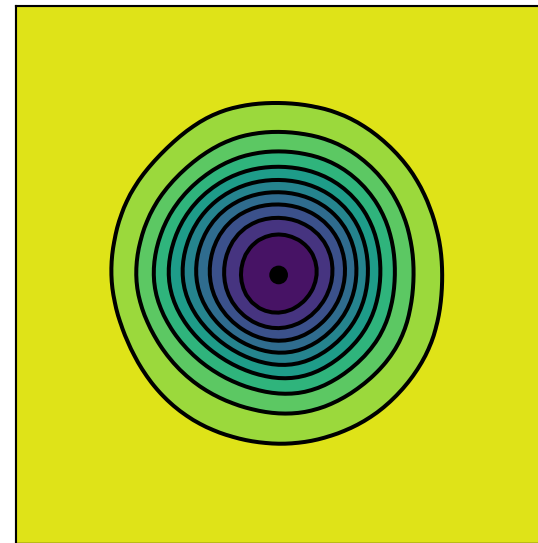
Smoothing interpolation
