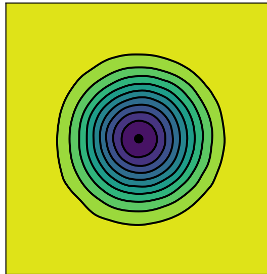
C1 interpolation
