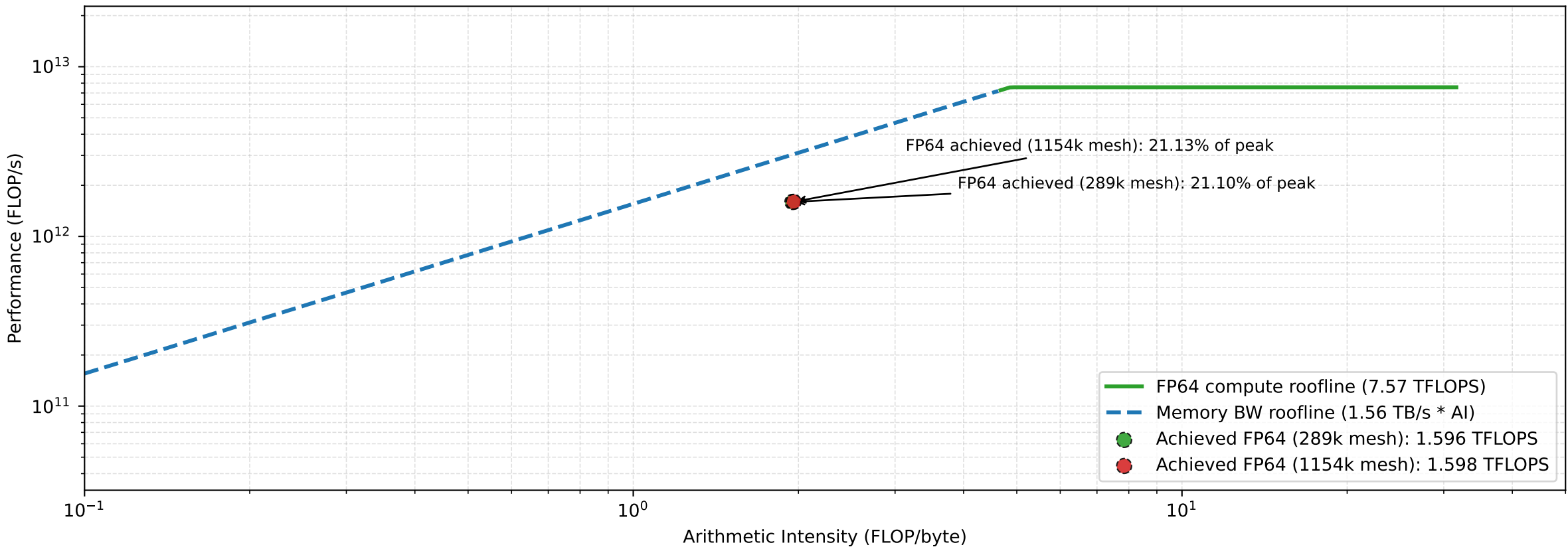
computeTracerTendenciesOnly Kernel Roofline (FP64) — NERSC Perlmutter-GPU (NVIDIA A100)
