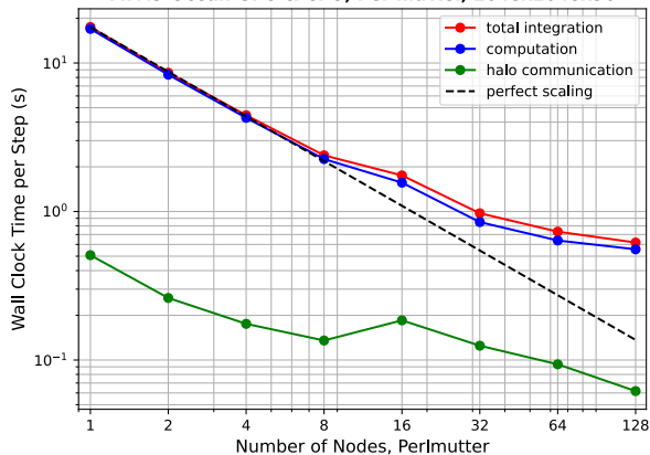
MPAS-Ocean GPU & CPU, Perlmutter, 2048x2048x96
