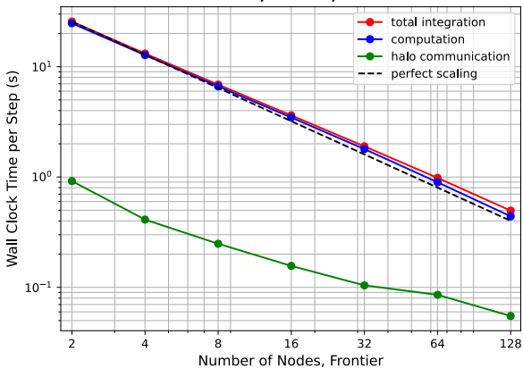
MPAS-Ocean CPU, Frontier, 2048x2048x96
