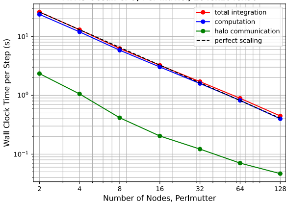
MPAS-Ocean CPU, Perlmutter, 2048x2048x96
