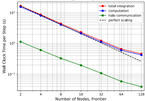
MPAS-Ocean GPU, Frontier, 2048x2048x96
