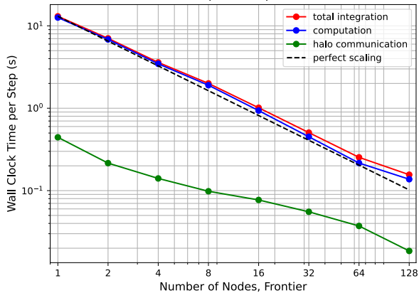
MPAS-Ocean CPU, Frontier, 1024x1024x96
