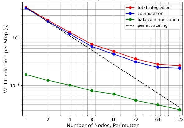
MPAS-Ocean GPU & CPU, Perlmutter, 1024x1024x96
