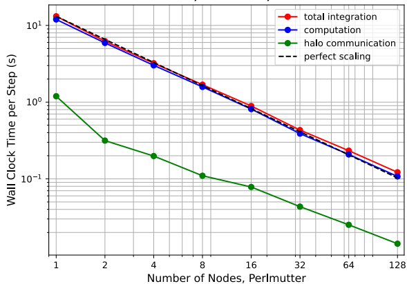
MPAS-Ocean CPU, Perlmutter, 1024x1024x96
