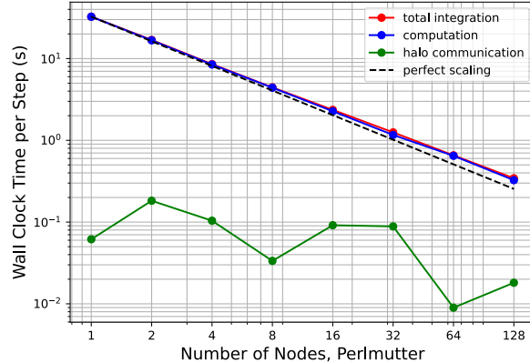
Omega-0 CPU, Perlmutter, 2048x2048x96
