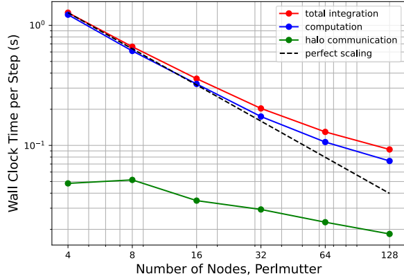
Omega-0 GPU, Perlmutter, 2048x2048x96
