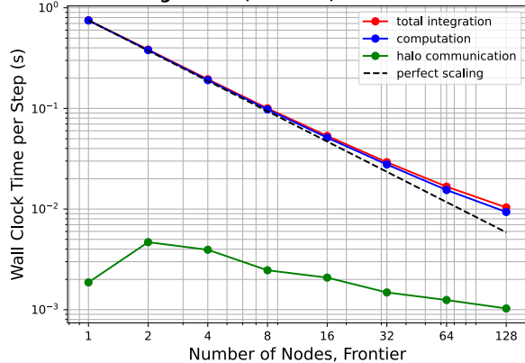
Omega-0 GPU, Frontier, 2048x2048x96
