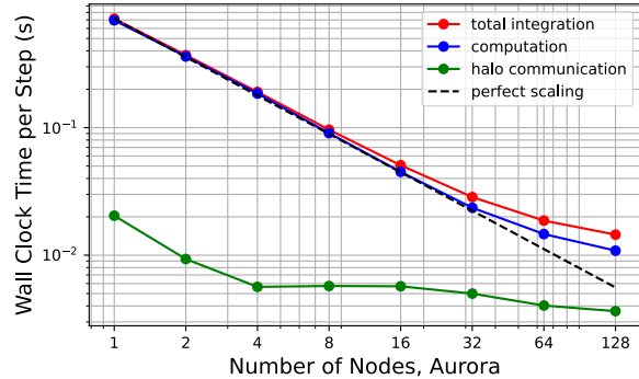
Omega-0 GPU, Aurora, 2048x2048x96
