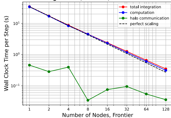
Omega-0 CPU, Frontier, 2048x2048x96
