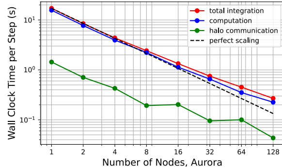
Omega-0 CPU, Aurora, 2048x2048x96
