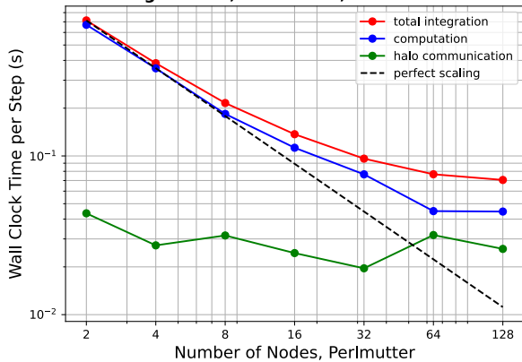
Omega-0 GPU, Perlmutter, 1024x1024x96
