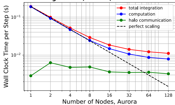
Omega-0 GPU, Aurora, 1024x1024x96
