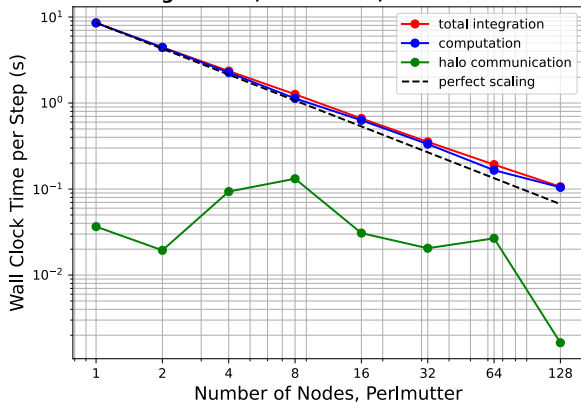
Omega-0 CPU, Perlmutter, 1024x1024x96
