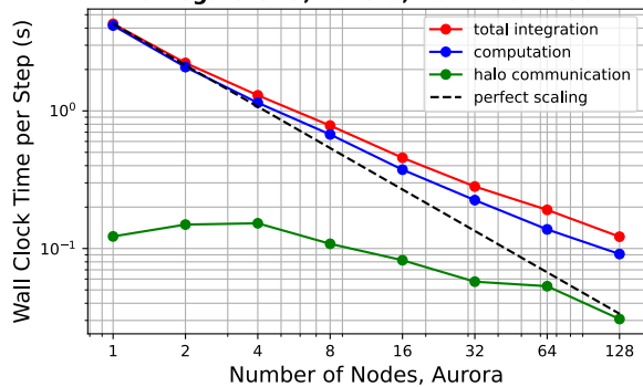
Omega-0 CPU, Aurora, 1024x1024x96
