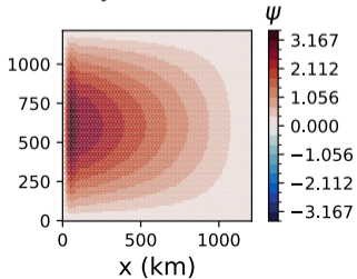
Analytical solution
