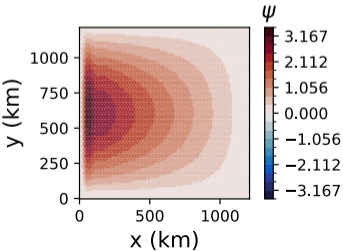
Numerical solution
