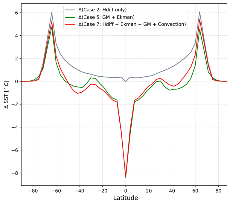
Figure 4. Zonal-mean sea surface temperature (SST) differences of the aquaplanet between selected simulations and Case 1 (no ocean heat transport, OHT), highlighting the impact of various transport mechanisms on the climate. The grey line shows the SST difference for Case 2 (horizontal diffusion only), the green for Case 5 (Gent–McWilliams and Ekman transport), and the red for Case 7 (all OHT enabled).
