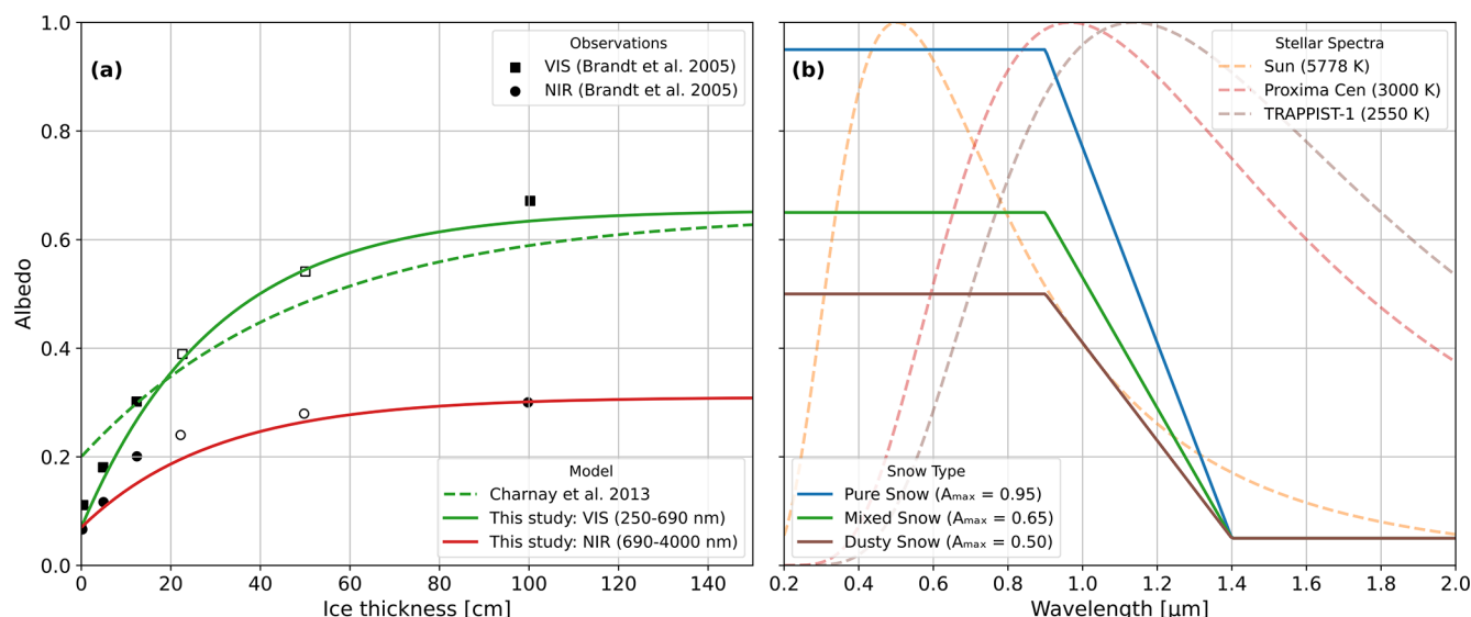
Figure 1. (a) Bare sea ice albedo as a function of ice thickness in the Visible (VIS; green) and Near-Infrared (NIR; red) bands in our study, with curves fit to Antarctic observations from Brandt et al. (2005, filled symbols: measurements; open: interpolated). The spectrally-independent albedo used in Charnay et al. (2013) is shown for reference (dashed green). (b) Broadband spectral distribution of snow and ice albedo for pure (blue), mixed (green), and dusty (brown) snow – with A_{\max} values of 0.95, 0.65, and 0.50, respectively. Dashed lines indicate the normalised black body emission of the Sun (orange), Proxima Centauri (red), and TRAPPIST-1 (brown).
