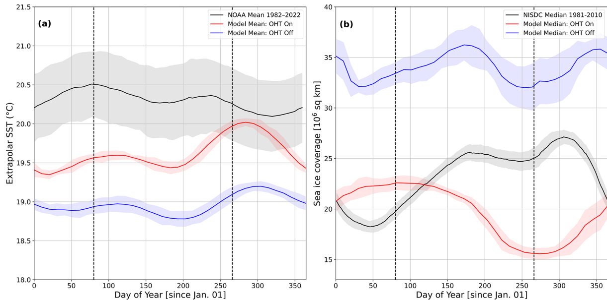
Figure 8. (a) Seasonal evolution of extrapolar sea surface temperatures (SST; 60° S–60° N), and, (b) global sea ice coverage for NOAA/NISDC observations (black), for the model with ocean heat transport enabled (red), and disabled (blue). Shaded regions represent the 2\sigma inter-annual variability (30–40 years). Vertical dashed lines indicate the timing of the March and September equinoxes.
