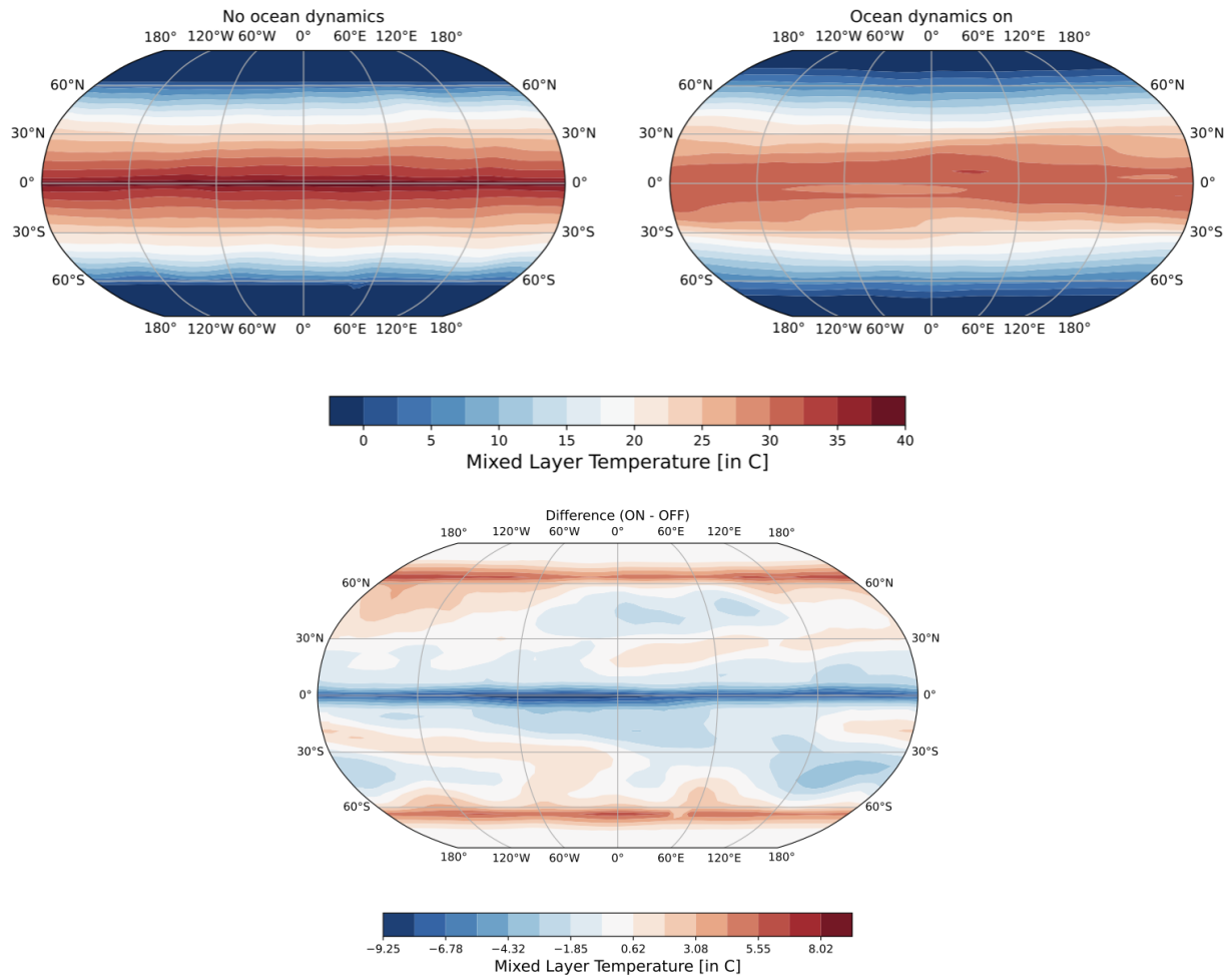
Figure C1. Annually averaged sea surface temperature (SST) maps for the zero-obliquity aquaplanet simulations. The top-left panel shows SST for Case 1 (no ocean heat transport, OHT), while the top-right panel shows SST for Case 7 (all OHT enabled). The bottom panel displays the difference between the two (Case 7 – Case 1), highlighting the impact of OHT. Notable features include equatorial upwelling of cold water and enhanced warming at higher latitudes.
