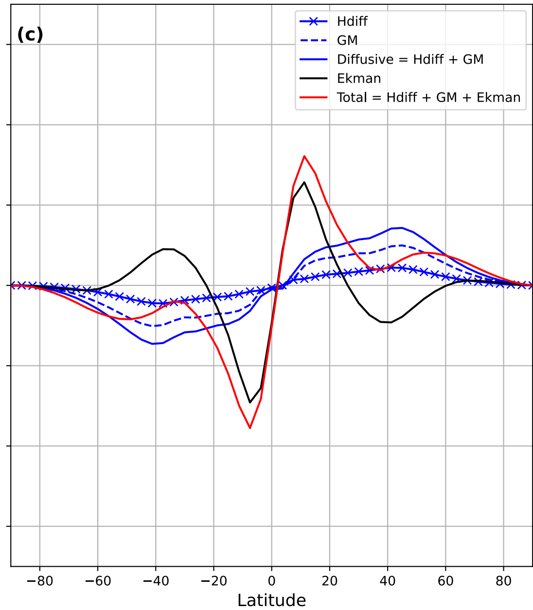
This work: Hdiff8000 + Ekman + Sve. + GM2000 + Conv.
