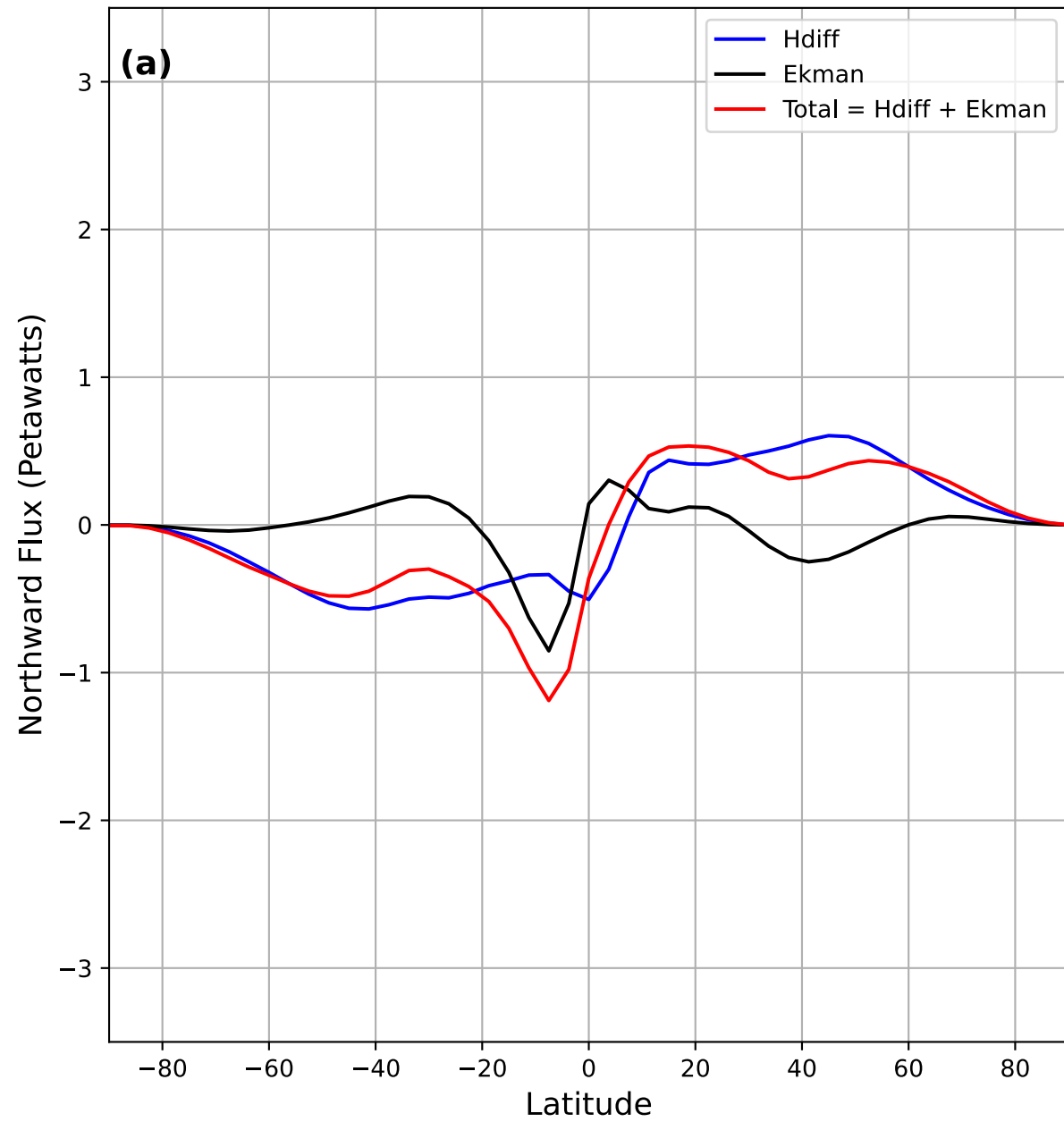
Codron (2012) Setup: Hdiff25000 + Ekman + Conv.
