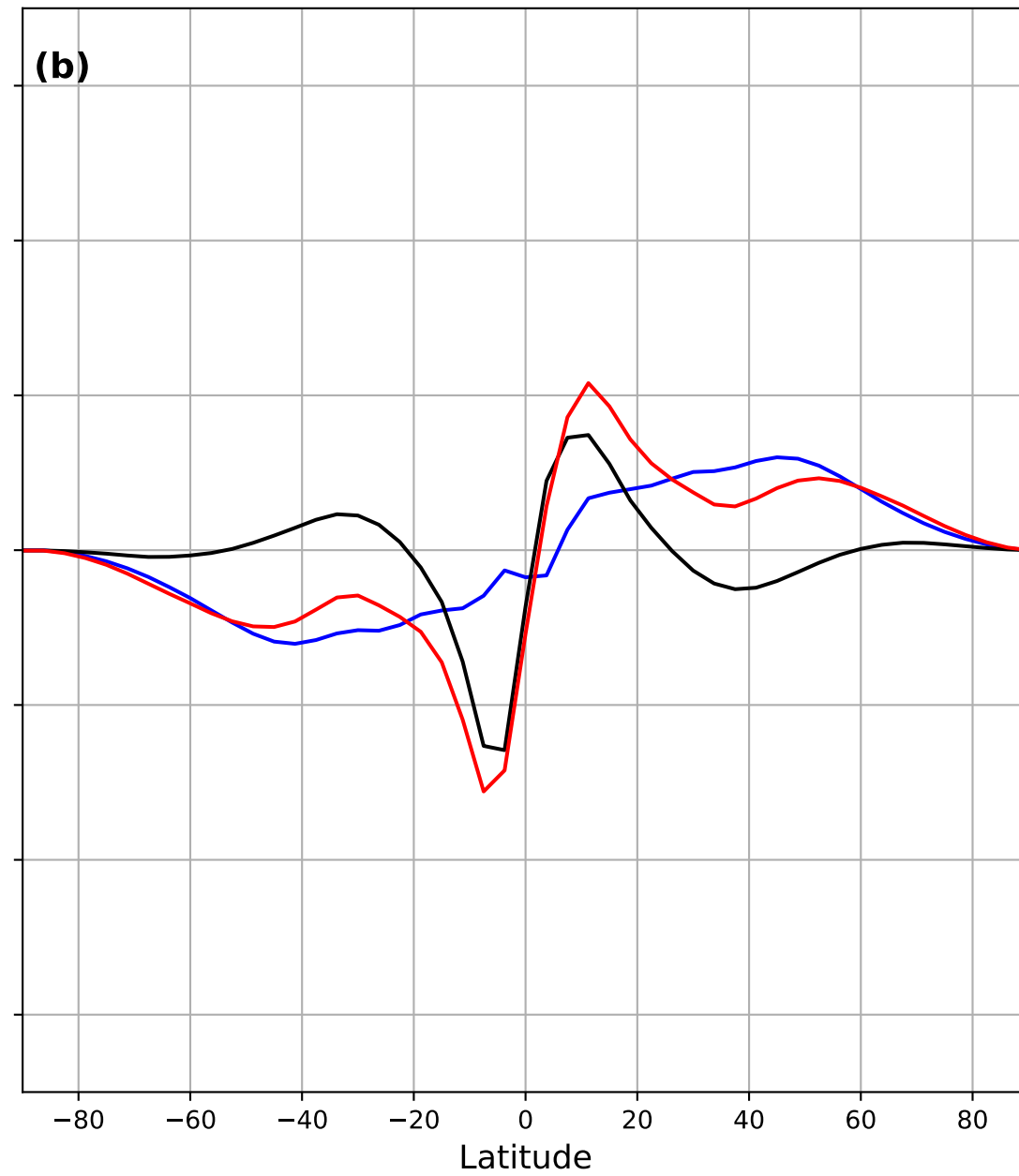
Codron (2012) Setup + Sve.
