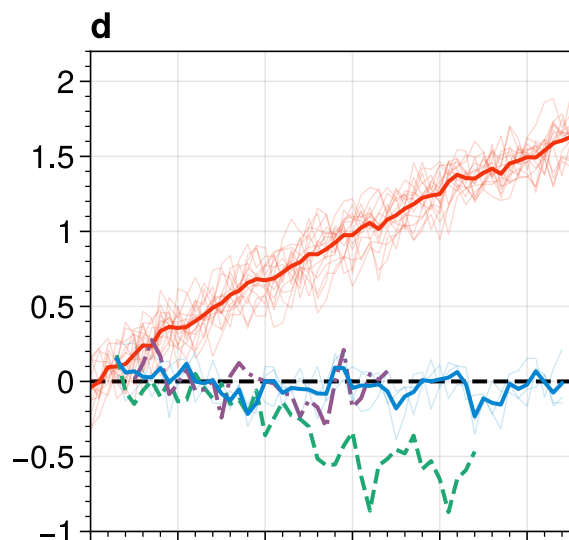
Global Mean 2m Temperature Anomaly from 2020-2039 ( \Delta K )
