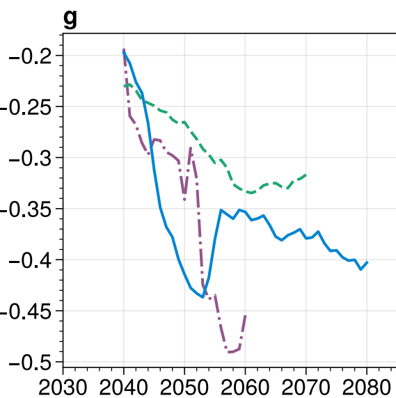
MCB GMST anomaly per SSA mass emission (K yr/Tg)
