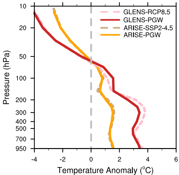
a) SSP2-4.5/RCP8.5 versus PGW
