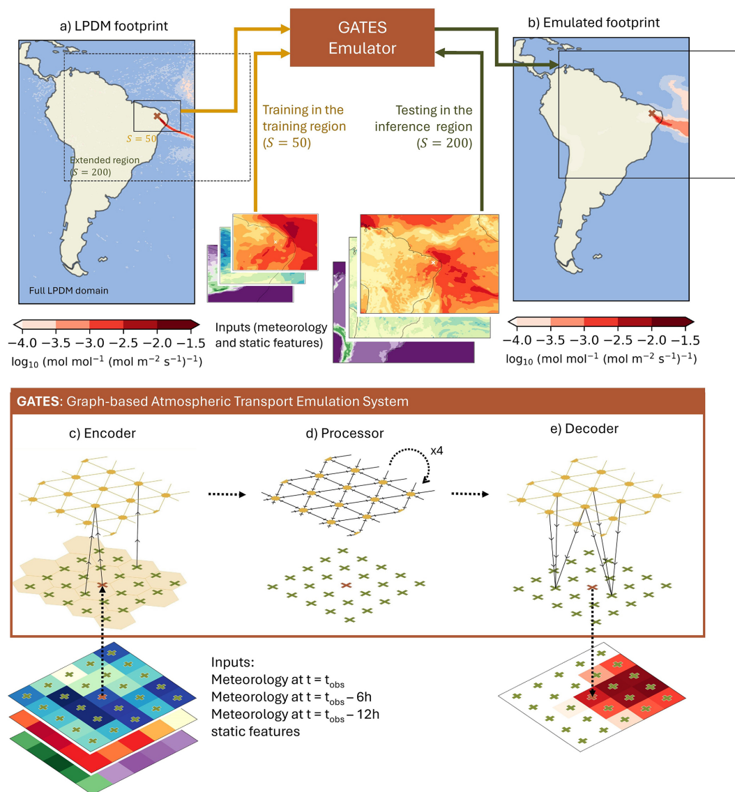
Figure 1. GATES model schematic and architecture. Top: (a) Example of an LPDM-generated footprint ( \sim 20 min to generate on a single CPU) showing the sensitivity of a satellite measurement to fluxes from the surrounding domain. (b) Corresponding GATES-emulated footprint ( \sim 1.5 s to generate). Both (a) and (b) are shown over the full LPDM domain and resolution ( 0.352^\circ \times 0.234^\circ , \approx 33 \text{ km} \times 25 \text{ km} in mid-latitudes) used in Tunnicliffe et al. (2020). In (a) , the solid-line box corresponds to the training region, a square of size 50 \times 50 grid-cells centered around the coordinates of the satellite measurement. The solid-line box in (b) corresponds to the inference region, a 200 \times 200 grid-cell square over which footprints were emulated. When this area escapes the original footprint domain, as above, the added space is filled with zeros and ignored in evaluation (here shown as whitespace inside the boxes). Bottom: Architecture of the graph and emulator, demonstrated for a square domain of size 5 \times 5 . GATES is composed of (c) an encoder, (d) a processor, and (e) a decoder. The black solid arrows indicate the flow of information. The inputs are represented as node attributes on a latitude–longitude grid (crosses) centered around the measurement point (red cross). (c) In the encoder, local regions of the inputs are mapped into nodes in the abstract feature space (yellow hexagons), arranged as a triangular mesh. Each mesh-node is connected with edges to its six neighbors (yellow lines). (d) In the processor, each mesh-node is updated using message-passing from the neighboring nodes. Four independent message-passing blocks are learned. (e) The decoder maps the latent space back to the original latitude–longitude grid of the same resolution as the inputs, outputting the footprint value at each node.
