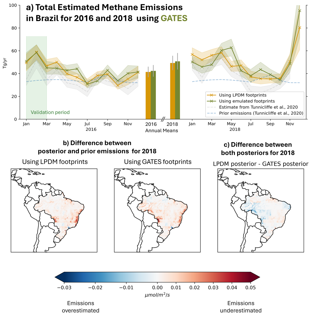
Figure 3. Deriving methane emissions for Brazil, in time (top panel) and space (bottom panels). (a) Estimated methane emissions, for 2016 and 2018. We compare the emissions estimates derived in an inversion using the LPDM footprints (yellow) with those emulated by GATES (green). The emissions inferred with the emulated footprints are well within the posterior inversion uncertainty of the emissions inferred with the traditional method. Note that we report the annual means (bars at the center of the plot) for the full 2016 (i.e. including the validation set January–March) to allow for like-for-like comparisons with 2018. We also show the monthly priors used by Tunncliffe et al. (2020) and their derived emissions. (b) Difference between the inversion posterior and prior fluxes for 2018, using the LPDM footprints (left) and the GATES footprints (right). The difference highlights the areas that were underestimated or overestimated in the initial estimate. The fluxes calculated with the GATES footprints (right) show good spatial agreement with those calculated from the traditional method (left). (c) Difference between the two posteriors for 2018. Blue shows the areas where the GATES posterior estimates higher emissions than the LPDM posterior, and red shows the opposite.
