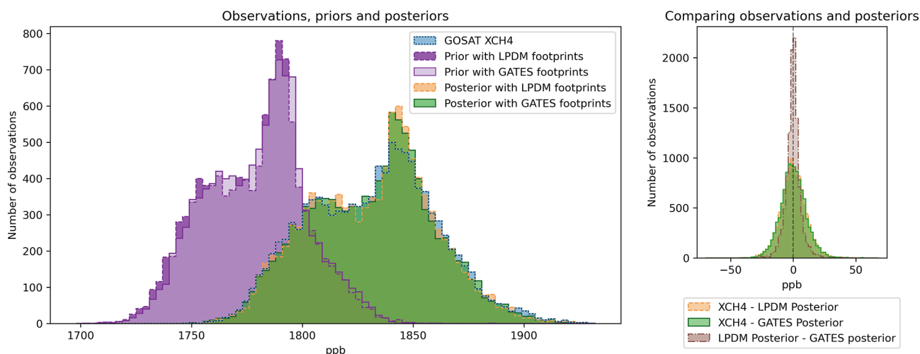
Figure G1. Comparing the distributions of the GOSAT observations, prior and posterior mole fractions in 2018. Left panel: Distributions for a priori modelled methane mole fractions (dark and light purple), GOSAT XCH_4 observations (blue) and the posterior mole fractions (orange and green). We show the prior and posterior pair generated with the LPDM footprints (purple and orange, respectively, dashed edges) and the posterior and prior pair generated with the GATES footprints (purple and green, respectively, solid edges). Both posteriors fit the observations well. Right panel: Distribution of errors between the XCH_4 observations and the mole fractions calculated from both sets of posteriors (in orange and green), and differences between the mole fractions derived with both posteriors (brown). Both posteriors show similar error patterns between the estimated emissions and the actual XCH_4 observations. The errors between the two posteriors (brown) are normally distributed, with a small positive mean bias (2.69 ppb) which indicates a small overpredicting tendency in GATES.
