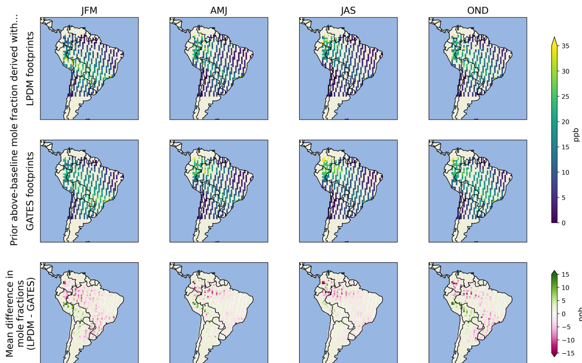
Figure E1. Seasonal mean above-baseline mole fractions, derived with the LPDM footprints (top row), with GATES footprints (middle row) and the difference between the two (bottom row). The mole fractions are derived by convolving a monthly emissions prior with each footprint (see Sect. 5.2 or Tunnicliffe et al. (2020) for a description of the prior). Here, the mole fractions are binned by season (see key below) and in 1^\circ bins, averaged for both 2016 and 2018. The mole fractions calculated with GATES footprints (middle row) show similar spatial patterns to those calculated with LPDM footprints (top row). The two are compared in the bottom row, where positive values (green) indicate mole fractions that were underpredicted by GATES, and negative values (pink) indicate mole fractions that were overpredicted by GATES. (Key: JFM = January, February, March, AMJ = April, May, June, JAS = June, July, August, OND = October, November, December).
