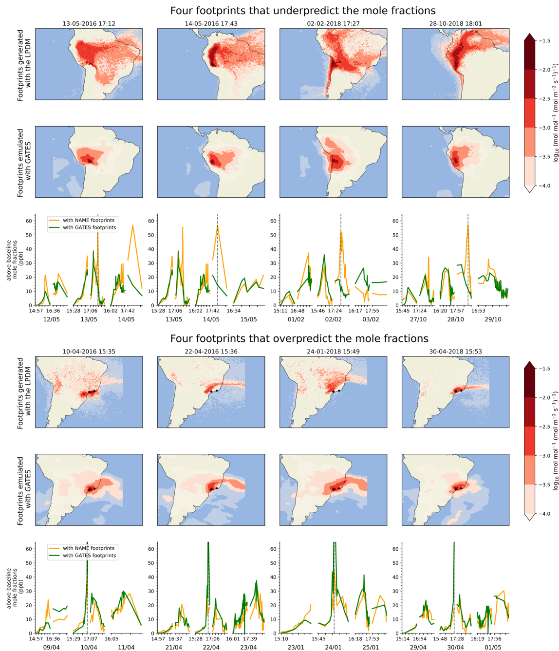
Figure F1. Two sets of footprints that lead to the largest errors in the emulated mole fractions, through underprediction (top panel) or overprediction (bottom panel). In each panel, we show the LPDM footprint (top row), the GATES-emulated footprint (bottom row) and the derived mole-fraction timeseries, for the day of the footprint, the day before and the day after. Top panel: Footprints for measurements near the central Andes area accumulate higher errors than other areas (see Fig. D1), and for these four footprints GATES fails to emulate complex dispersion patterns from difficult meteorology and topography. The LPDM footprints capture dispersion over the Amazon basin, where estimated emissions are large, leading to a big difference between the two estimates. Bottom panel: The smoothing effect is particularly visible here, as sharp, narrow plumes in the LPDM footprints over or near Sao Paulo and Rio de Janeiro (black dots) are emulated to be wider and with softer edges. When convolved with the prior, the large emissions from the cities inflate the small errors in the GATES footprints, leading to overpredictions.
