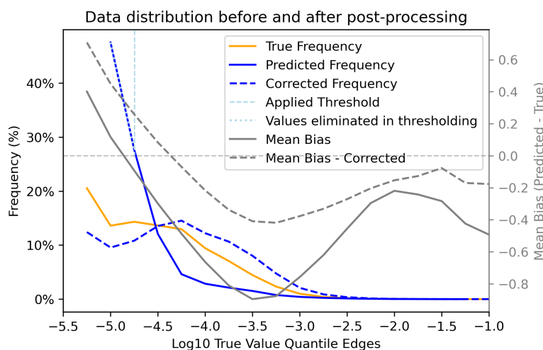
Figure B2. Impact of the bias correction on the data distribution of the test set. In orange we show the logged distribution of the test data (wherever it is non-zero) for April–December 2016 (left axis), split into 20 bins. The distribution of the values predicted directly by GATES is shown with the blue line: there is a very high proportion of small background values. The solid gray line, on the right axes, indicates the mean bias of the raw GATES predictions in each quantile of the true data (in the logged space). GATES tends to under-predict particularly the mid-range values ( \log(f) \approx -3.5 ). The post-processing steps are then applied. First we remove background values under a threshold tuned with the validation set ( 1.757 \times 10^{-5} ), indicated by the dashed light blue line. Bias correction is then applied on the remaining values, with the resulting distribution shown as the dashed blue line. The corrected presents an improved fit against the true frequency, and the mean bias of the two distribution with a dashed gray line on the right axes, shows that the mid- and high-range values are better captured.
