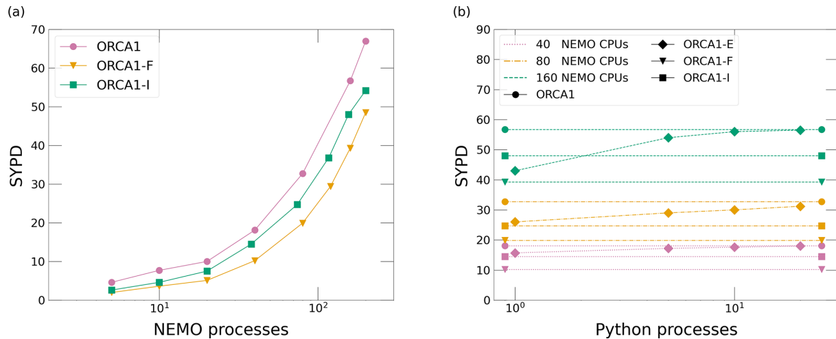
Figure 9. (a) Simulation speed in Simulated Year Per Day as a function of the number of MPI processes allocated to NEMO for different implementations of the Storto et al. (2025) ML model: NEMO without ML model (ORCA1), with Fortran (ORCA1-F), and Infero (ORCA1-I). (b) Simulation speed in Simulated Year Per Day for ORCA1-E as a function of the number of MPI processes allocated to the Python script for different number of processes allocated to NEMO. Results are compared for different implementations of the Storto et al. (2025) ML model: NEMO without ML model (ORCA1), with Fortran (ORCA1-F) and Infero (ORCA1-I). Lines for those cases are here for readability as their values are fixed and independent of the number of Python processes.
