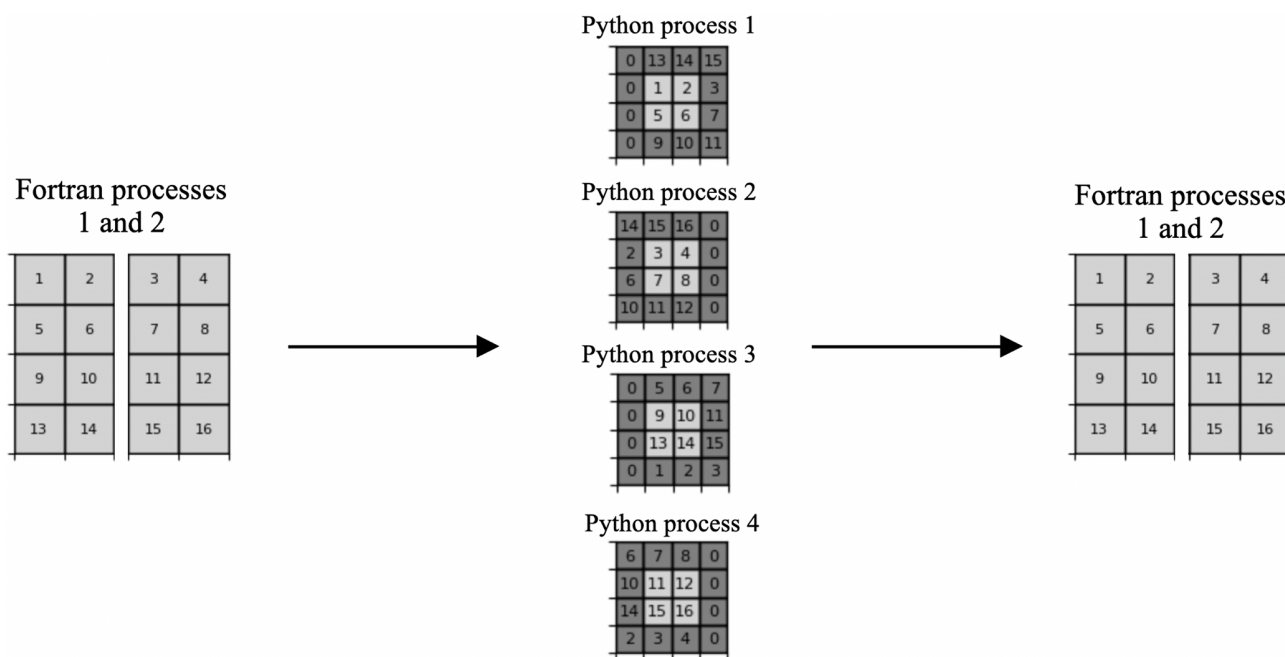
Figure 4. Halo reconstruction principle diagram. In regular coupling, each cell (in light gray) is communicated once between processes, as in Fig. 3. Eophys can configure OASIS3-MCT parallel features to communicate grid cells several times. The local grid from one Python process can receive a copy of cells (in dark gray) addressed to another Python process. They correspond to the neighboring cells of the local grid. Halo cells are present on the Python side to let the Python scripts work with array-like objects without the need for internal communications. These are ignored when sending back the coupling information from Python to Fortran processes. The number of halos and how to fill them at the boundaries are user parameters.
